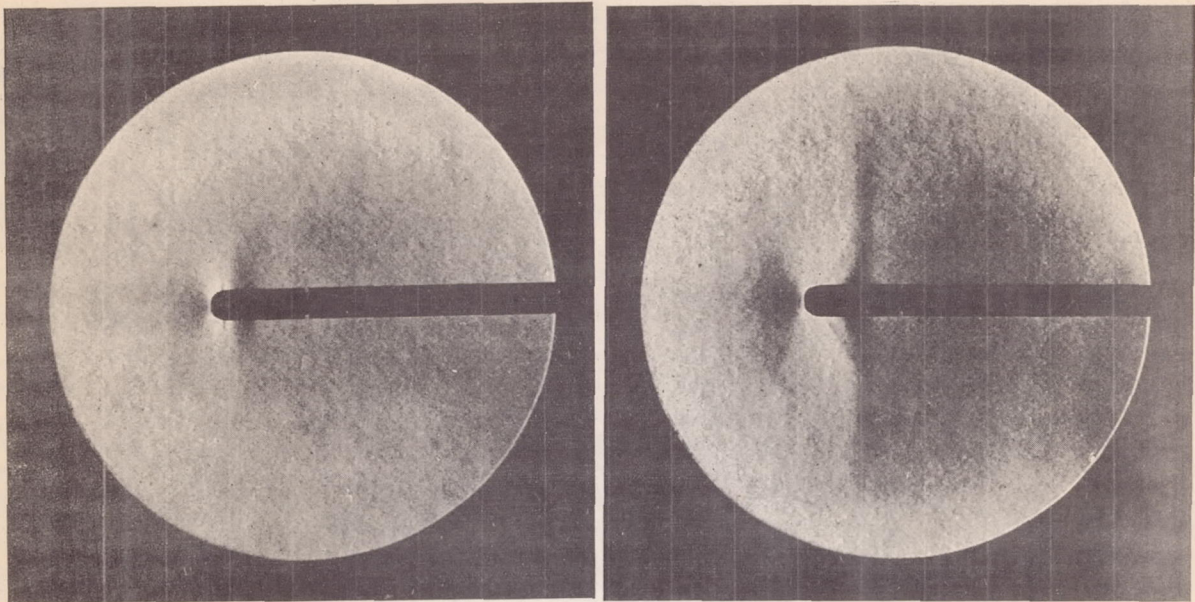
Figure 3.- Schlieren record at w/a = 0.85 .
