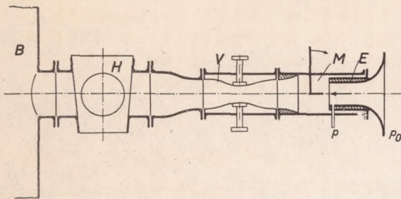
Fig. 1.- Prandtl type high-speed wind tunnel.
