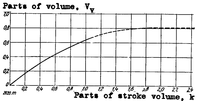
Figure 12.- Scavenging results for loop scavenging (adopted and extended according to reference 2)
