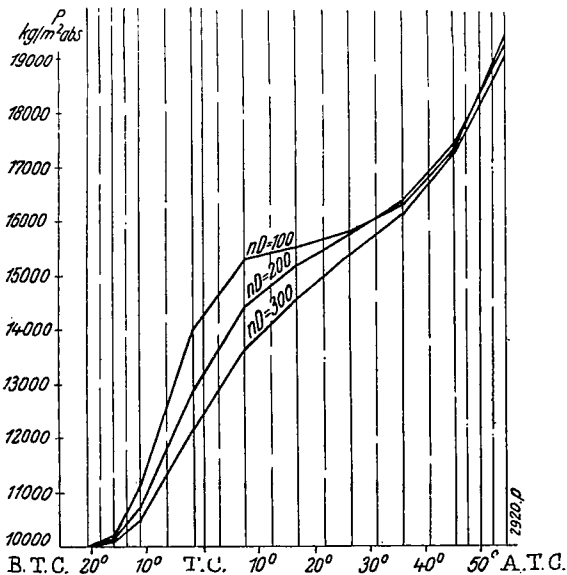
Figure 15.- Pressure variation during scavenging at P_s = 20,000 \text{ kg/m}^2 and different nD .
