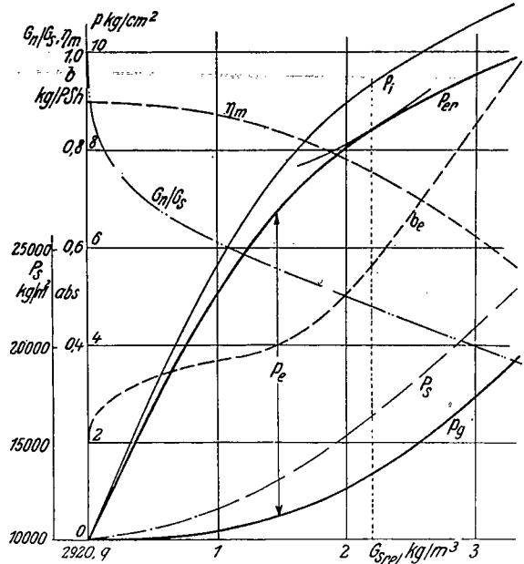
Figure 16.- Indicated and mean effective pressure, mechanical efficiency, fuel consumption against amount of scavenging air in mixture scavenging engines.
