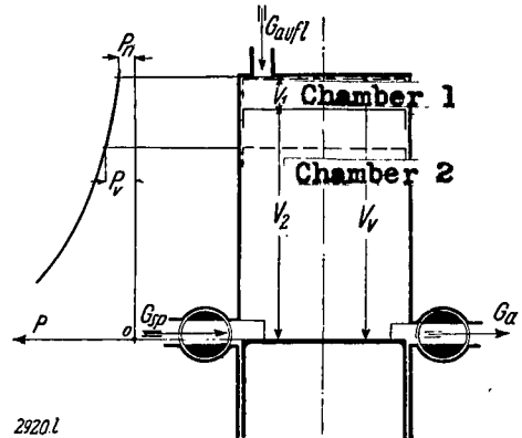
Figure 11.- Two-stroke cycle engine with scavenging and boosting separated in time and space.
