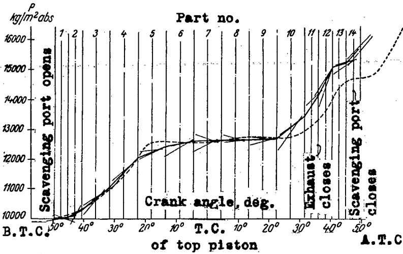
Figure 5.- Pressure variation during scavenging cycle in the Junkers engine. Solid line; computed; dotted line; indicated, as obtained by replotting fig. 4.
