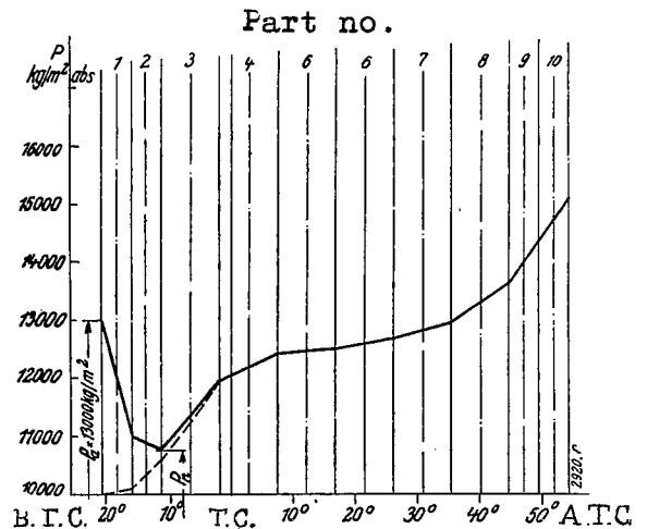
Figure 17.- Pressure variation during scavenging, for P_a = 13,000 \text{ kg./m}^2 .
