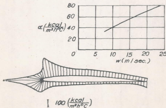
Figure 17.- Heat transfer at wing.
