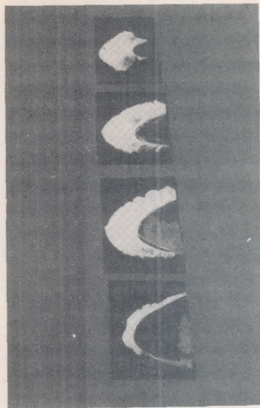
Figure 15.- Icing of profile noses of various chords.
