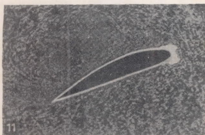
Figure 11.- Profile with clear ice in water tunnel.
