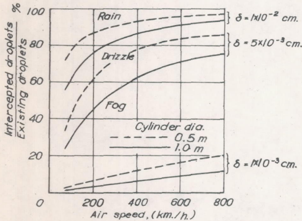
Figure 14.- Droplets intercepted by cylinder.
