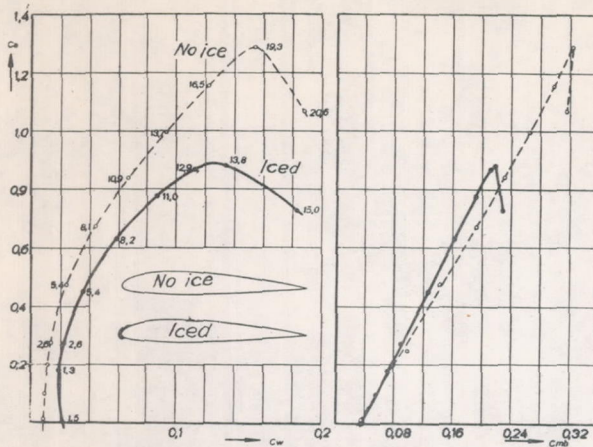
Figure 5.- Polars of a rectangular wing.
