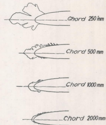
Figure 16.- Icing of NACA profile 2412 for various chords.
