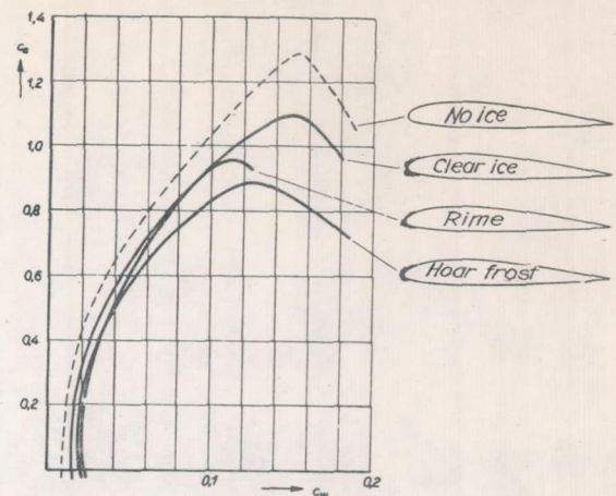
Figure 13.- Polars for three forms of icing.
