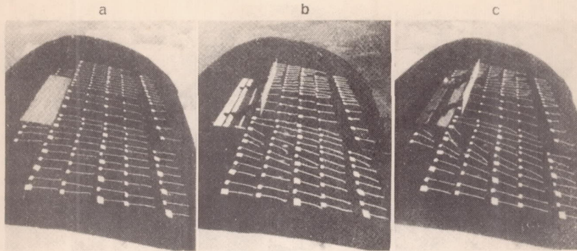
a, Flaps retracted b, " extended, version II c, " " , " III
