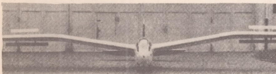
Figure 9.- Brake flaps fitted on Reiher.
