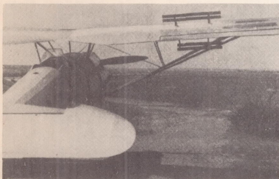
Figure 12.- Air brakes on Stösser extended.
