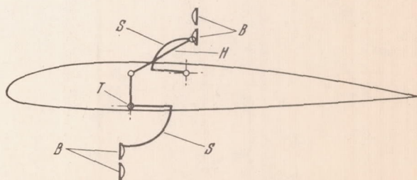
Figure 10.- Dive control brake drive on power glider FW 56 (Stösser)
