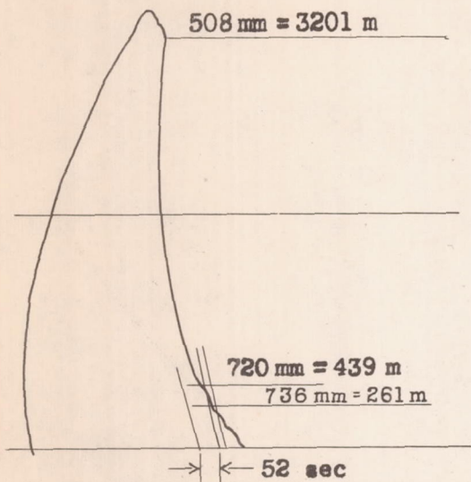
Figure 4.- Dive barogram with extended air brakes.
