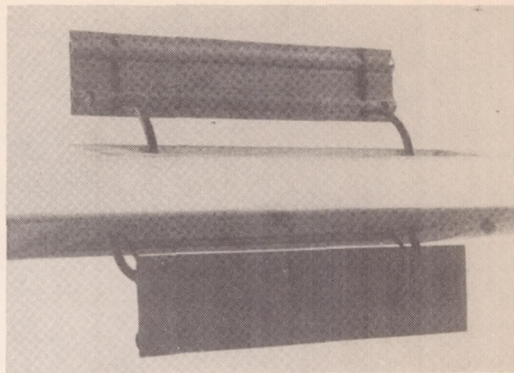
Figure 3.- DFS air brake fitted on glider, seen from trailing edge.
