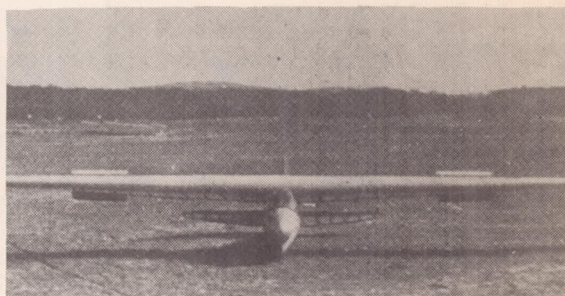
Figure 7.- Brake flaps fitted on Rhönadler.
