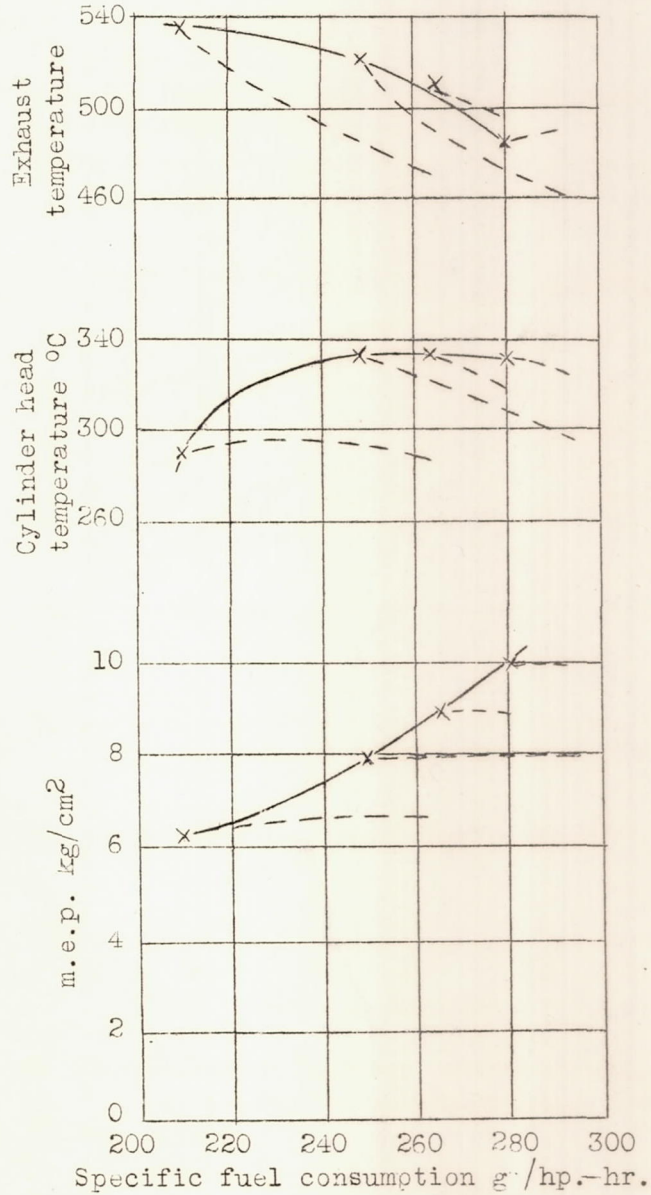
Figure 13.- Airplane engine. Relation between fuel consumption, mean effective pressure, and temperature for different degrees of supercharge.
