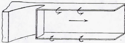
Figure 3.- Partially open jet.
