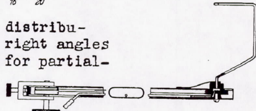
Figure 6.- Device for rotating the pressure survey apparatus about the vertical axis.
