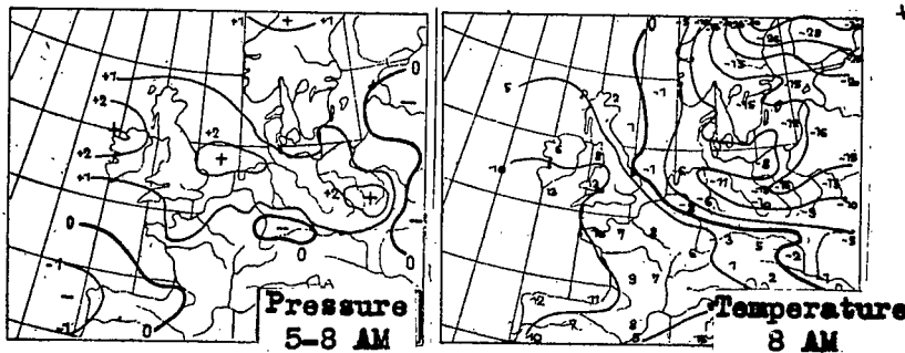
Figures 8b, c.- Temperature-pressure change for Fig. 8a.
