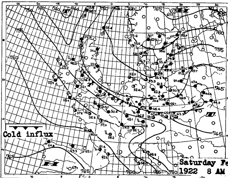
Figure 8a.- Weather conditions with ice formation due to super-cooled rain characterized by sharp cold air influx.
