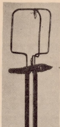
Fig. 4 Anemometric wire mounted on base.
