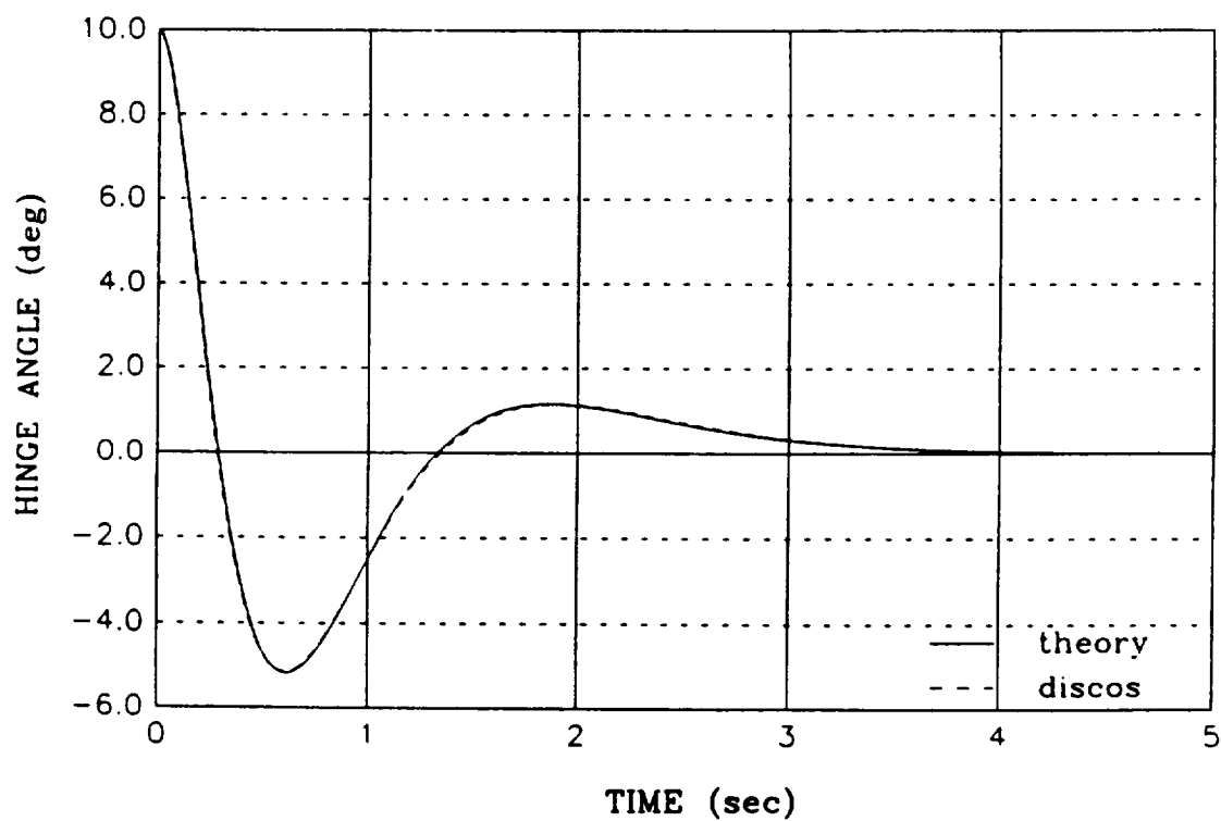
Fig. 5 Hinge Angle Response of Stabilized Inverted Pendulum
