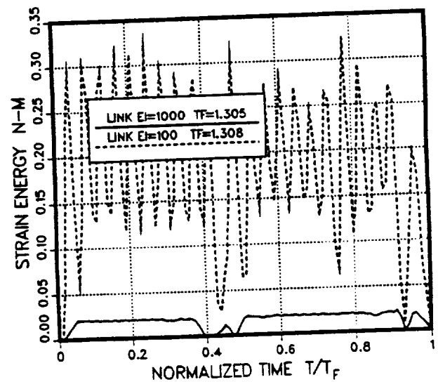
Figure 4: Strain energy histories
