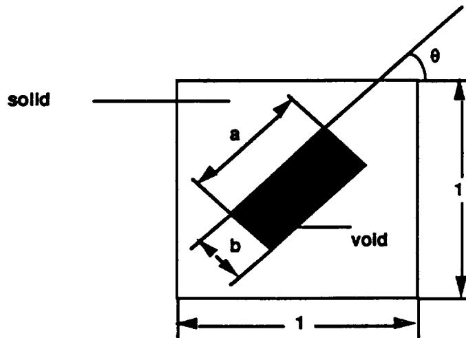
Figure 1. Definition of a microscale hole, i.e., a finite element for homogenization method.
