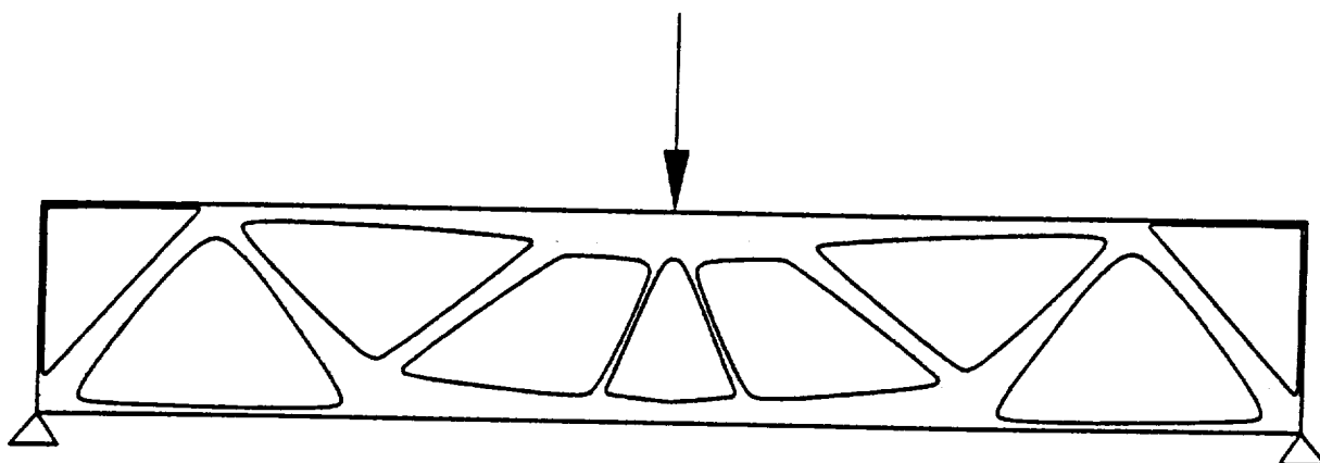
Fig. 5. Example of final geometry slightly modified by the designer. The upper right corner has been added again.
