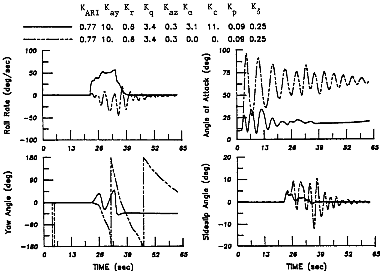
Figure 4 Design of a Control System to Prevent Pitch Departure of an F-16 Configuration in a Pull-up and Roll Maneuver at M = 0.5 and h = 30,000 ft.
