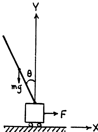
Fig.1C An Inverted Pendulum System
