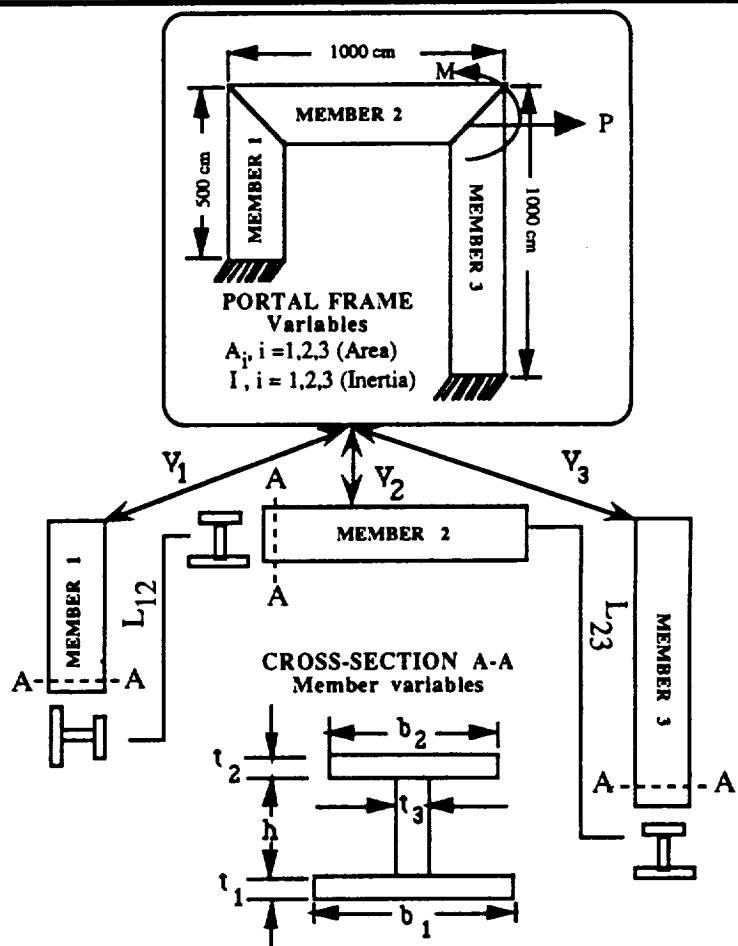
FIG. 1b - PORTAL FRAME AS A HIERARCHICAL MODEL
