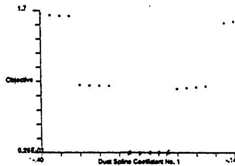
Figure 10. Objective as a function of duct geometry for the C^0 scheme with grid refinement
