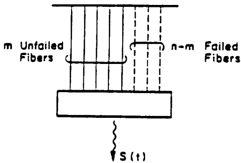
Figure 1. Daniels System with n Fibers in Damage State m \leq n
