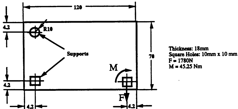
Figure 9. Boundary specifications and initial design domain for Example 3.
