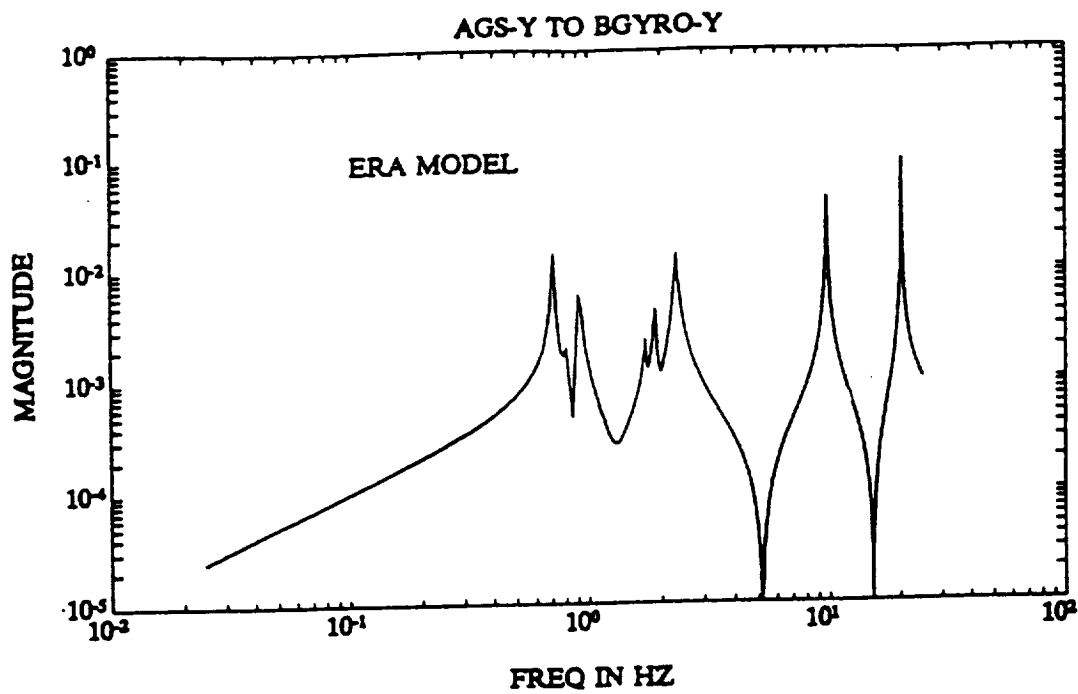
Figure 5.1. One of the two major feedback loops used to design vibration control laws for the ACES Structure at NASA Marshall Space Flight Center.
