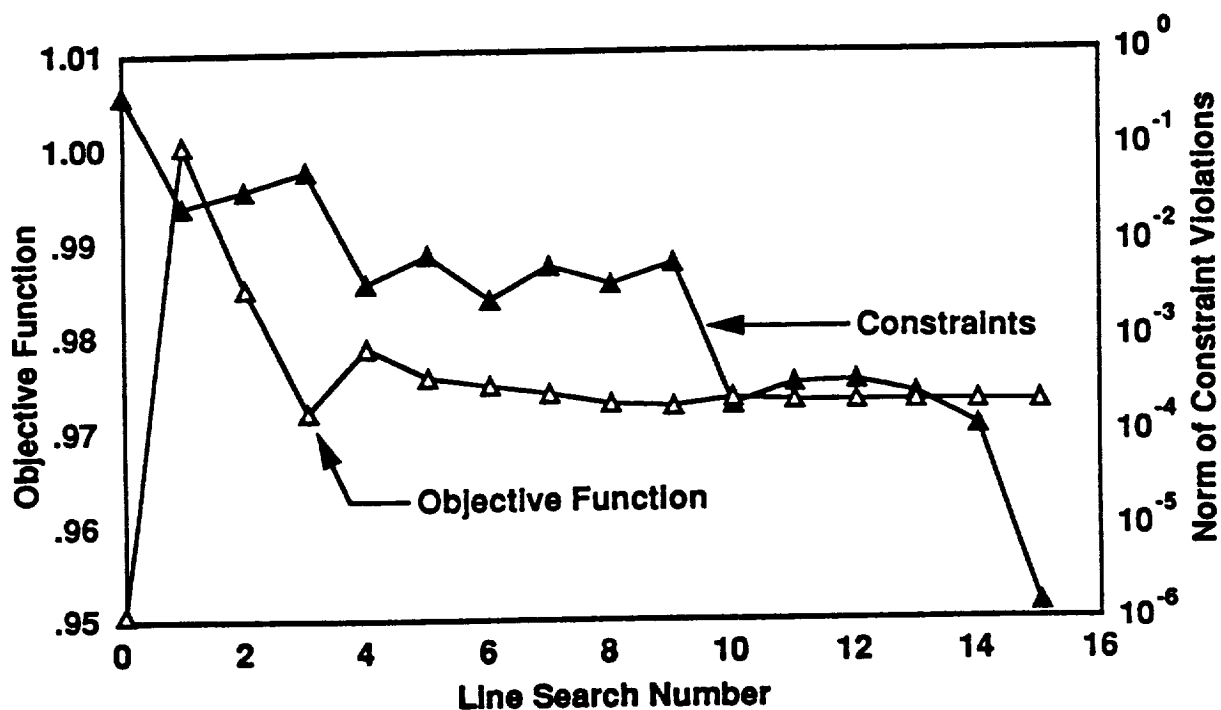
Fig. 5 The iteration history of the objective function and the constraint violations for a joined-wing design problem.
