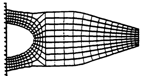
FIG.2. Optimal design of a beam. A: Optimal topology with outline showing reference domain. B and C: Initial and final design using the boundary variations method. Two blocks are used for the elliptic mesh generator. Only the boundaries of block 1 can move. The maximum stress is reduced by 55.7% and the compliance by 7.3%. Block divisions are shown as hatched, bold lines: design boundaries as bold solid lines.
