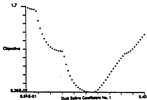
Figure 6. Objective as a function of duct geometry for the C^0 scheme
