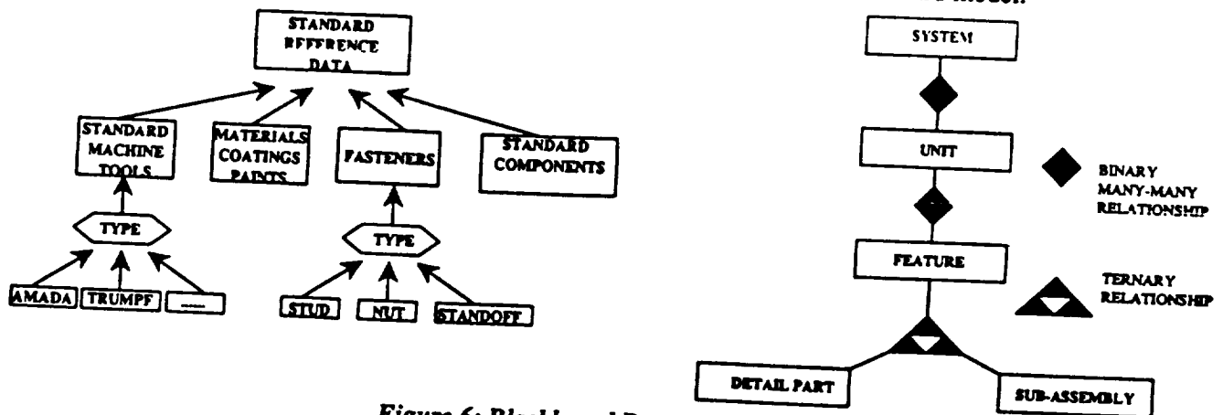
Figure 6: Blackboard Data Schema
