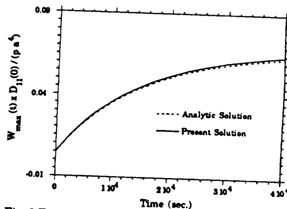
Fig. 2 Time dependent max. bending deflection of a simply supported composite plate.
