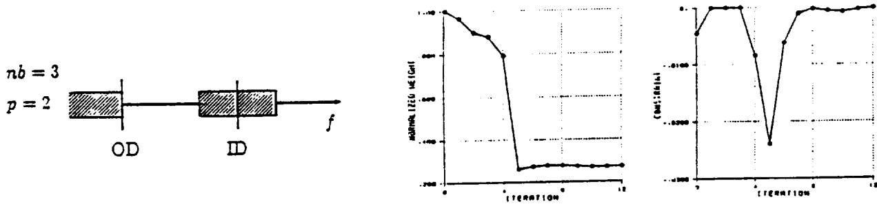
Figure 5: a) Multiple constraint for lowest eigenfrequency b) Weight history c) Constraint history
