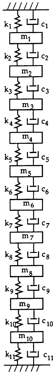
Figure 1. Ten Degree of Freedom Mass-Spring-Damper System
