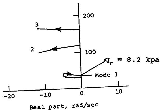
Fig. 7 Dynamic pressure root locus.
