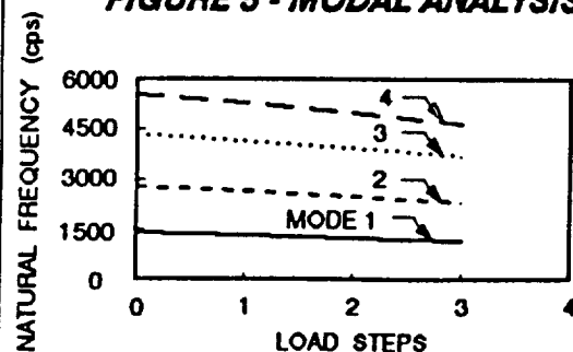
FIGURE 5 - MODAL ANALYSIS
