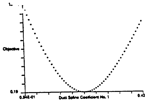
Figure 8. Objective as a function of duct geometry for the C^0 scheme
