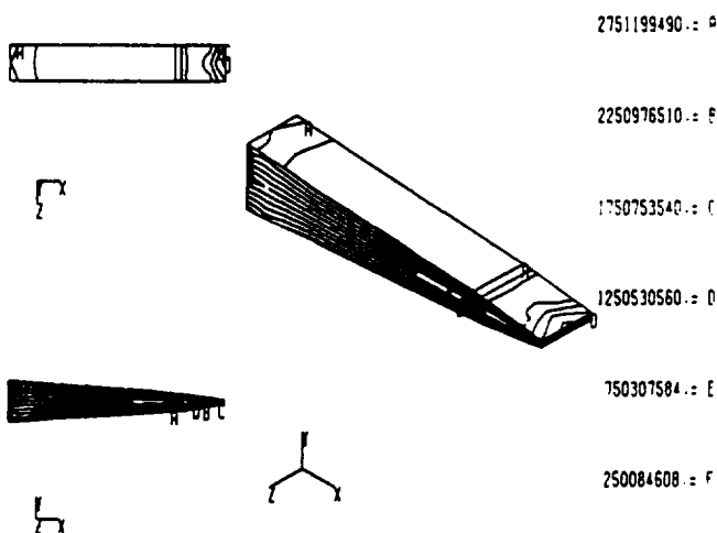
Figure 8: Constrained cantilever beam optimal design stress contours.
