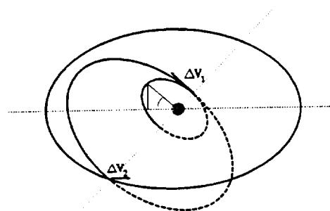
Figure 4 Hohmann Transfer with Plane Change
