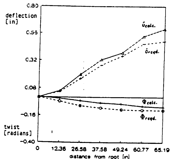
Figure 2. Test Problem 2 Deflection and Twist
