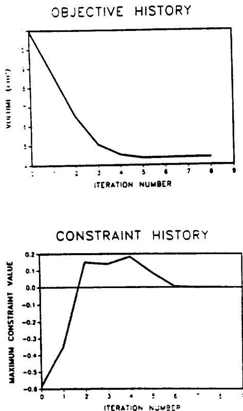
Figure 9: Constrained cantilever beam optimization history.
