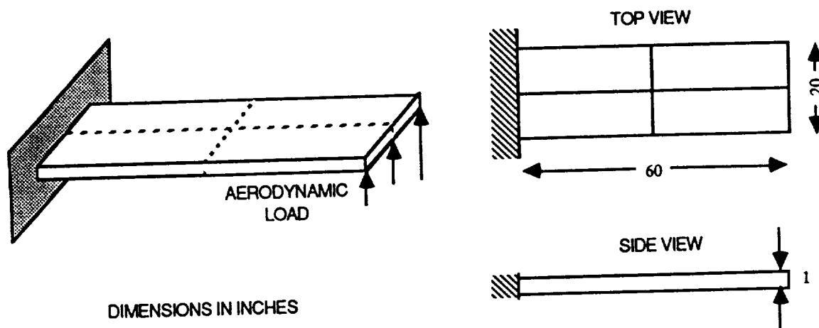
Figure 4. The Simple Wing Structure (SWS) was used to test the branch and bound method because it has only eight membrane elements modeling the skins, and requires only sixteen design variables.
