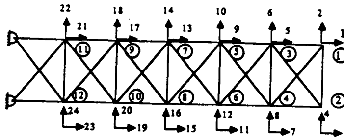
(a) Six-Bay Truss
