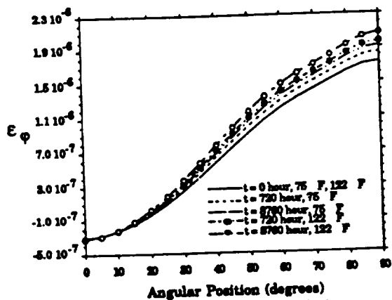
Fig. 9 Circumferential creep around a hole in GY70/339 (0/90)_s laminate
