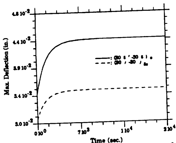
Fig. 5 Time dependent max. bending deflections of simply supported (30/-30)_{90} and (30_g/-30_g)_s laminate.
