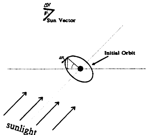
Figure 3 Vehicle-Sun Beta Angle
