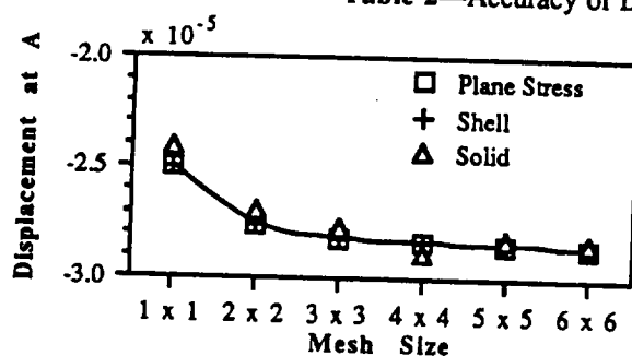
Figure 6—Accuracy of Displacement for Plate.
