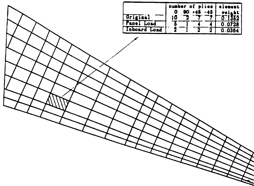
Figure 3 - User-selected Optimization : Outside Skin Elements Only
