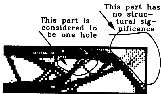
Fig. 2. Result of topology optimization.
