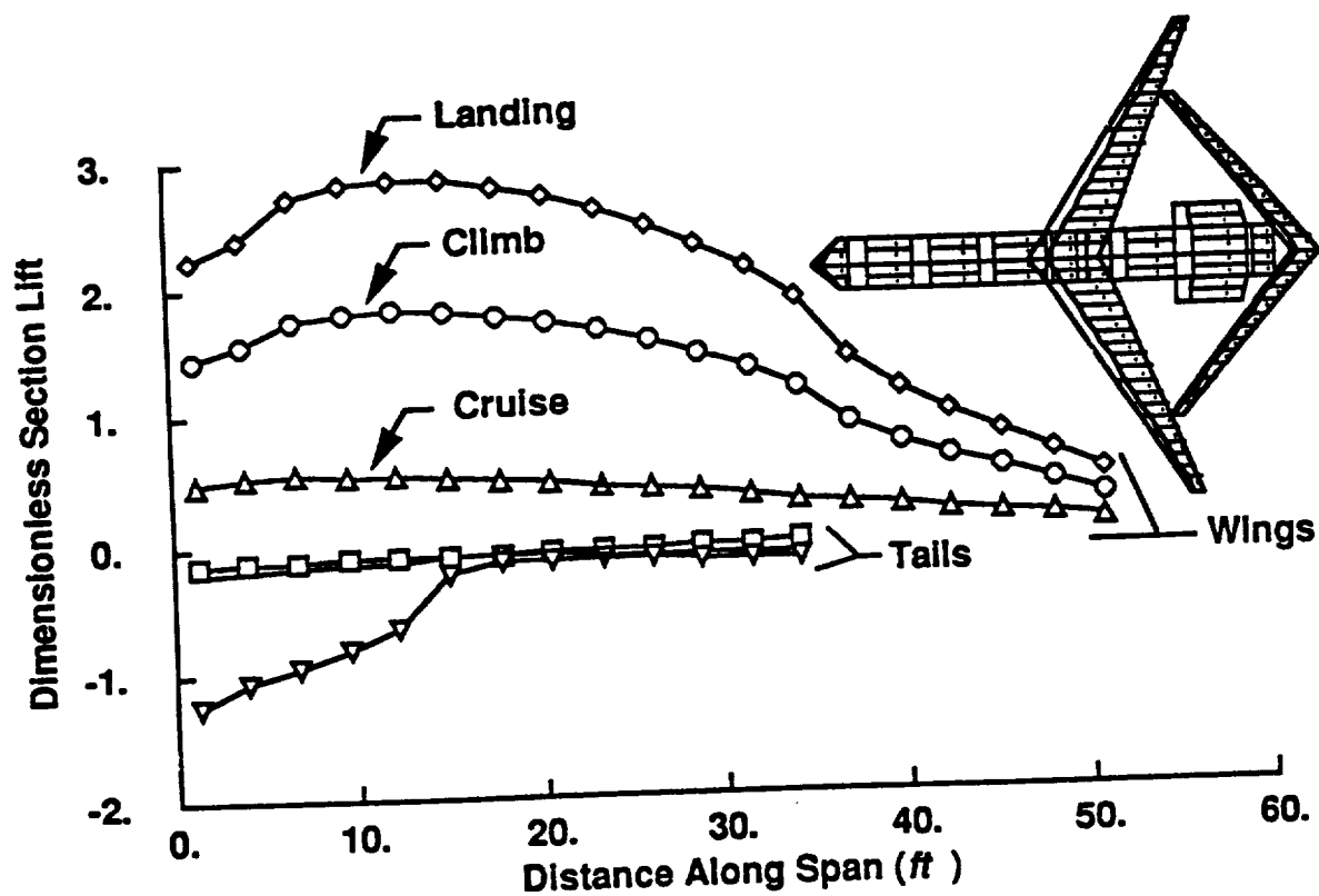
Fig. 1 Wing and tail lift distributions for a typical joined wing that is trimmed for climb, cruise, and landing approach.
