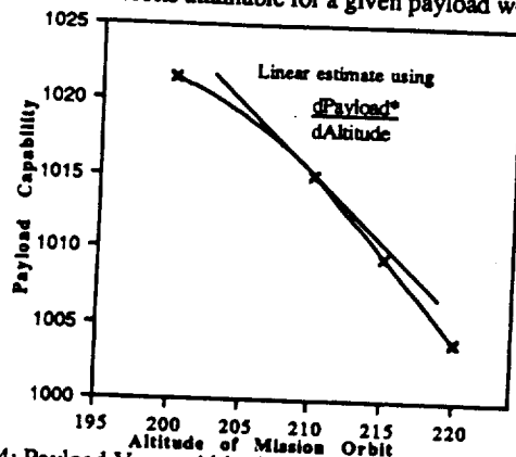
Figure 4: Payload Versus Altitude for generic Two Stage Booster
