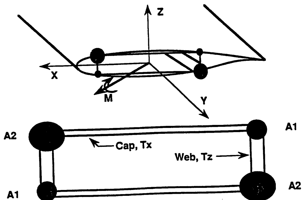
Fig. 2 Structural box model with skins, stringers, and the resultant bending moment.
