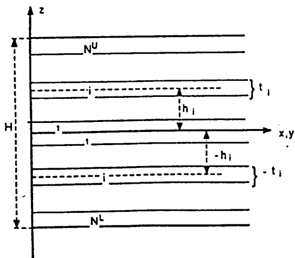
Figure 1 Coordinate system and geometrical parameters of the laminated plate
