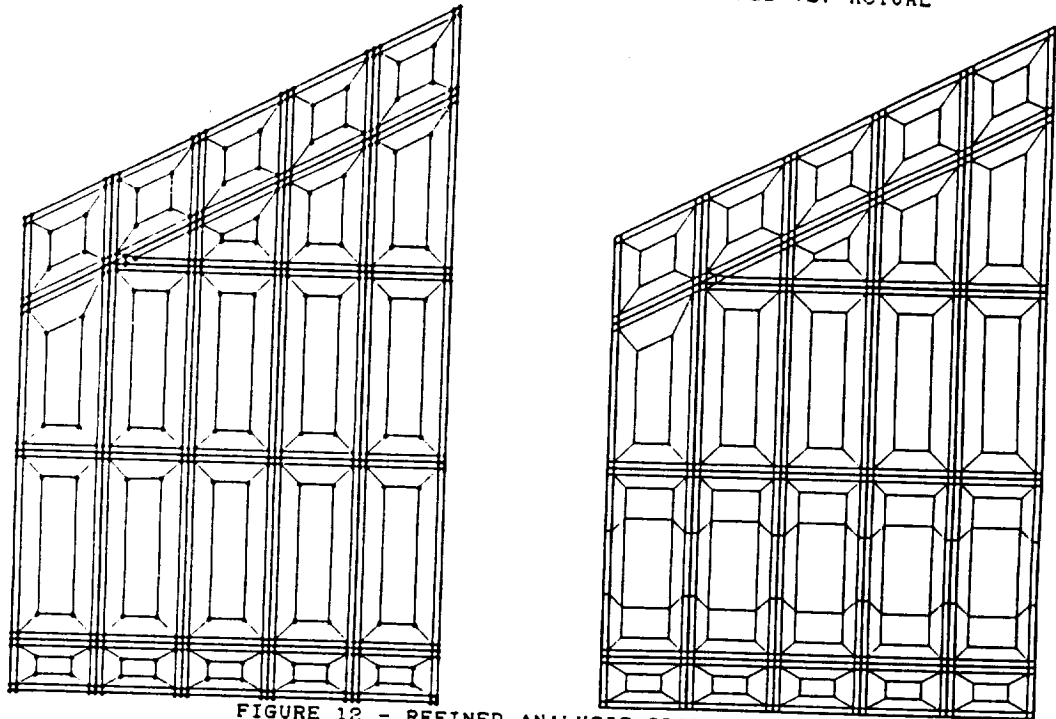
FIGURE 12 - REFINED ANALYSIS GRIDS OF HWTS
