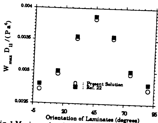
Fig. 1 Maximum bending deflection of square clamped composite laminate.
