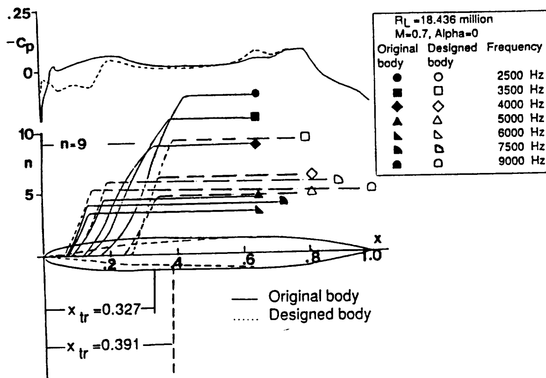
Fig. 2. Pressure distributions, predicted compressible T-S disturbance growth curves and transition locations on the original tiptank and the final design shape (optimization by hybrid transition criterion)
