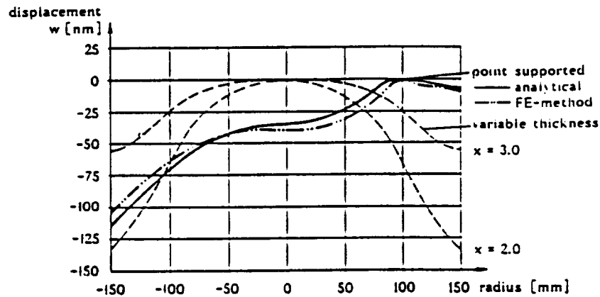
Fig. 4: Comparison of the displacements of a circular plate
