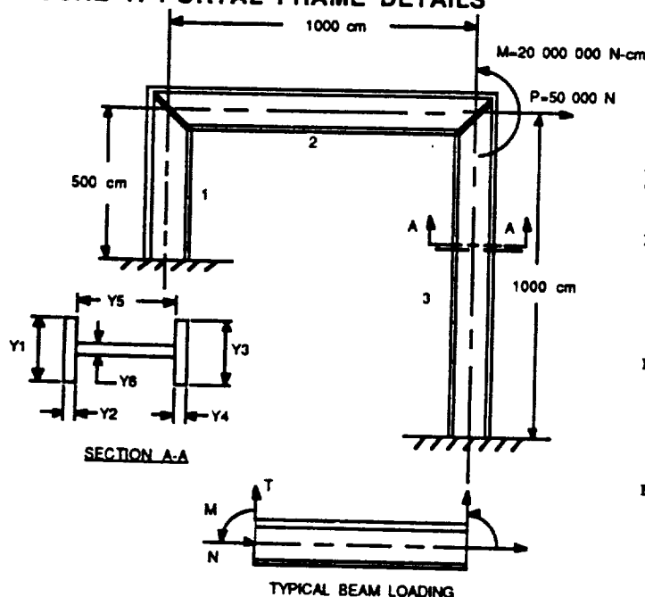
FIGURE 1: PORTAL FRAME DETAILS
