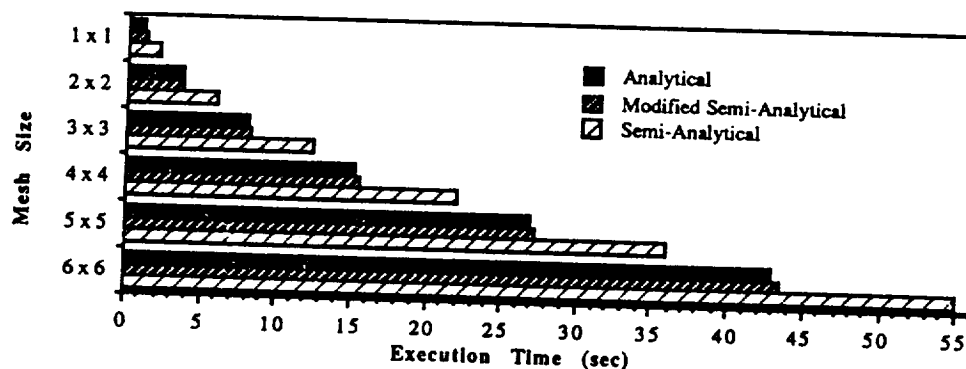
Figure 8—Execution Time for Plate Sensitivity Analysis
