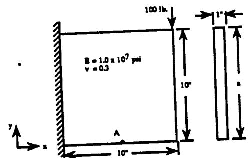
Figure 5—Plate.
