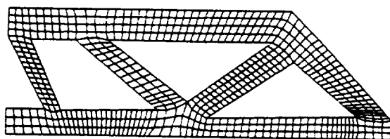
Fig. 3. Initial finite element mesh of optimized topology.
