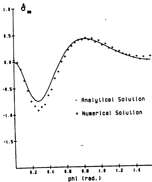
Figure 4. Angular variation of \sigma_{\theta\theta}^{\Delta} around the quarter ellipse.
