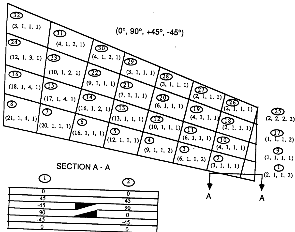
Figure 2. The Intermediate Complexity Wing was designed using ASTROS, but interleaves were required in several locations, including Section A-A.
