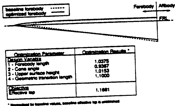
Figure 11. Case 2 results - addition of 2-D Navier-Stokes contributing analysis to case 1
