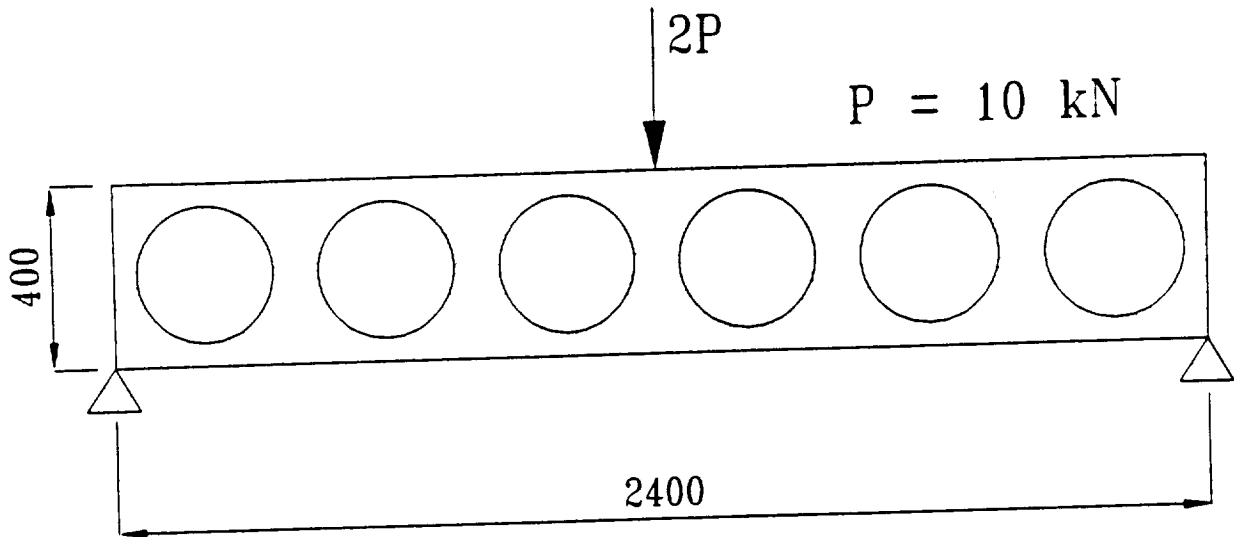
Fig. 1. Initial geometry with loads and boundary conditions.
