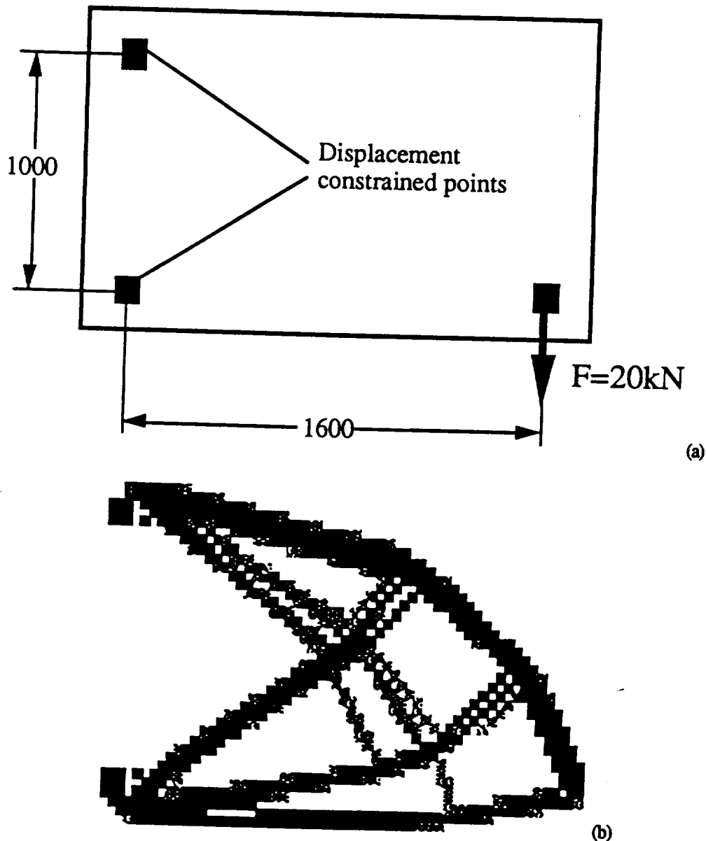
Figure 6. (a) Design specifications and (b) Optimum material distribution for Example 2.
