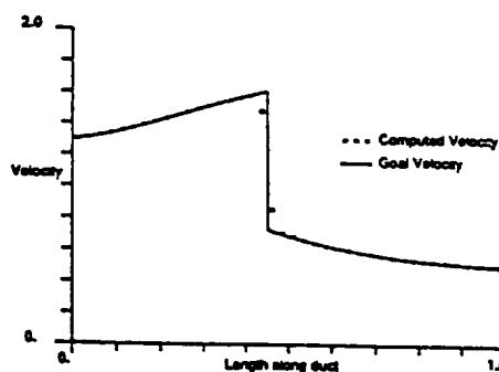
Figure 4b: Velocity profile, optimal duct with 10 design variables, no design constraints, using C^1 scheme
