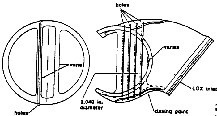
Figure 1. LOX Inlet Tee
