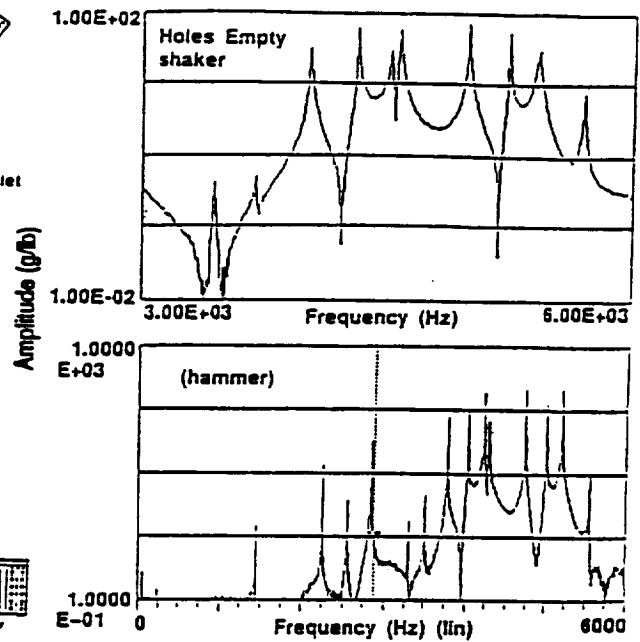
Figure 4. Vane Frequency Response Function
