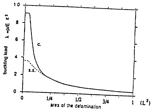
Figure 5. Variations of the buckling loads as functions of the area of a (square) delamination, for two boundary conditions
