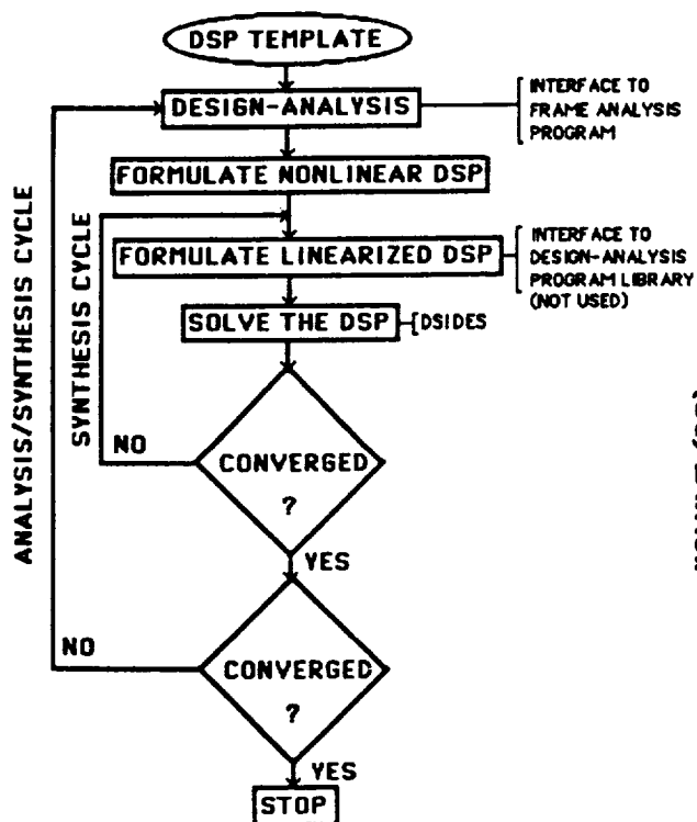
FIGURE 3 - SOLUTION SCHEME
