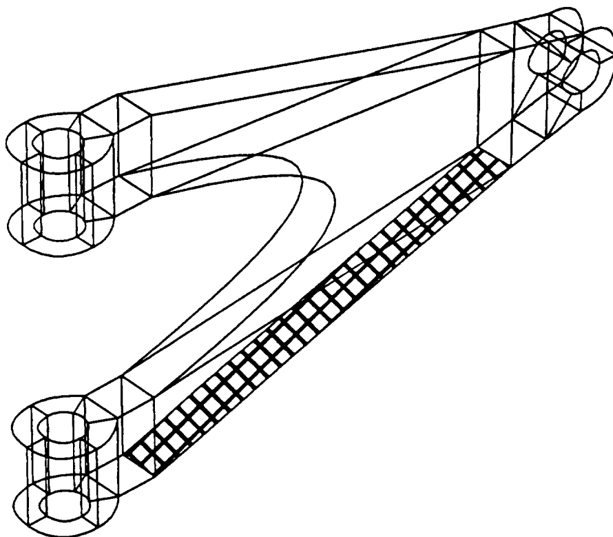
Fig. 4 Geometric Model for Torque Arm
