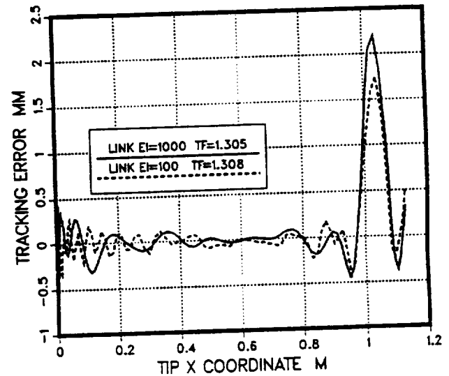
Figure 3: Straight-line tracking error
