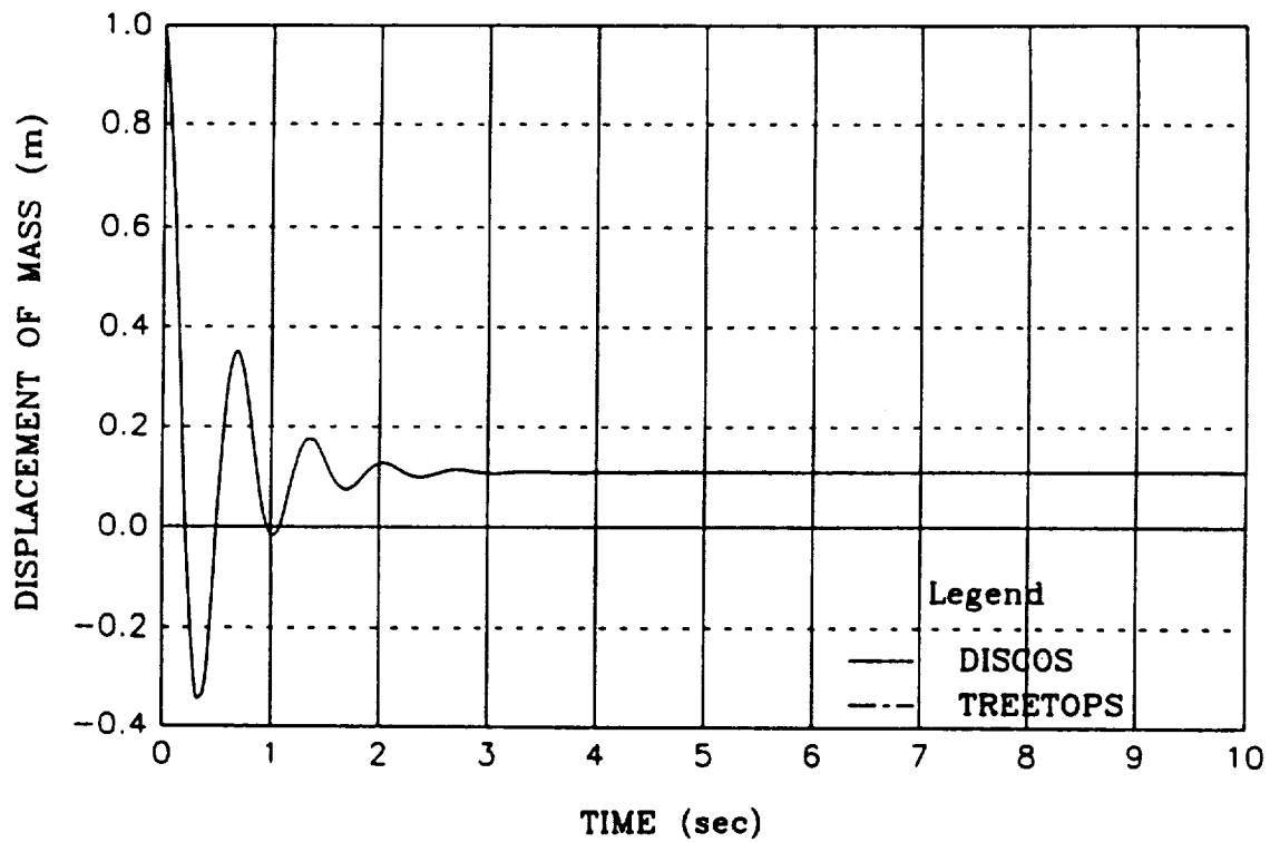
Fig. 2 Time History Response of Spring-Mass-Damper
