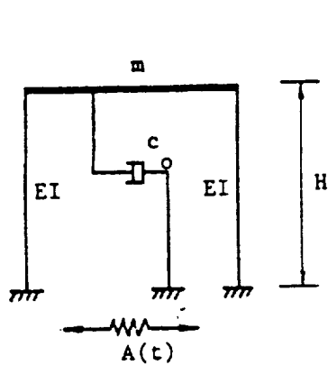
Fig. 1. Structural model
