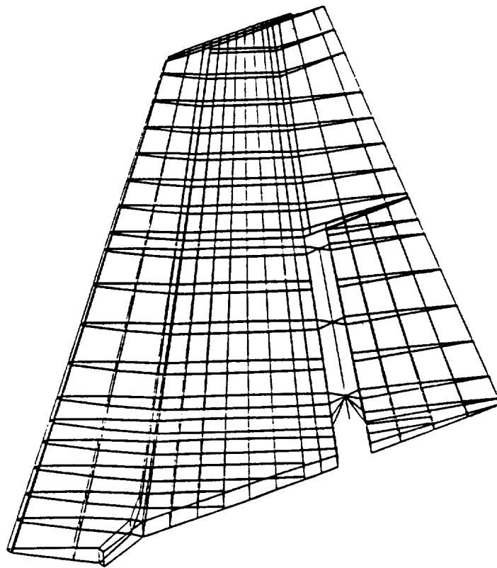
Figure 1 - Structural Model of F-15E Vertical Tail
