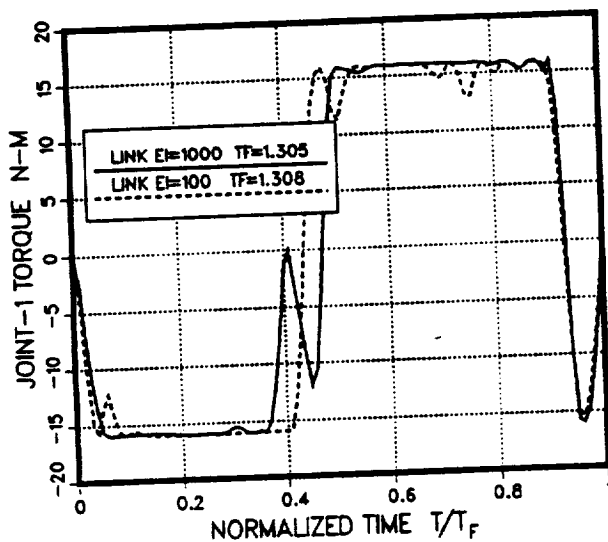
Figure 2: \tau_1 joint torque histories
