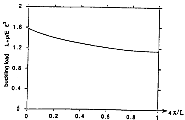
Figure 6 Variations of the buckling load as functions of the position of the delamination. The center of the delamination is at (x,0) and (y,0) , respectively
