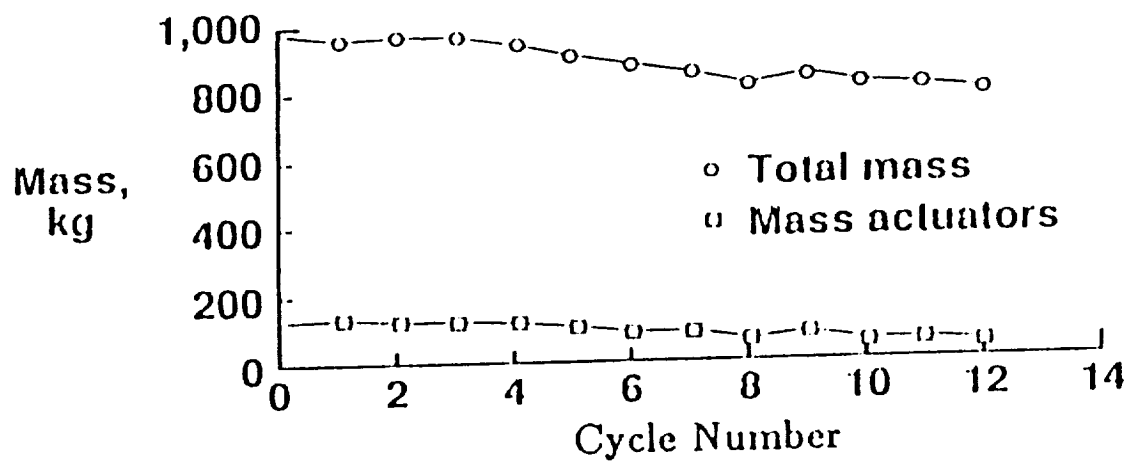
Figure 7 Mass convergence of slightly infeasible case using 15 design variables.
