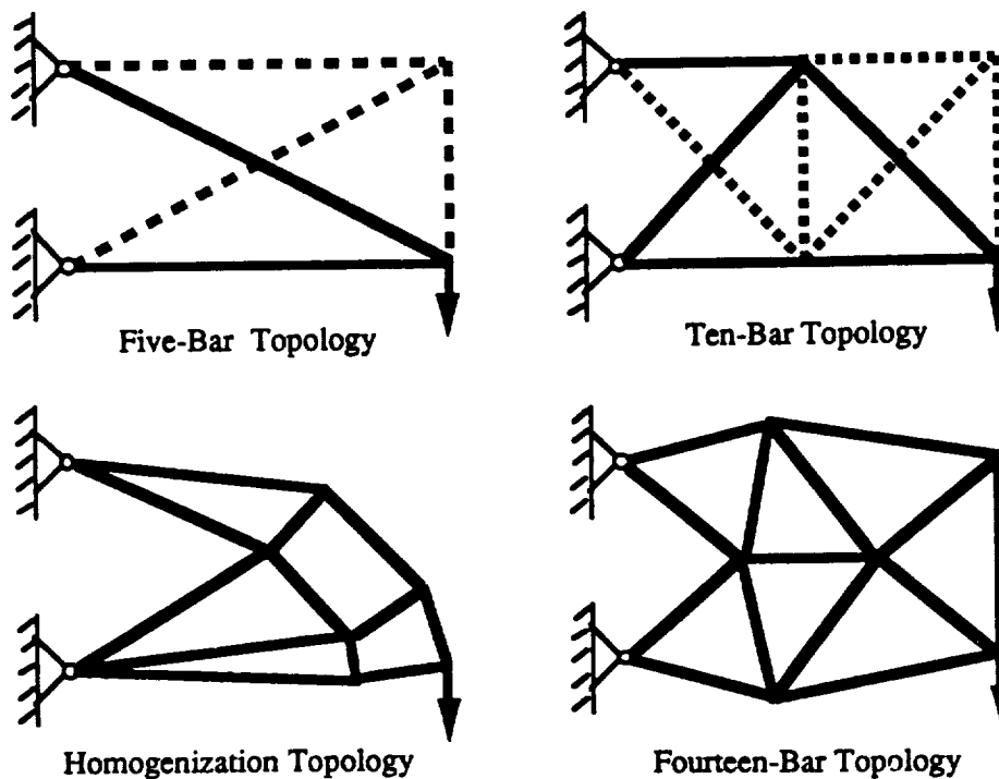
Figure 8. Alternative engineering solutions for the bracket problem.
