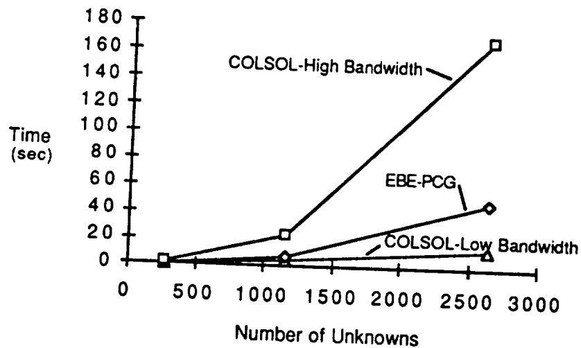
Figure 3. Solution time required for a single load case (20x20 mesh).
