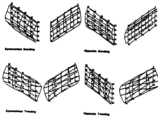
Figure 3. Vane Mode Shapes
