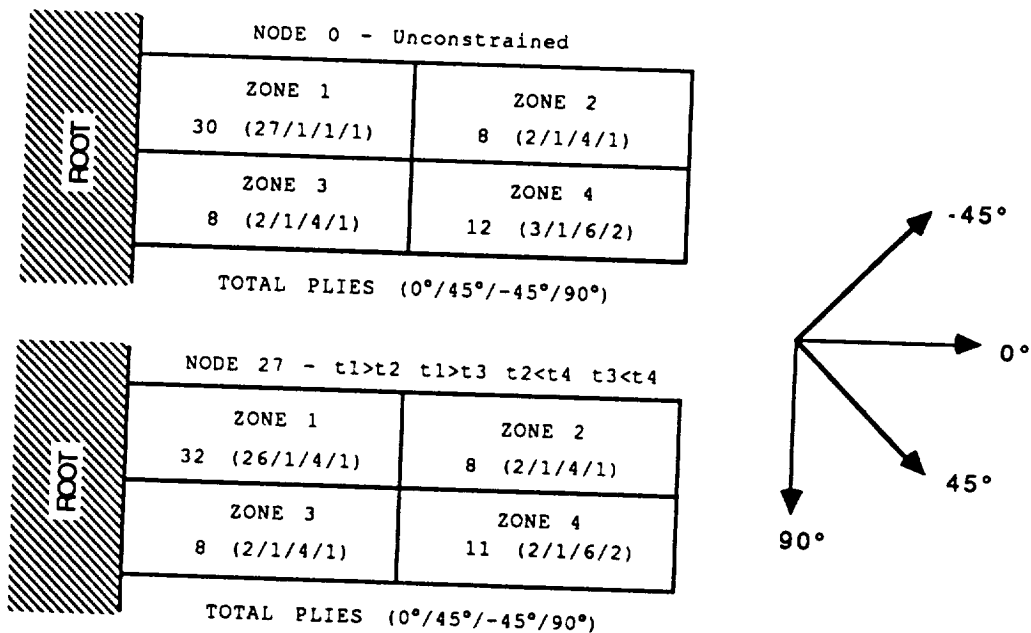
Figure 6. Ply thicknesses of Node 0 and Node 27 show how the thicknesses change to satisfy interleaving constraints.
