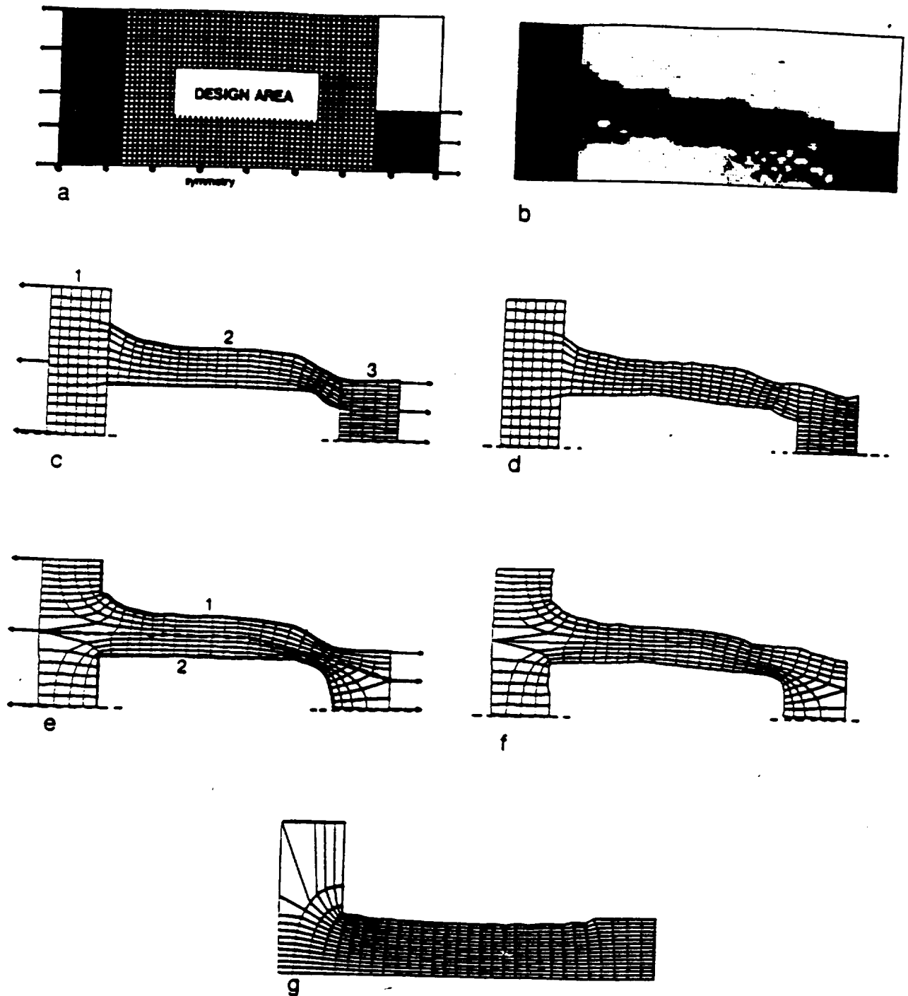
FIG.3. Optimal design of a fillet. A: The reference domain showing loads etc. and the reduced design area. B: The optimal topology. C and D: Initial design and optimal design with the boundary variations method. Mesh generated using three blocks. E and F: Initial and final optimal design using different mesh (two blocks). G: Optimal design with no hole (minimum compliance design).
