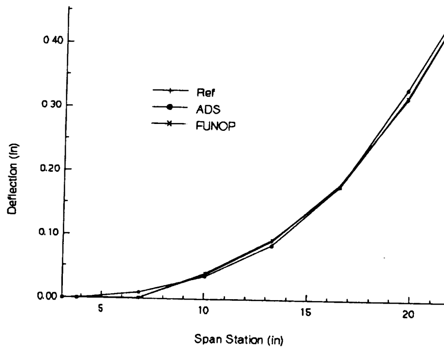
Figure 4. Deflections Along TE Due to Unit Load at Pt 28.
