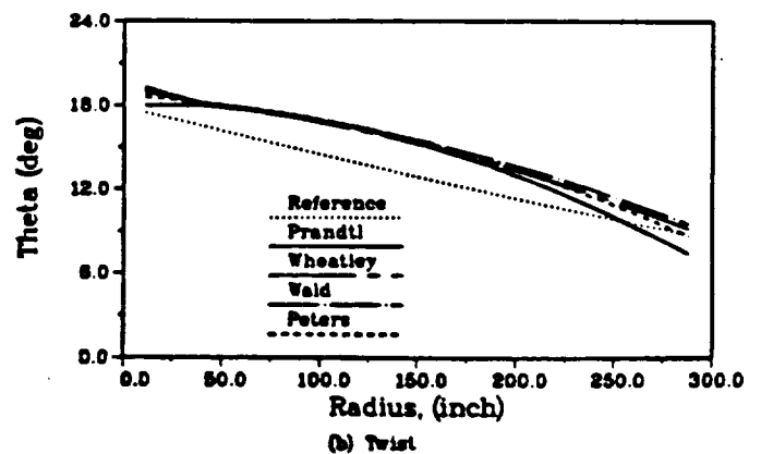
Figure 2 Comparison of Different Blade Tip Loss Formulations.
