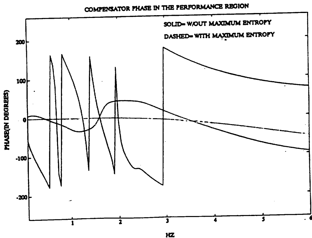
Figure 5.2. Maximum Entropy design rendered the compensators for the AGS to BGYRO loops positive real in the performance region.
