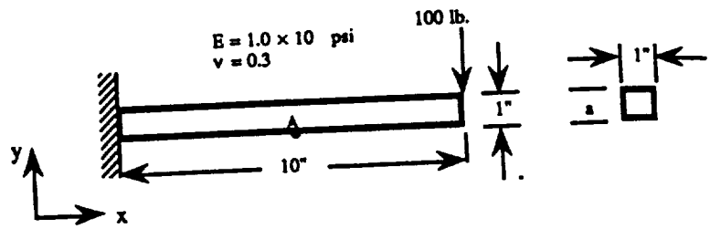
Figure 2—Cantilever Beam.
