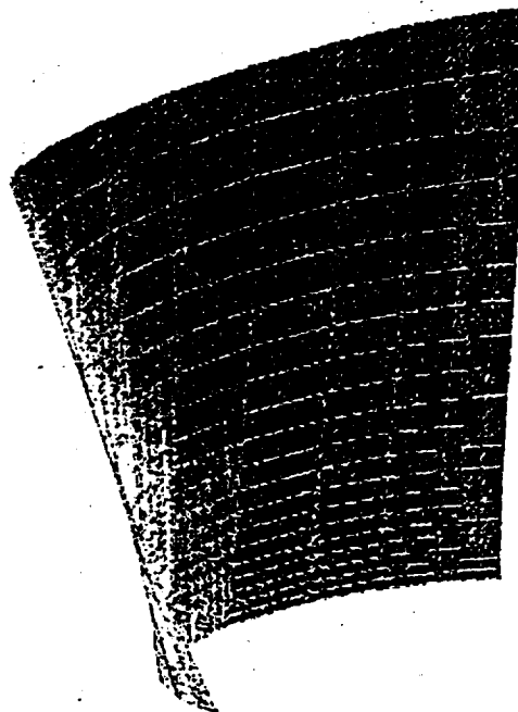
Fig.1. Power turbine blade FE model
