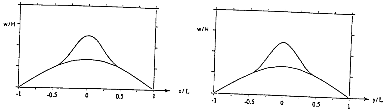
Figure 3 Cross-sections of the buckling mode of the delaminated plate.
