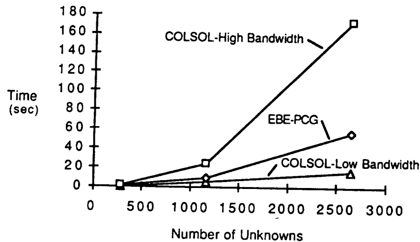
Figure 5. Solution time required for two identical load cases (20x20 mesh).
