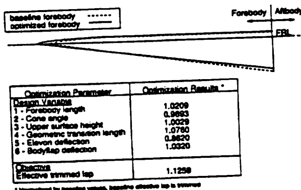
Figure 13. Case 4 results - addition of flexibility to case 3
