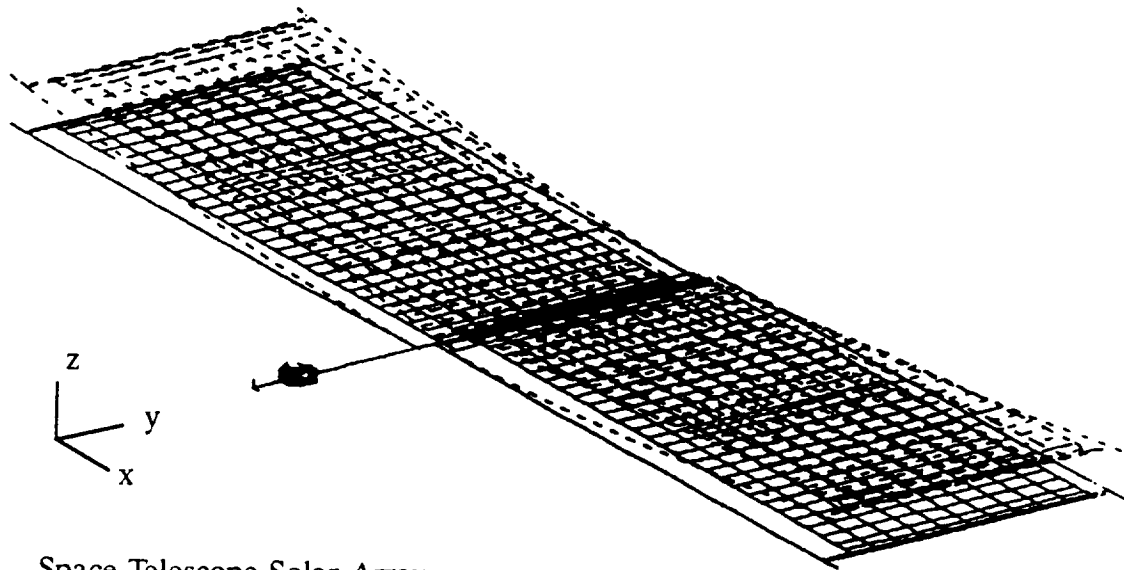
Figure 1: FEM model and some related main modes.
