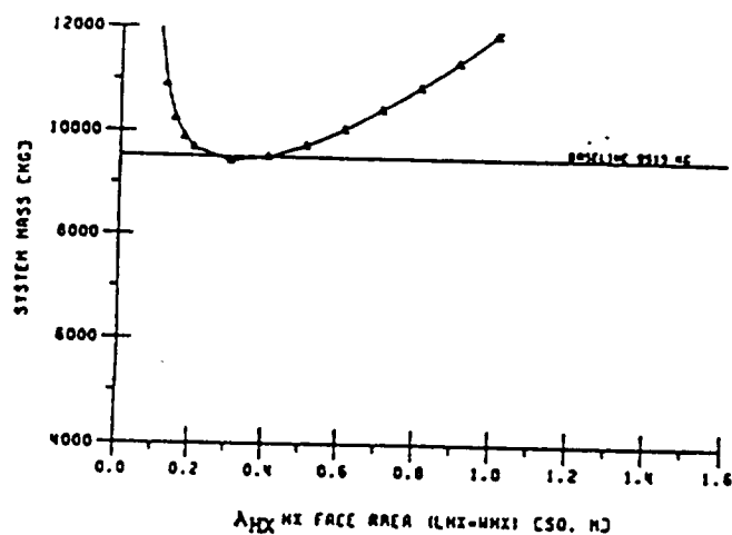
Figure 2 HX Face Area vs. System Mass (Parametric Study)
