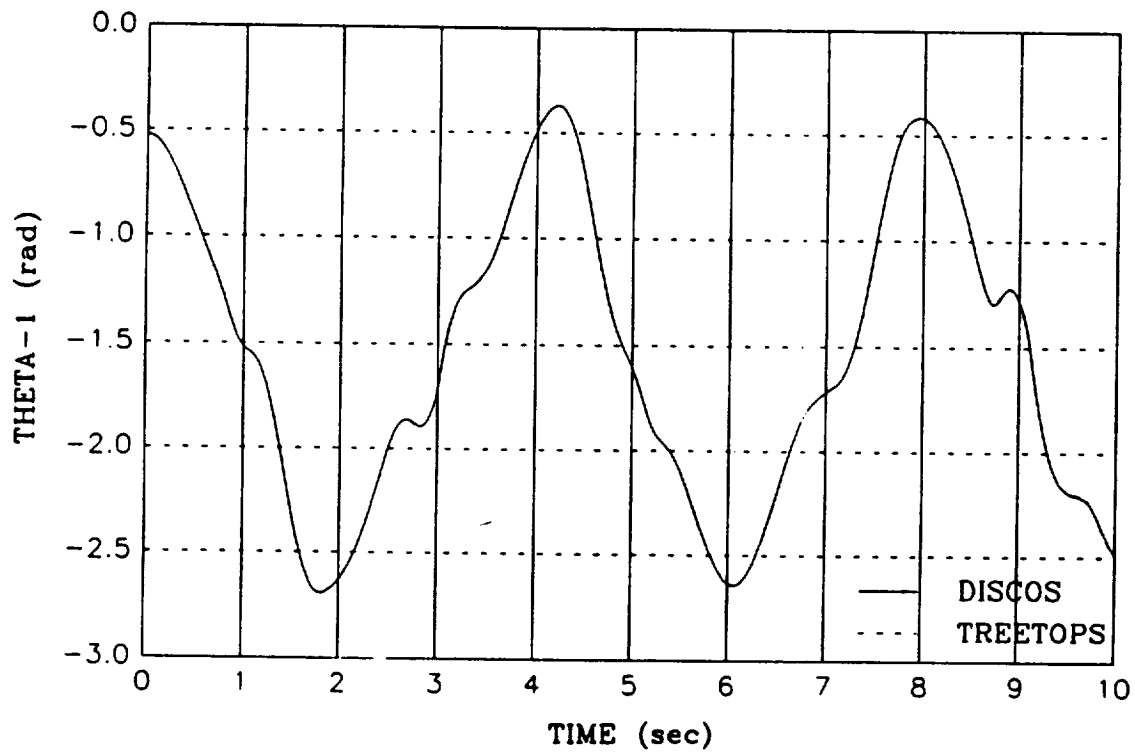
Fig. 3 Time History Response of Hinge Angle 1
