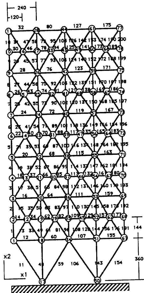
Figure 1 200-Member truss
