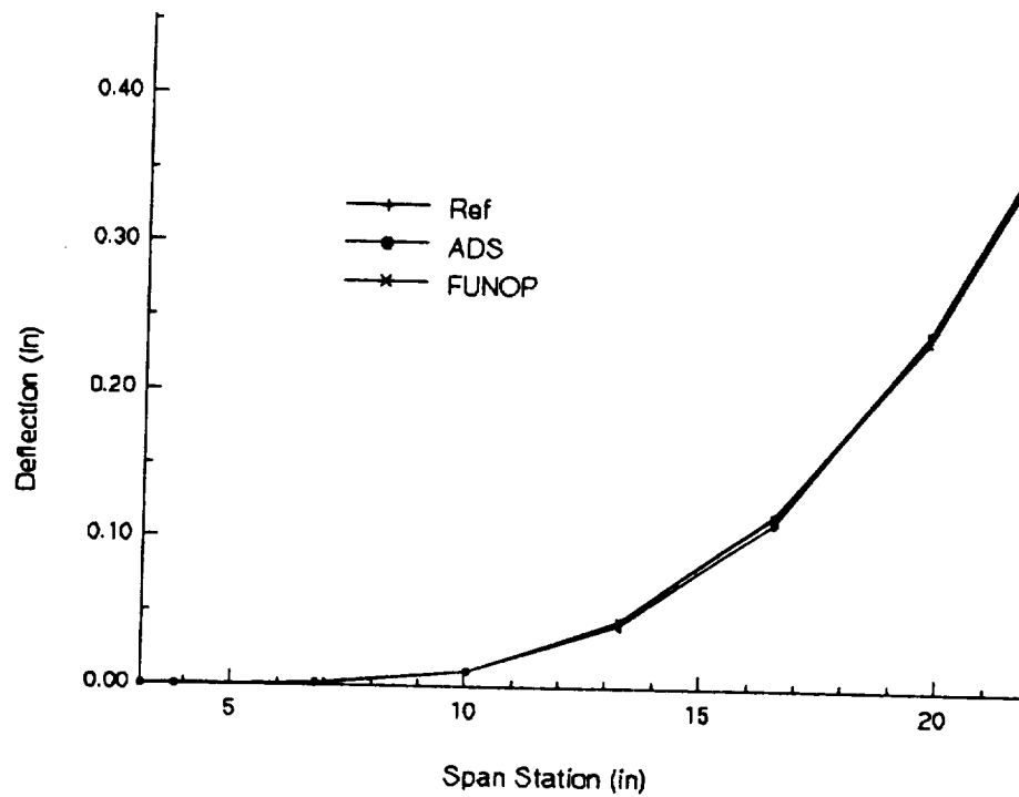
Figure 3. Deflections Along LE Due to Unit Load at Pt 28.
