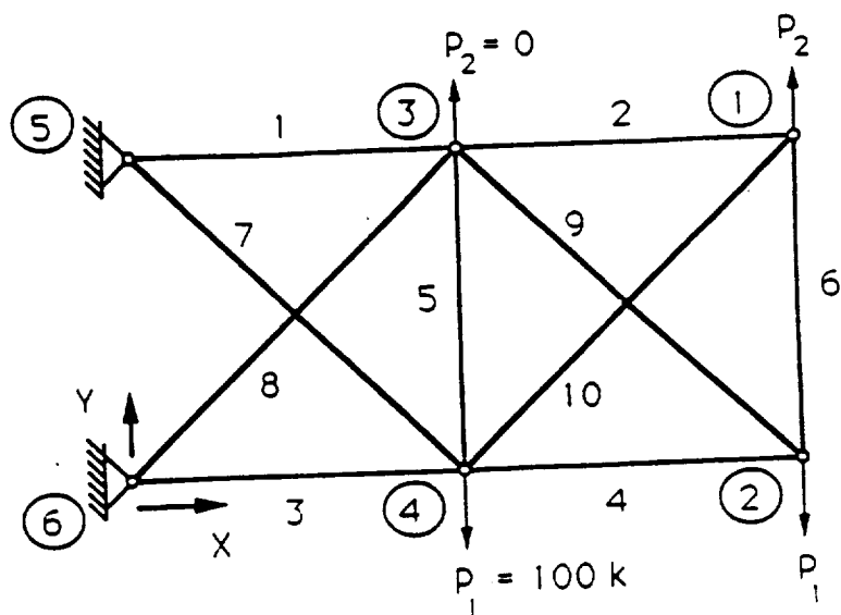
(a) Ten-Member Planar Truss
