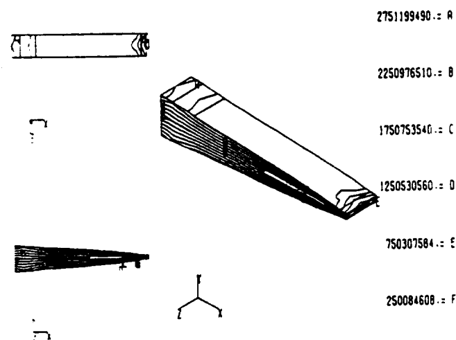
Figure 5: Cantilever beam optimal design stress contours.
