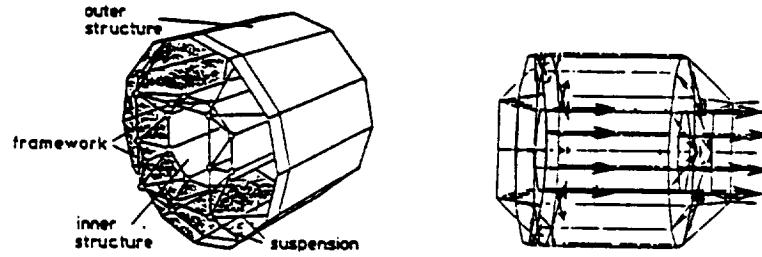
Figure 3: a) Satellite structure b) 9th mode shape (initial design)
