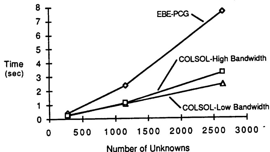
Figure 6. Additional time required for the second load case.
