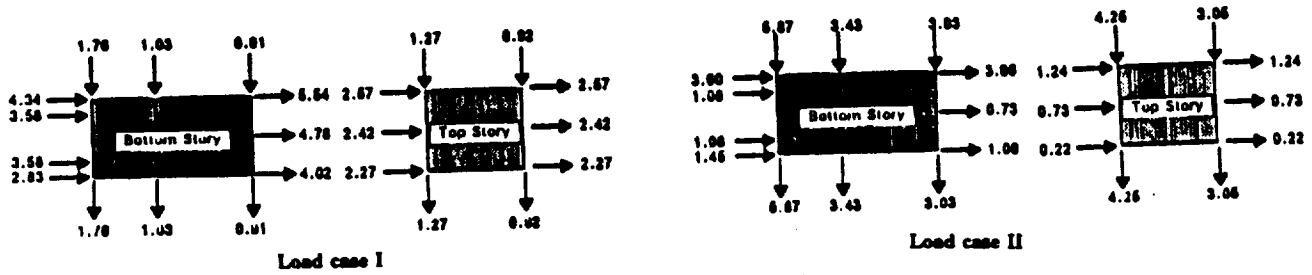
Fig. 2 Load cases for setback structure
