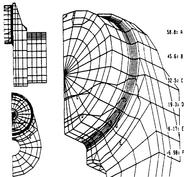
Figure 10: Automobile crankshaft original design.
