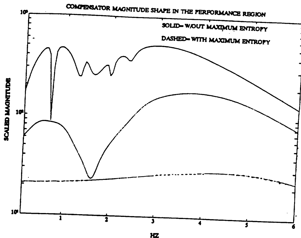
Figure 5.3. For the AGS to BGYRO loops Maximum Entropy design smoothed out the compensator magnitudes in the performance region, thus providing performance robustness and also indicating that the robust controllers were effectively reduced-order controllers.
