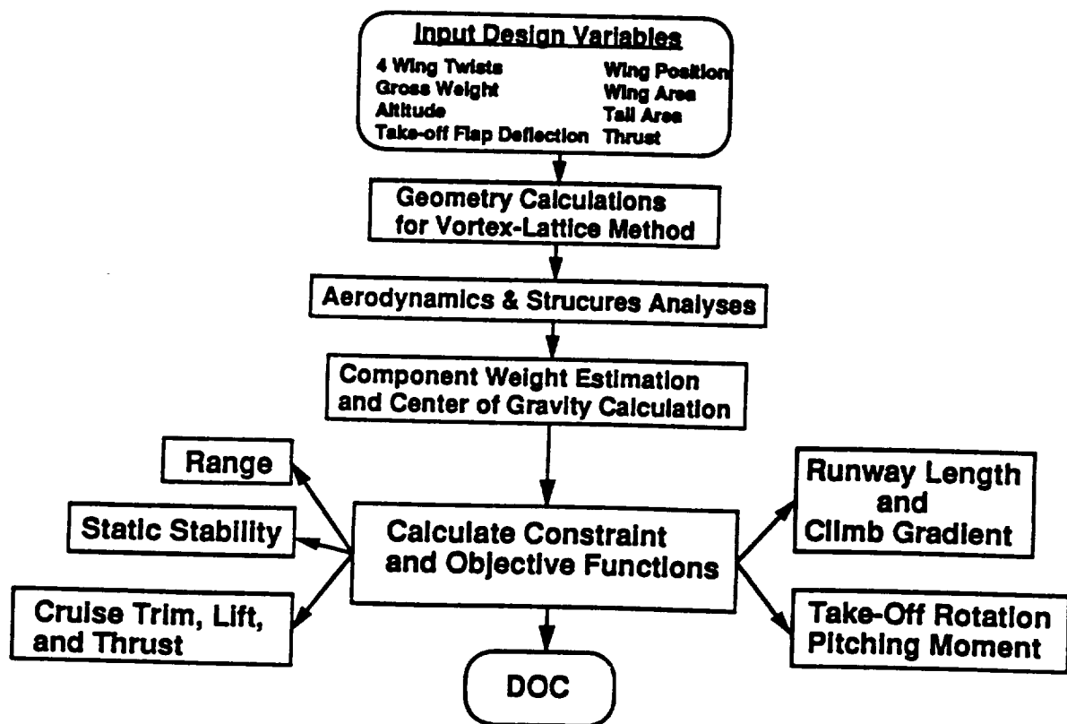
Fig. 4 Design variables, constraints, and a flow chart of the calculations in the design code.
