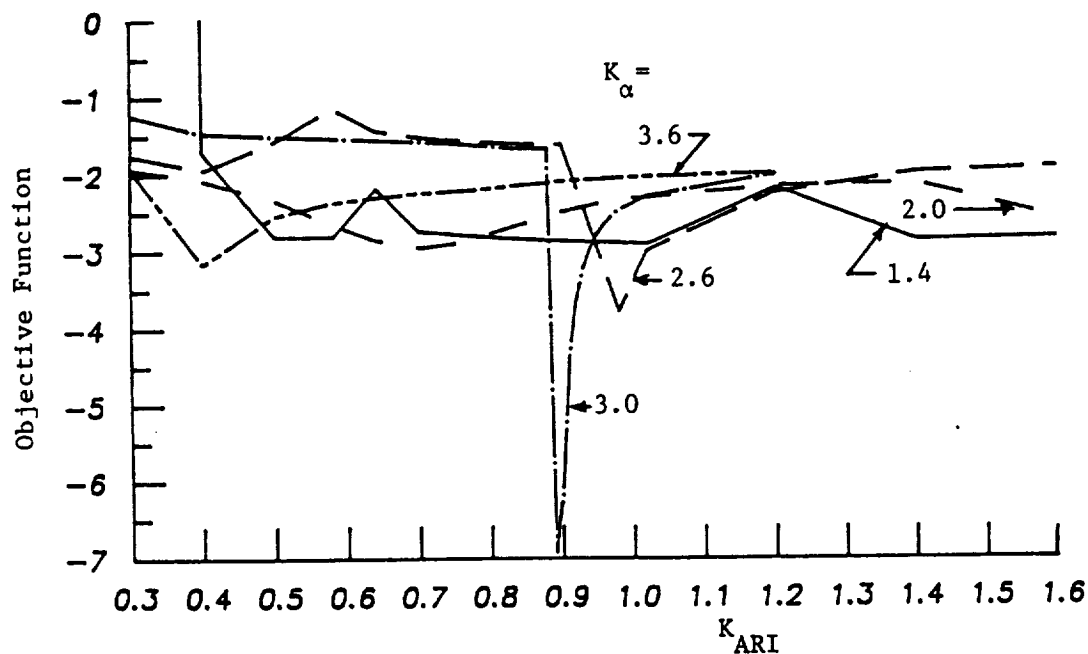
Figure 3 Variation of the Objective Function with K_{ARI} .
