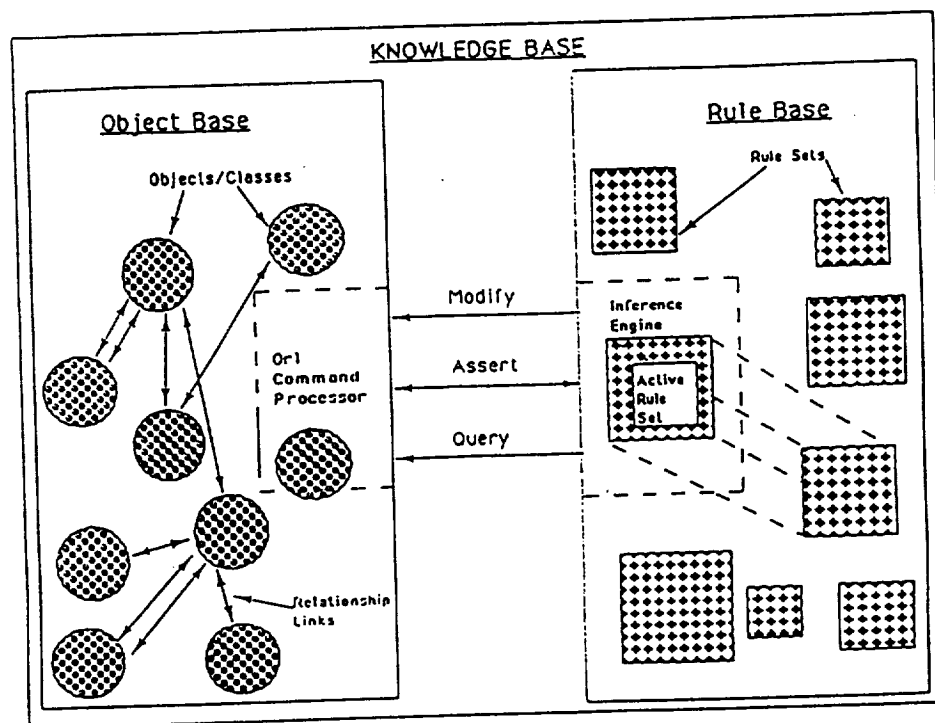
Figure 2. Integrated Object-Oriented/Rule-Based Knowledge Representation Scheme
