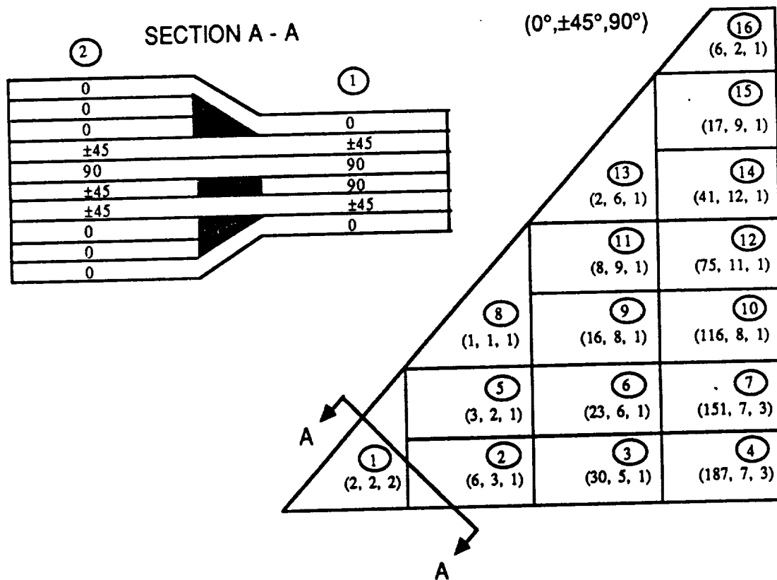
Figure 1. The delta wing designed by Schmit and Fleury required interleaves at several locations, including Section A-A.
