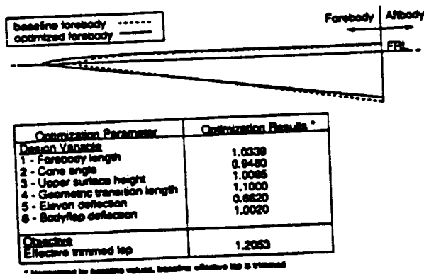
Figure 12. Case 3 results - addition of trim constraint to case 2
