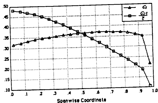
Figure 6. Optimal Lift and C_l Distributions
