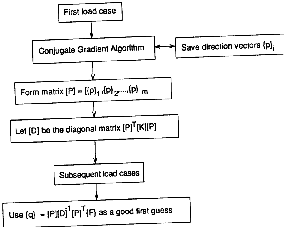
Figure 4. Scheme to improve convergence for multiple load cases.
