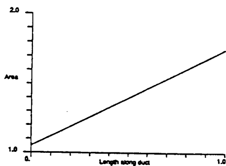
Figure 2a: Area profile, linear duct, using C^0 scheme
