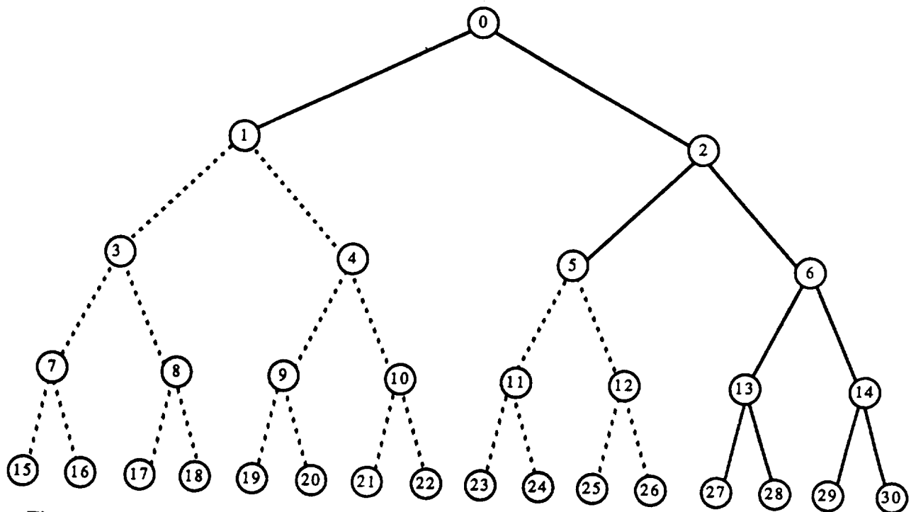
Figure 3. The branch and bound method reduces the number of constraint combinations that must be analyzed.
