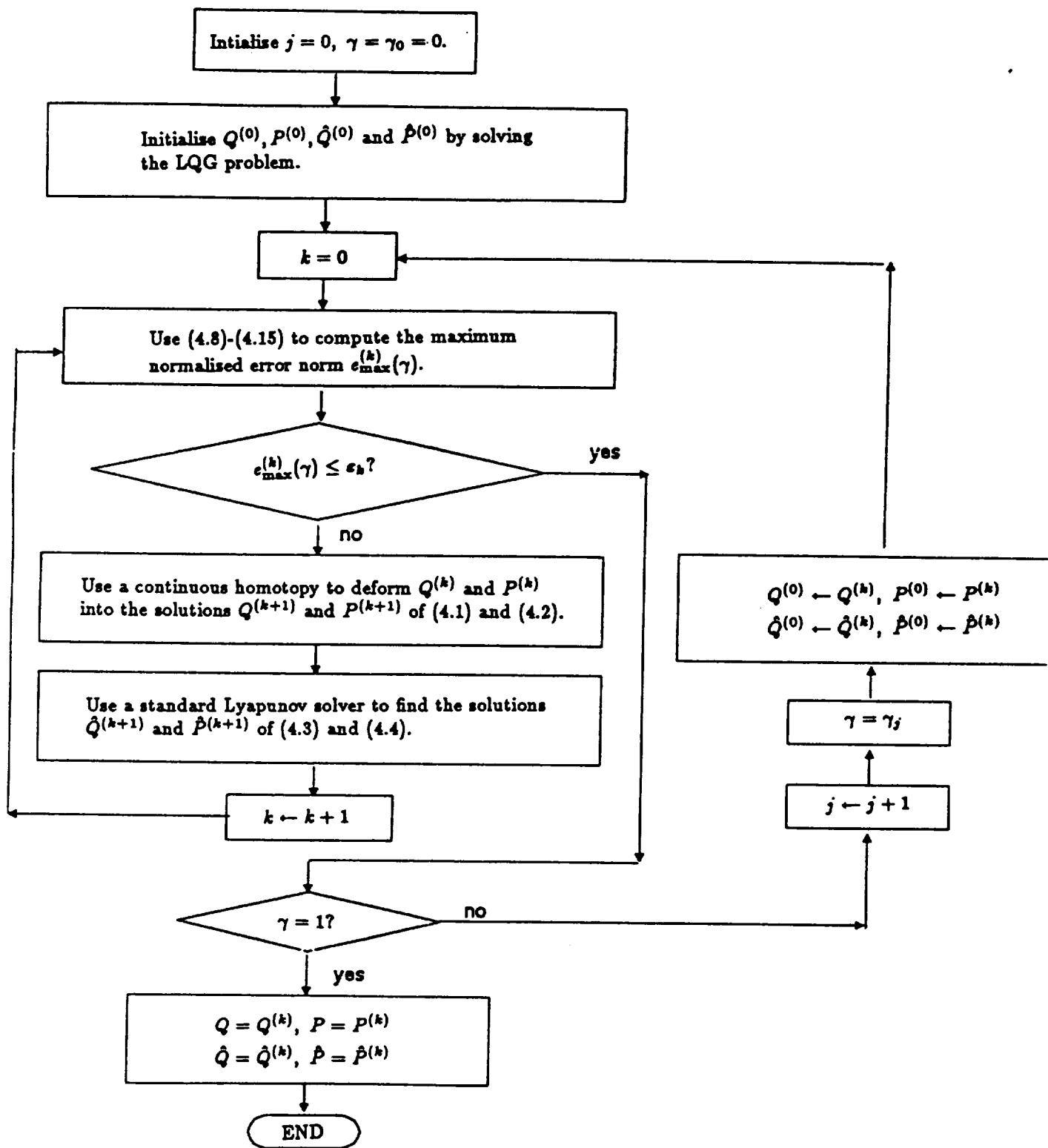
Figure 4.1. Flowchart of the Homotopy Algorithm for Solving the Maximum Entropy Design Equations.
