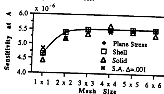
Figure 7—Accuracy of Sensitivity for Plate
