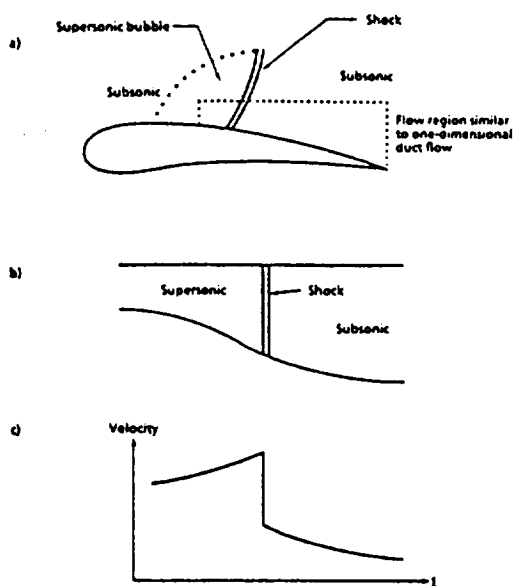
Figure 1: Analogy between a) flow over a transonic airfoil and b) flow in a duct. Of course, the flow in a) is two-dimensional, but is assumed one-dimensional in b). In either case, the velocity along the airfoil surface or along the duct length is qualitatively given in c).
