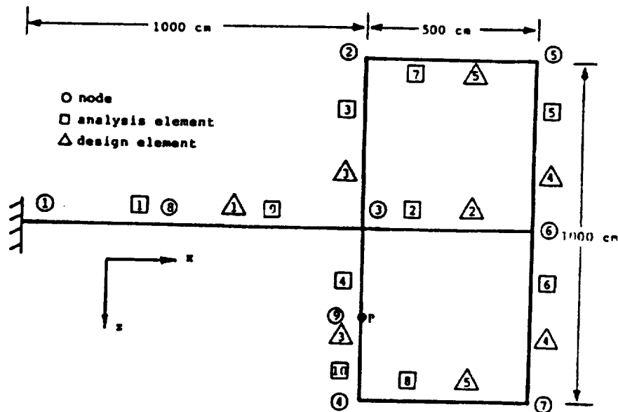
Figure 1. Antenna Structure
