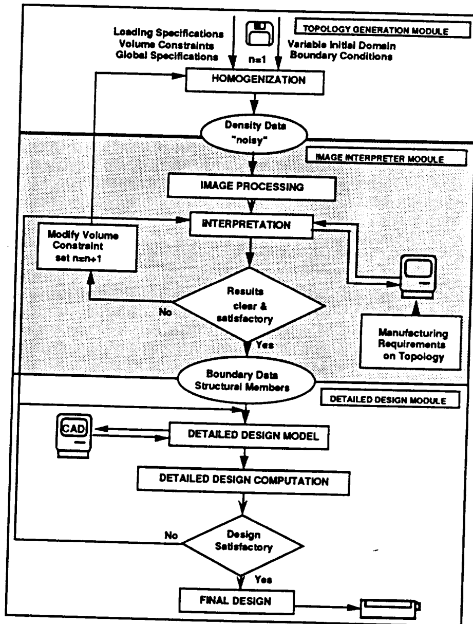
Figure 2. Basic flow chart for the three-phase structural optimization system ISOS.
