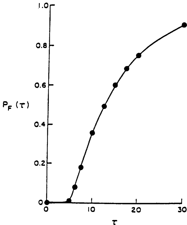
Figure 3. Probability of Failure P_F(\tau) for a Daniels System with n = 5 Fibers.
