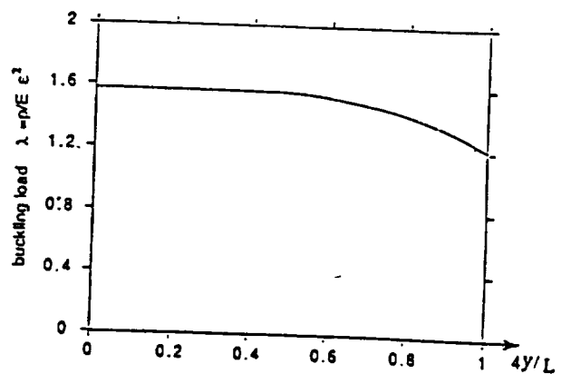
Figure 6 Variations of the buckling load as functions of the position of the delamination. The center of the delamination is at (x,0) and (y,0) , respectively
