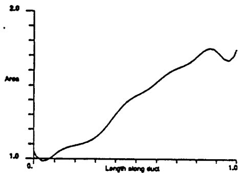
Figure 5a. Area profile, optimal duct with 10 design variables, no design constraints, using C^0 scheme
