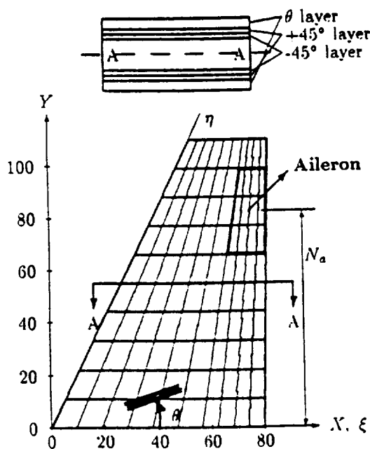
Figure 1: Wing planform geometry.
