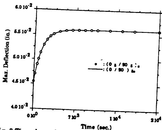
Fig. 3 Time dependent max. bending deflections of simply supported (0_g/90_g)_s and (0/90)_{ss} laminate.
