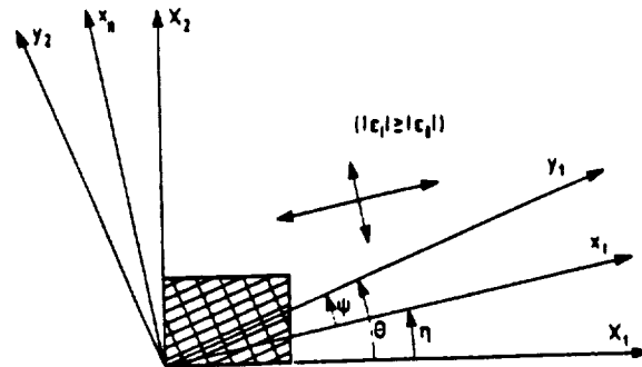
Fig. 1. Definition of the angles \psi , \theta and \eta for mutual rotations of the finite element coordinate system X_1, X_2 , the principal strain coordinate system x_1, x_2 and the material coordinate system y_1, y_2 .
