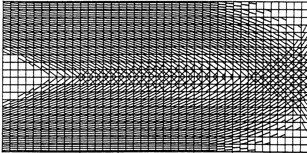
Fig. 5. Optimal distribution and orientation of fibers in second example: Two fiber fields, n=800 , maximization of stiffness
