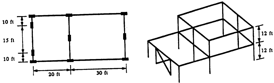
Fig. 1 Topology of the setback frame
