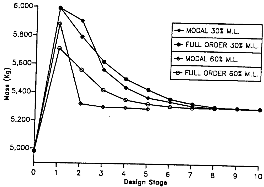
Figure 4. Mass Iteration Histories for Example 1
