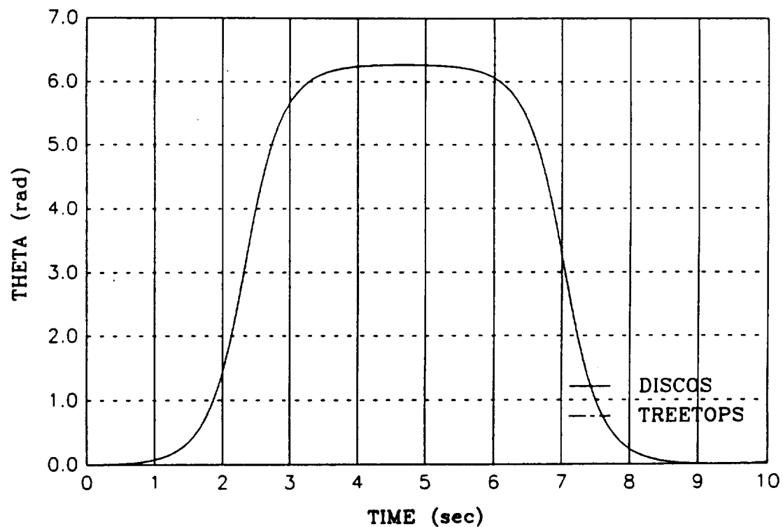
Fig. 4 Time History Response of Hinge - Inverted Pendulum
