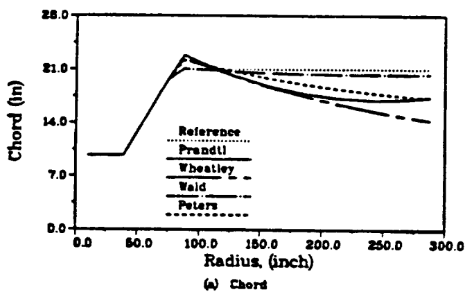
Figure 2 Comparison of Different Blade Tip Loss Formulations.
