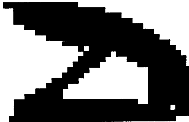
Figure 10. Optimum material distribution for Example 3 (solid/void ratio=1/1)
