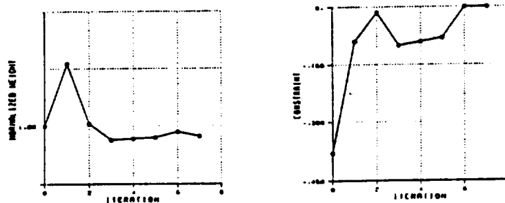
Figure 2: Weight and constraint history for Ariane propulsion stage
