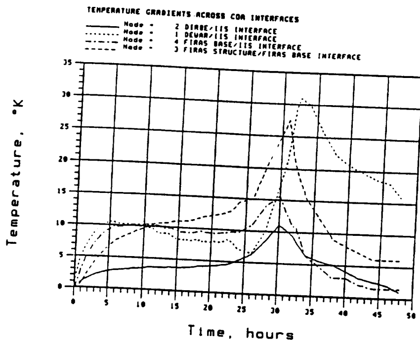
Figure 3. Average Temperature Gradients Across COA Interfaces
