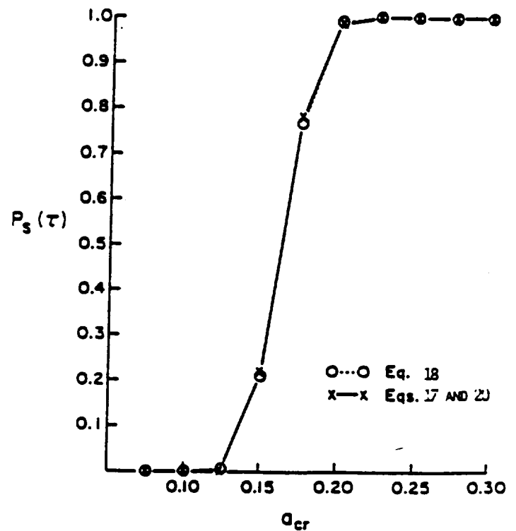
Figure 4. Reliability of Plate in Fig. 2.
