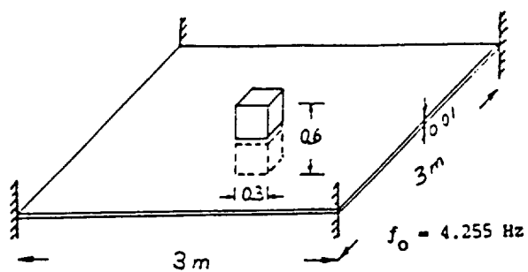
(a) SQUARE PLATE WITH NONSTRUCTURAL MASS AT THE CENTER
