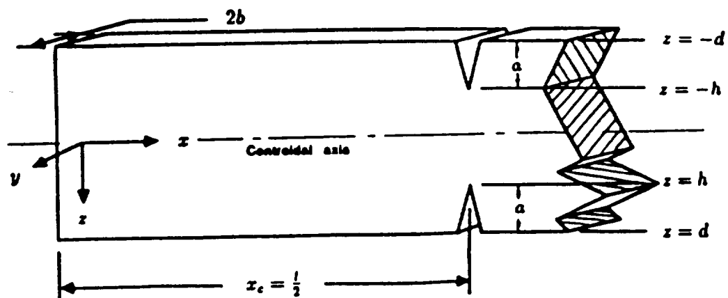
Figure 1. Geometry of a simply supported beam containing a pair of symmetric edge cracks at mid-span, x_c = \frac{l}{2} .
