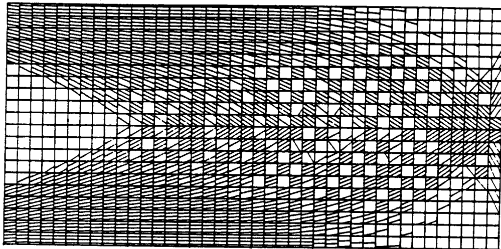
Fig. 4. Optimal distribution and orientation of fibers in first example: One fiber field, n=800 , maximization of stiffness
