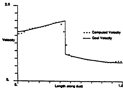
Figure 5b. Velocity profile, optimal duct with 10 design variables, no design constraints, using C^0 scheme
