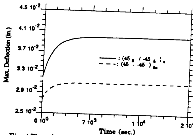
Fig. 4 Time dependent max. bending deflections of simply supported (45/-45)_{ss} and (45_g/-45_g)_s laminate.
