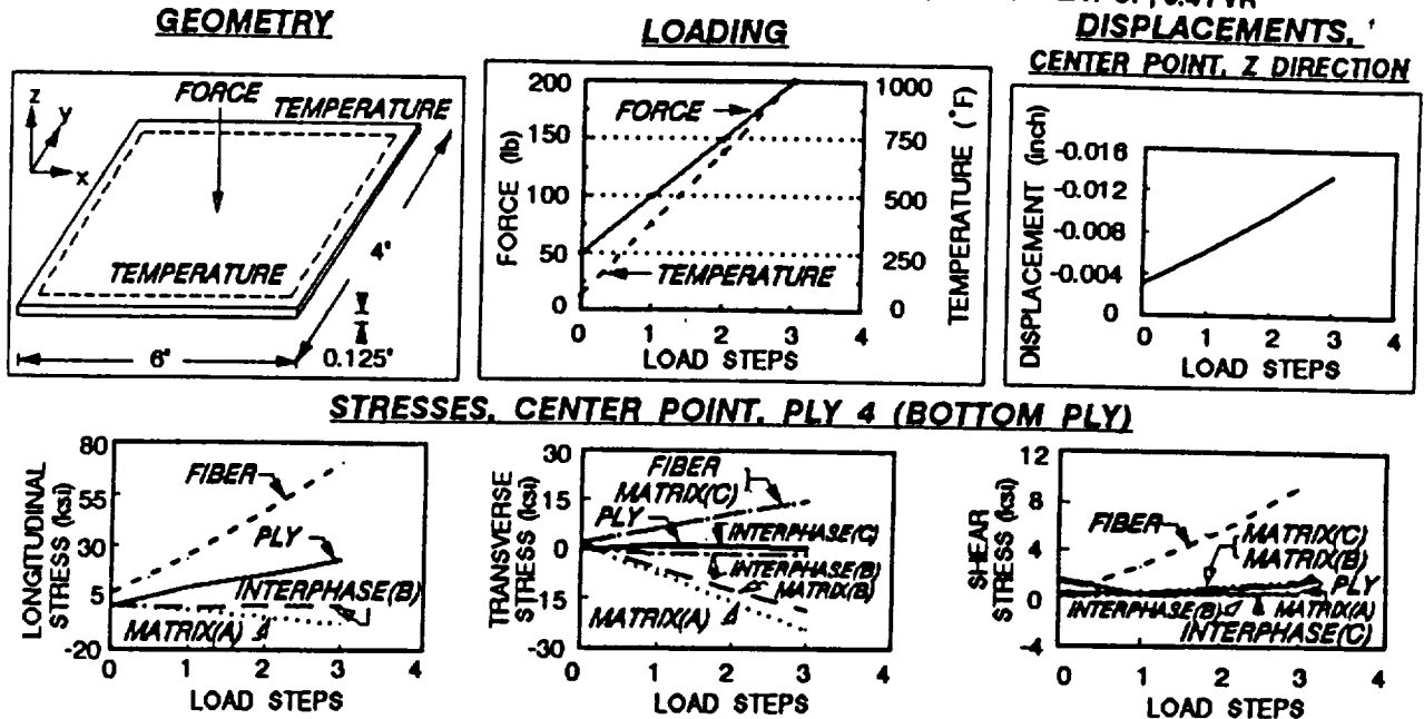
FIGURE 4 - LOAD STEPPING ANALYSIS: SENSITIVITY CASES SENSITIVITY ANALYSIS AT LOAD STEP 3 FABRICATION COOLING LOAD
