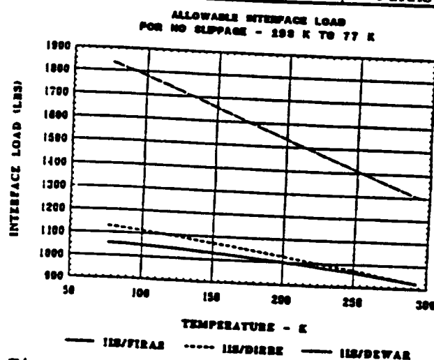
Figure 5. Allowable Interface Loads
