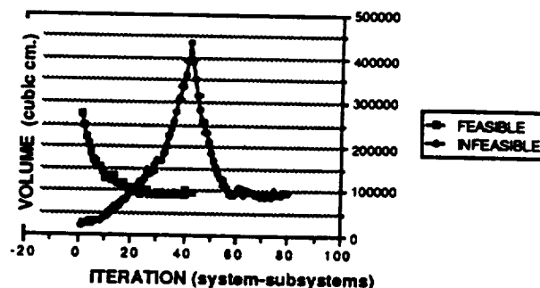
FIGURE 3: PORTAL FRAME CONVERGENCE
