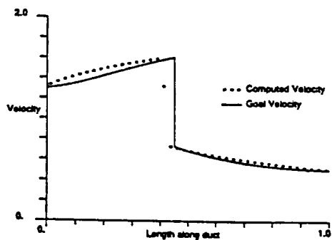
Figure 2b: Velocity profile, linear duct, using C^0 scheme
