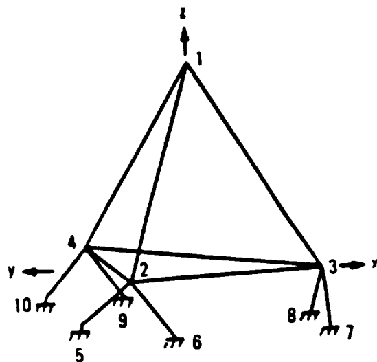
FIGURE 1: ACOSS-FOUR structure
