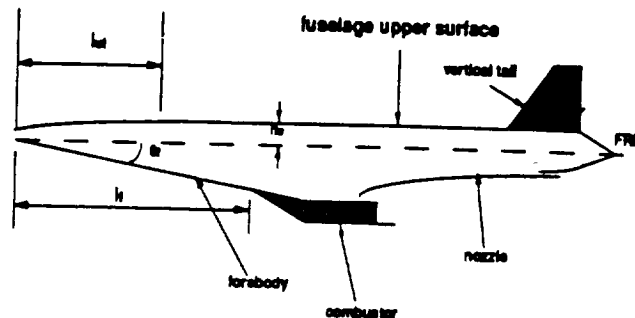
Figure 2. Baseline configuration
