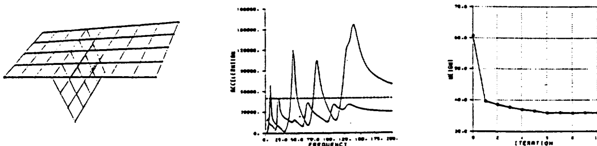
Figure 7: a) cantilever plate b) amplitude response spectra c) weight history
