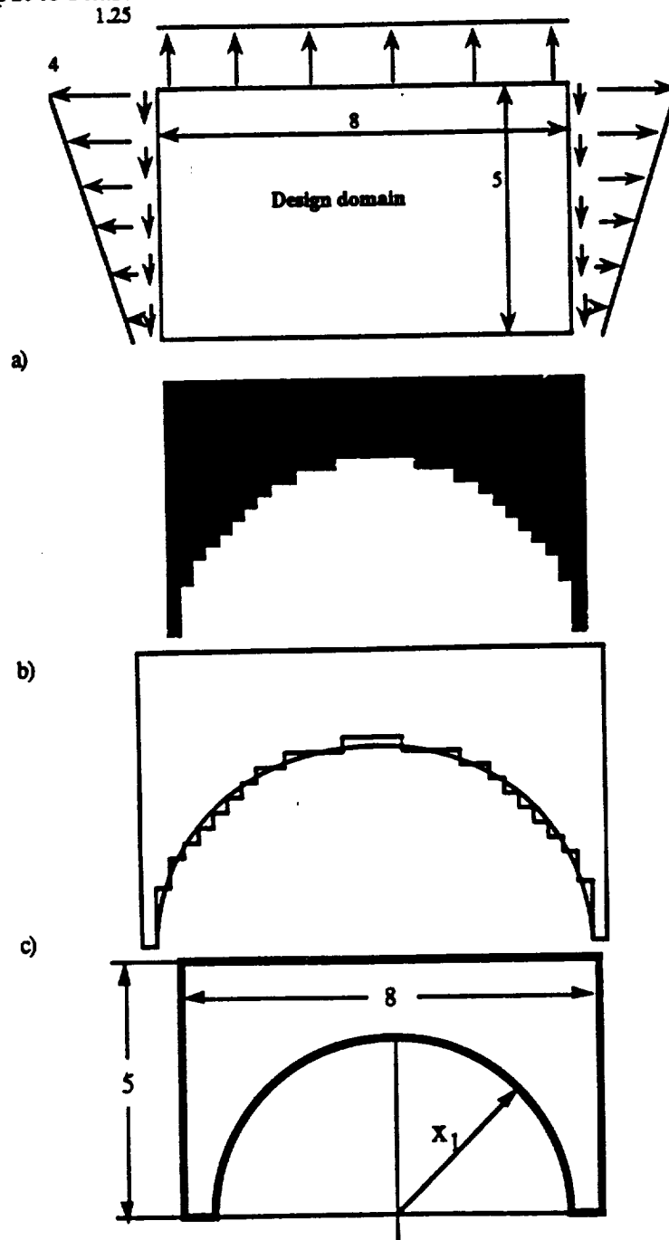
Figure 3. Design example 1: a) design domain and boundary conditions; b) density distribution generated by homogenization; c) processed image; d) user interpretation and detailed design model (design variable x_1 ).
