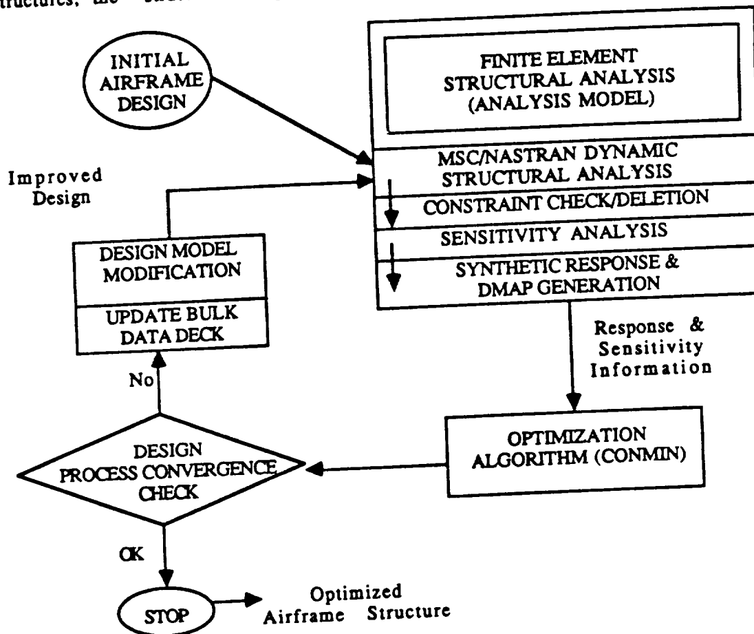
Figure 1. General Airframe Structural Optimization Methodology
