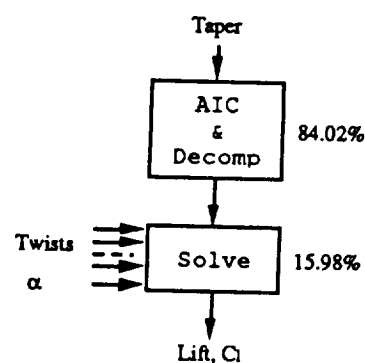
Figure 5. Structure of the Analysis Routines
