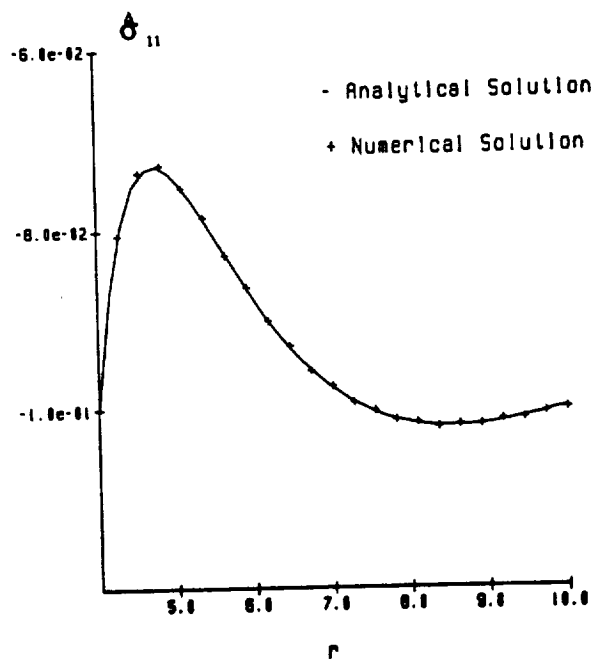
Figure 2. \sigma_{11}^{\Delta} on DC--analytical and DBEM solution.
