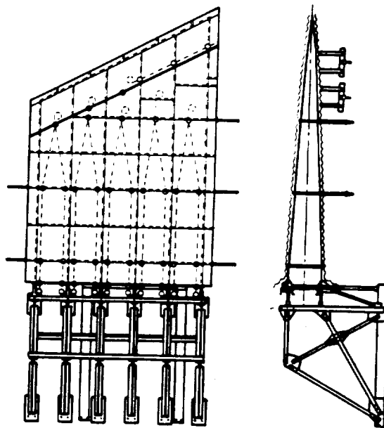
FIGURE 2 - HYPERSONIC WING TEST STRUCTURE (HWTS)
