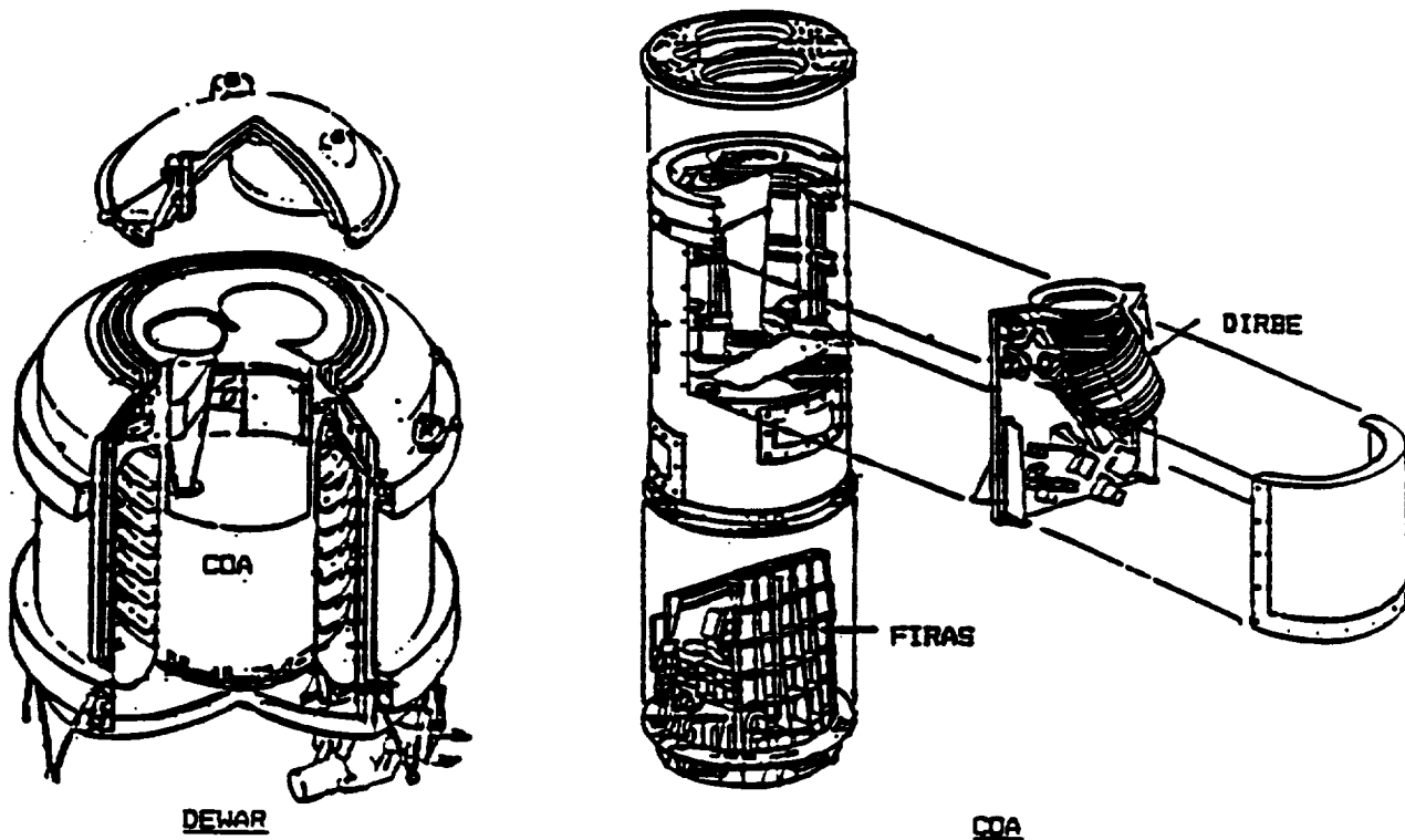
Figure 1. Dewar and COA
