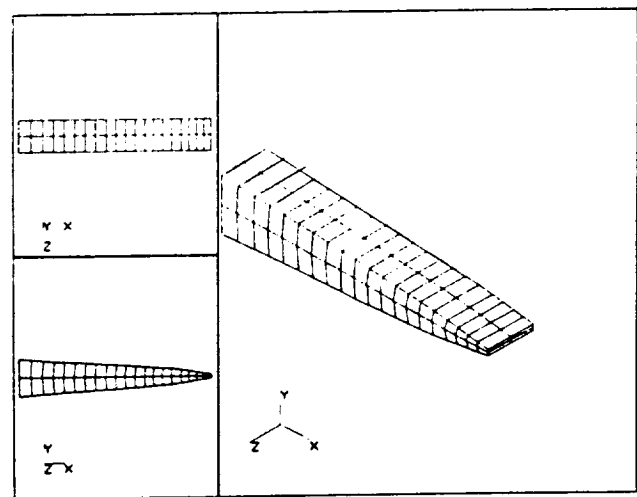
Figure 7: Constrained cantilever beam optimal design.
