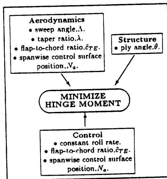
Figure 2: Wing design synthesis(first example).
