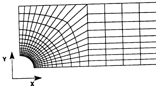
Fig. 8 Finite element mesh for GY70/339 composite plate with a circular hole
