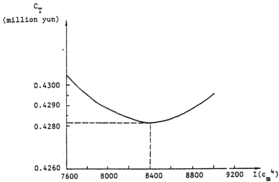
Fig. 6. Cross section ( I ) vs. cost ( C_T )
