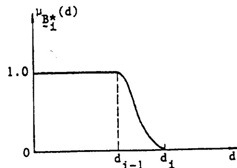
Fig. 5. Membership function of fuzzy safe region
