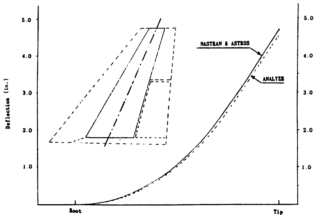
Figure 2 - Typical Deflection Curve Along 50% Chord Line
