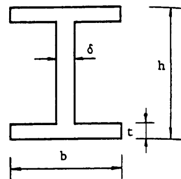
Fig. 3. Cross section
