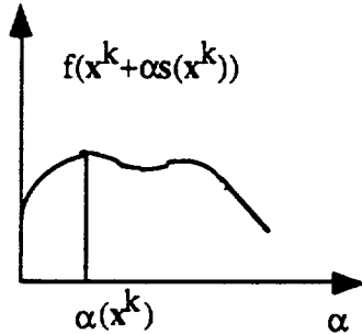
Figure 2 Exact line search
