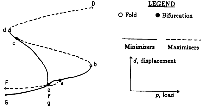
Fig 4.1: Feasible Solutions of (2.1)
