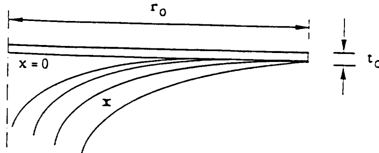
Fig. 2: Circular plate with variable thickness
