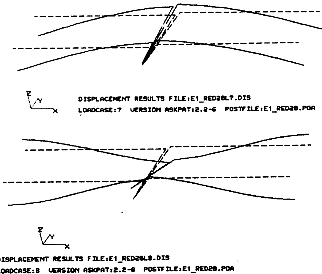
Figure 2: Free-free modes computed with the Craig-Bampton model.
