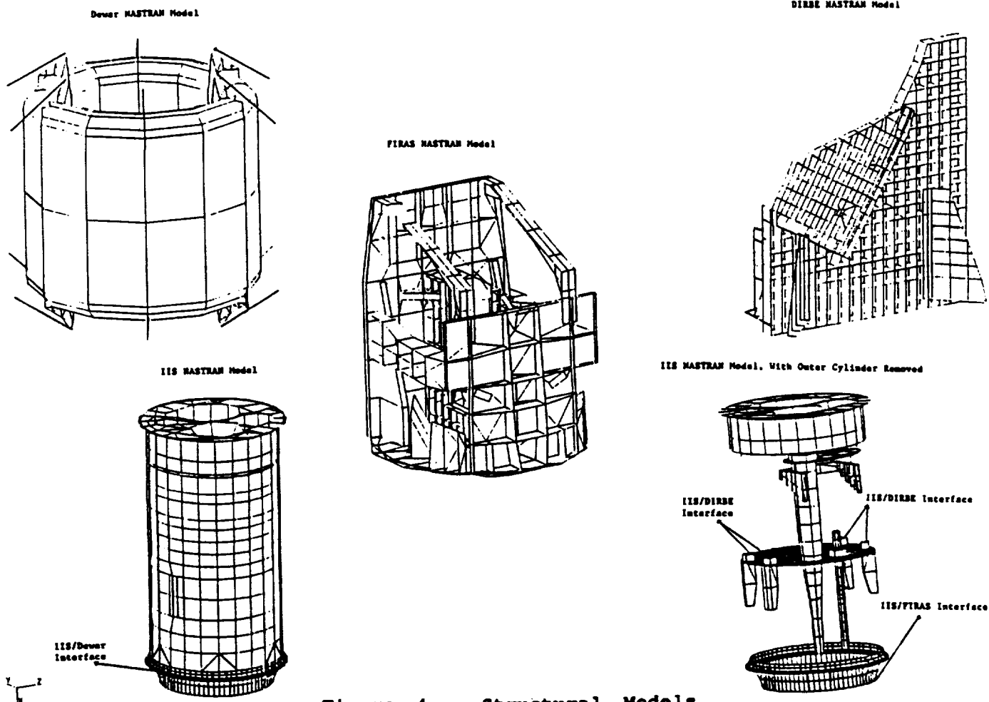
Figure 4. Structural Models
