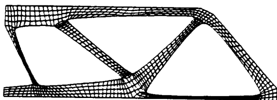
Fig. 4. Final finite element model.
