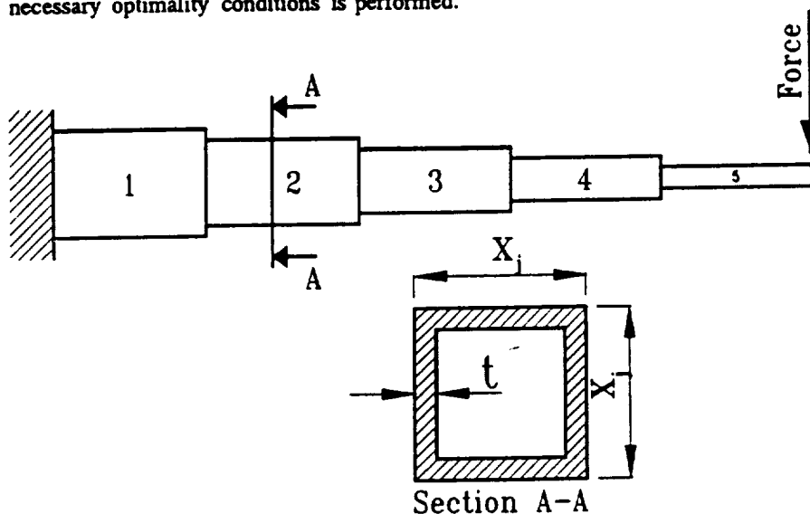
Fig. 2. Cantilever beam with 5 sizing design variables.
