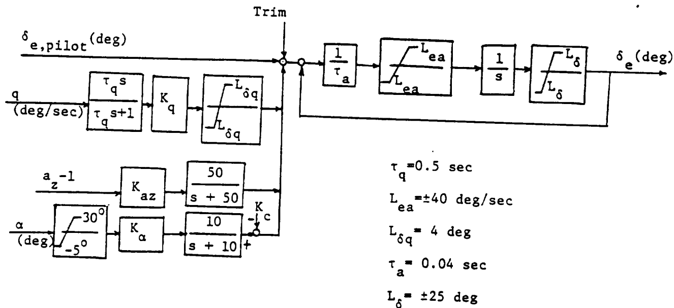
Figure 1 Block Diagram of an Assumed Pitch Control System for an F-16 Configuration
