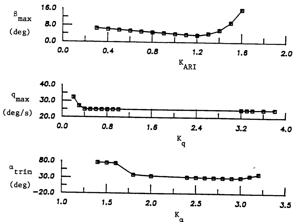
Figure 2 A Sensitivity Analysis of the Effect of System Gains on Dynamic Characteristics
