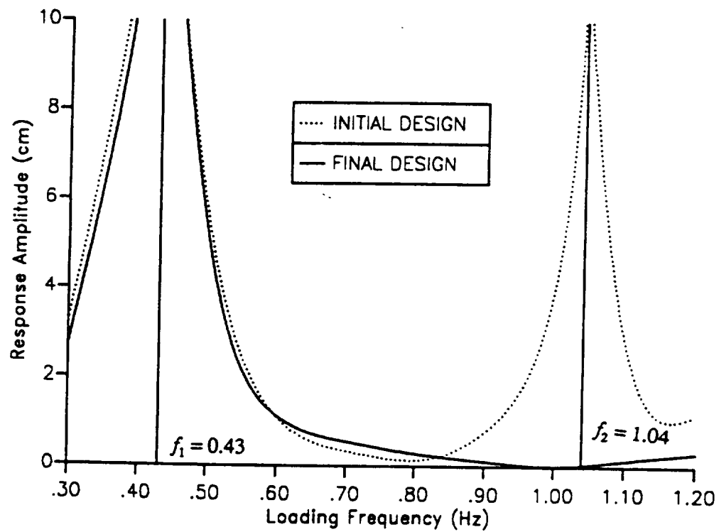
Figure 3. Structural Response at Various Frequencies
