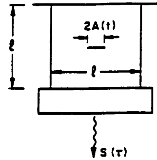
Figure 2. Plate with Initial Crack of Length 2a_0
