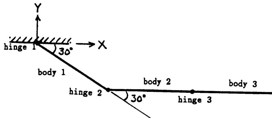
Fig.1B A Triple Pendulum System
