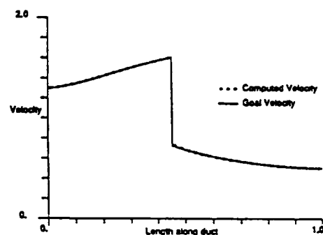
Figure 3b: Velocity profile, optimal duct with 10 design variables, no design constraints, using C^0 scheme
