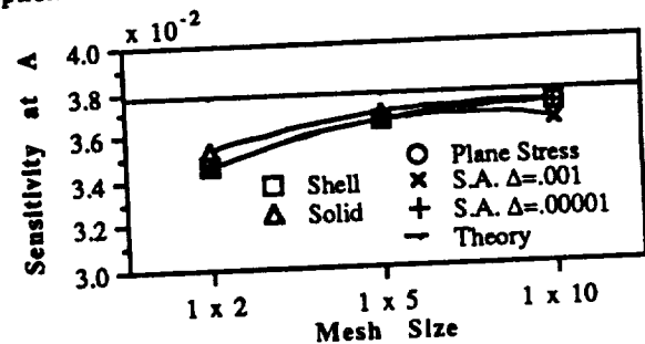
Figure 4—Accuracy of Sensitivity for Beam
