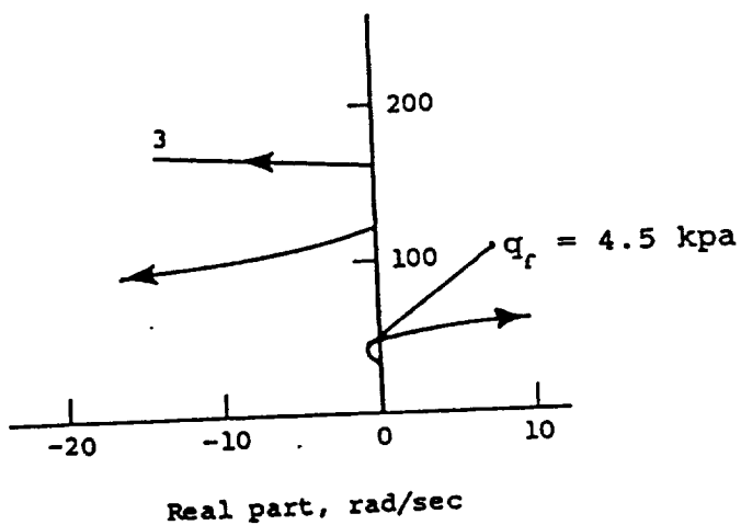
Fig. 7 Dynamic pressure root locus.
