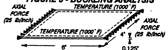
FIGURE 6 - BUCKLING ANALYSIS
