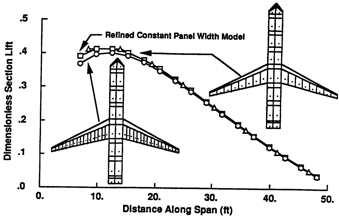
Fig. 3 Lift distributions calculated with and without a panel width discontinuity at the wing-fuselage joint.
