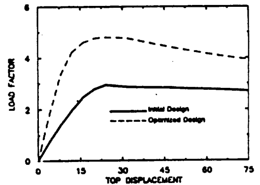
Fig. 3 Response of setback structure under one load case
