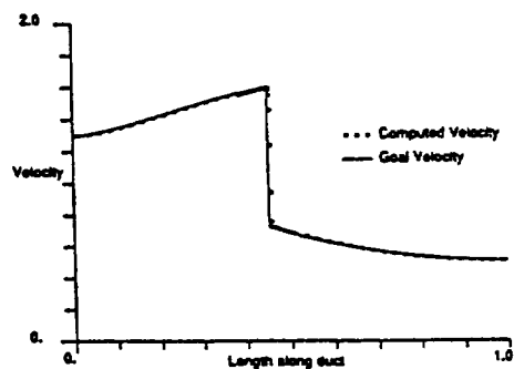
Figure 9. Velocity profile of optimal duct using grid refinement and the C^0 scheme
