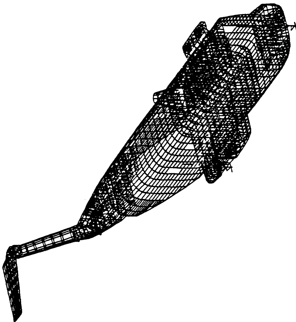
Figure 2. Finite Element Model of the MH-53J Helicopter
