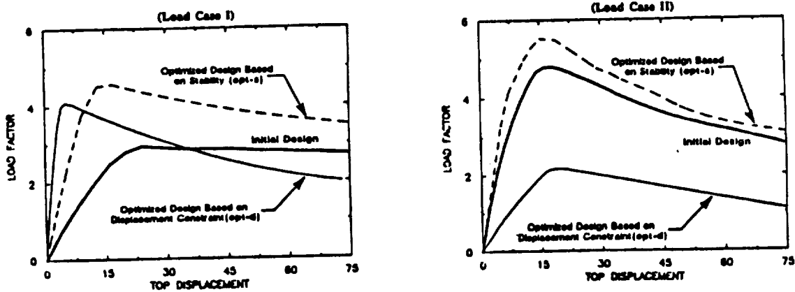
Fig. 4 Comparison of displacement constraint and stability based optimization
