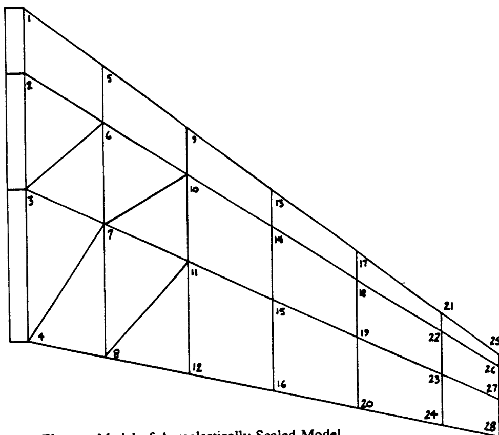
Figure 2. Finite Element Model of Aeroelastically Scaled Model.
