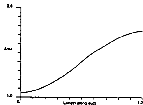
Figure 3a: Area profile, optimal duct with 10 design variables, no design constraints, using C^0 scheme
