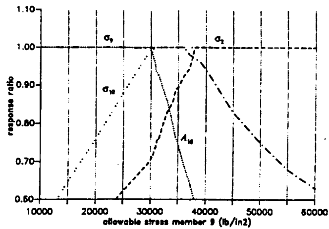
Figure 3. Changes in Active Constraints for Ten Bar Truss Example.
