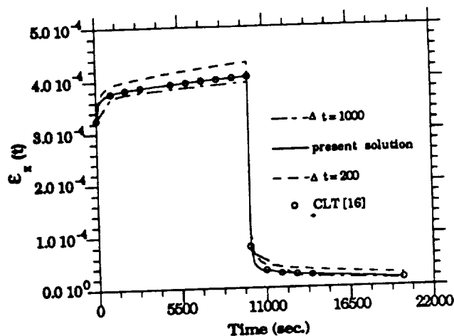
Fig. 6 Time dependent in-plane strain of (45/-45)_s graphite/epoxy laminate (Temp.=140 °F).
