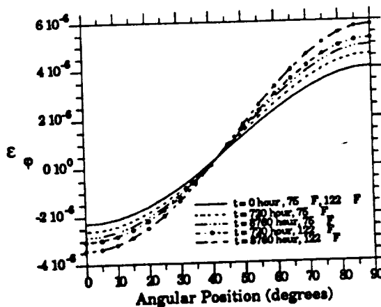
Fig. 10 Circumferential creep around a hole in GY70/339 (45/-45)_s laminate
