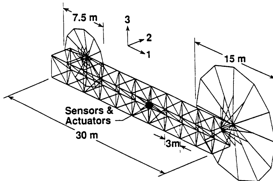
Figure 1. Generic geostationary platform.
