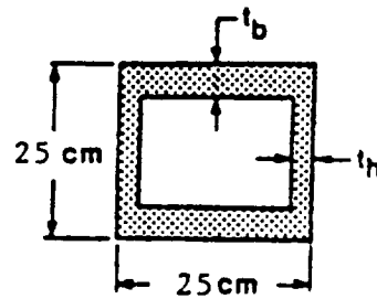
Figure 2. Beam Element Cross Section
