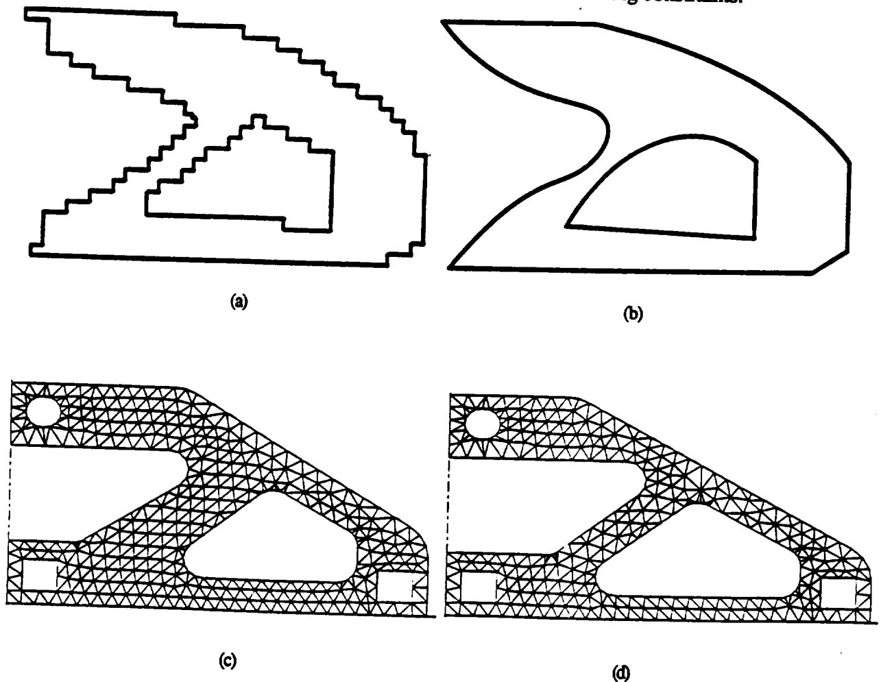
Figure 11 (a) Non-smooth and (b) smooth boundary representation of image shown in Fig. 10; finite-element models of (c) initial and (d) final bracket design.
