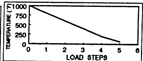
FIGURE 4 - LOAD STEPPING ANALYSIS: SENSITIVITY CASES SENSITIVITY ANALYSIS AT LOAD STEP 3 FABRICATION COOLING LOAD
