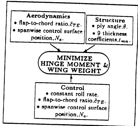
Figure 3: Wing design synthesis(second example).
