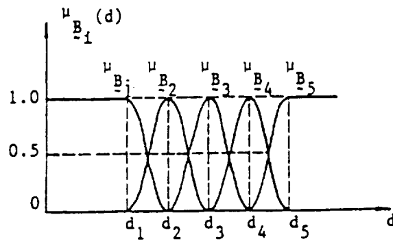
Fig. 4. Membership function of fuzzy damage grades
