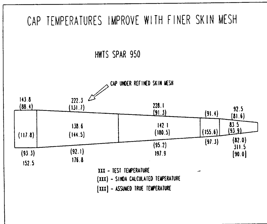
FIGURE 10 - SPAR TEMPERATURES AFTER LOCAL REFINEMENT
