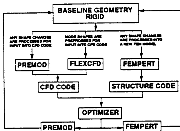
Figure 7. Pre/postprocessors
