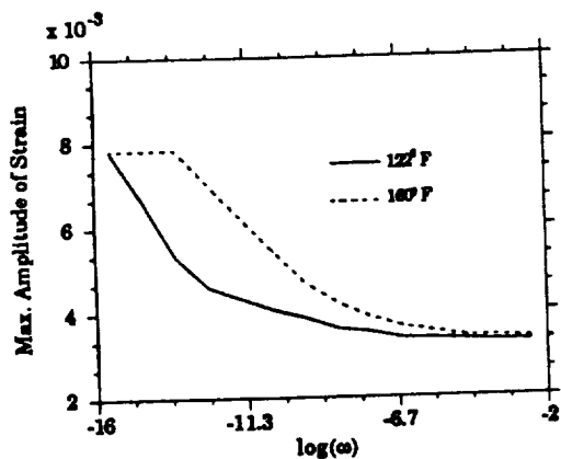
Fig. 7 Max. strain amplitudes of (45/-45)_s graphite/epoxy laminate vs frequency.
