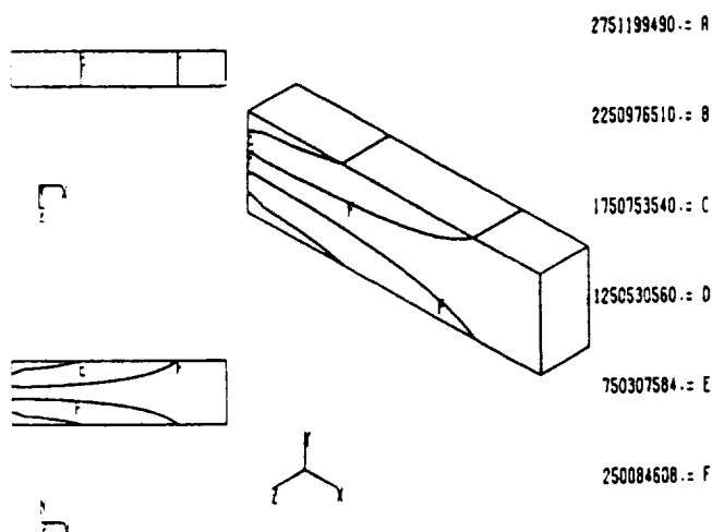
Figure 3: Cantilever beam initial design stress contours.
