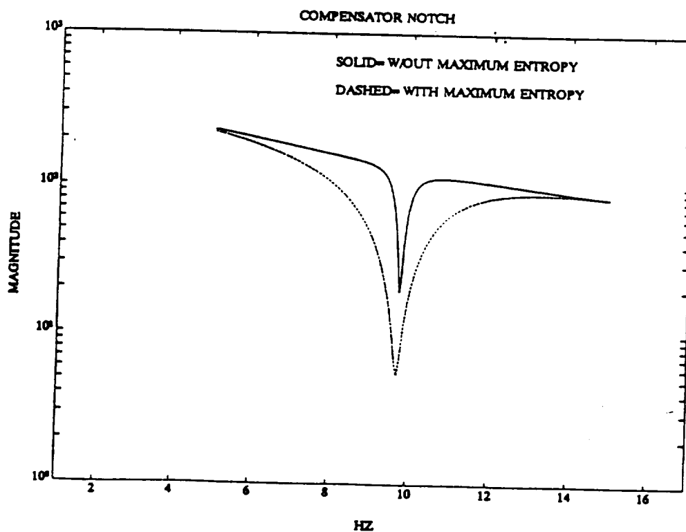
Figure 5.4. For the AGS to BGYRO loops Maximum Entropy design robustified the notches for the high frequency modes by increasing their width and depth.
