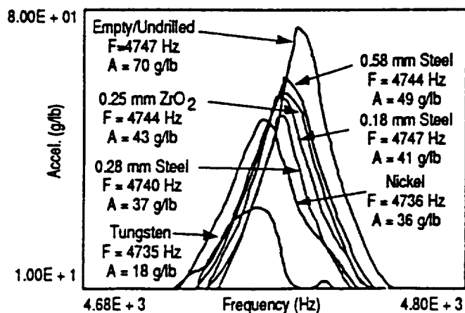
Figure 7. Accelerance Plots to Show Damping with Various Materials for a Torsional Mode of the LOX Inlet Tee Splitter Vane
