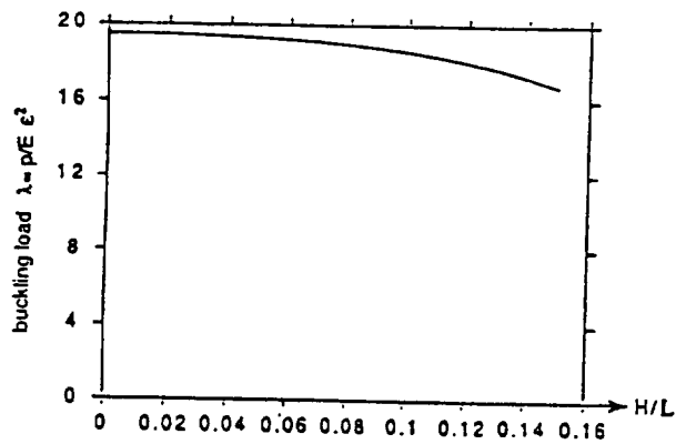
Figure 4 Effect of the plate thickness on the buckling load for a square delamination
