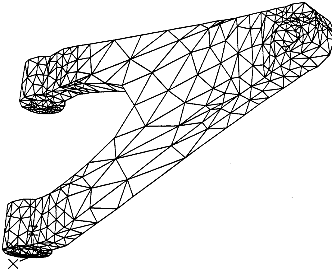
Fig. 3 Control Arm Mesh
