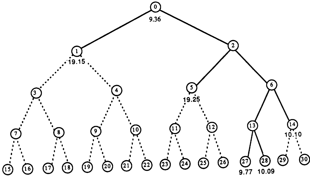
Figure 7. Checking all the branches required only six optimization runs, because most nodes cannot satisfy all the design constraints without a significant increase in weight.
