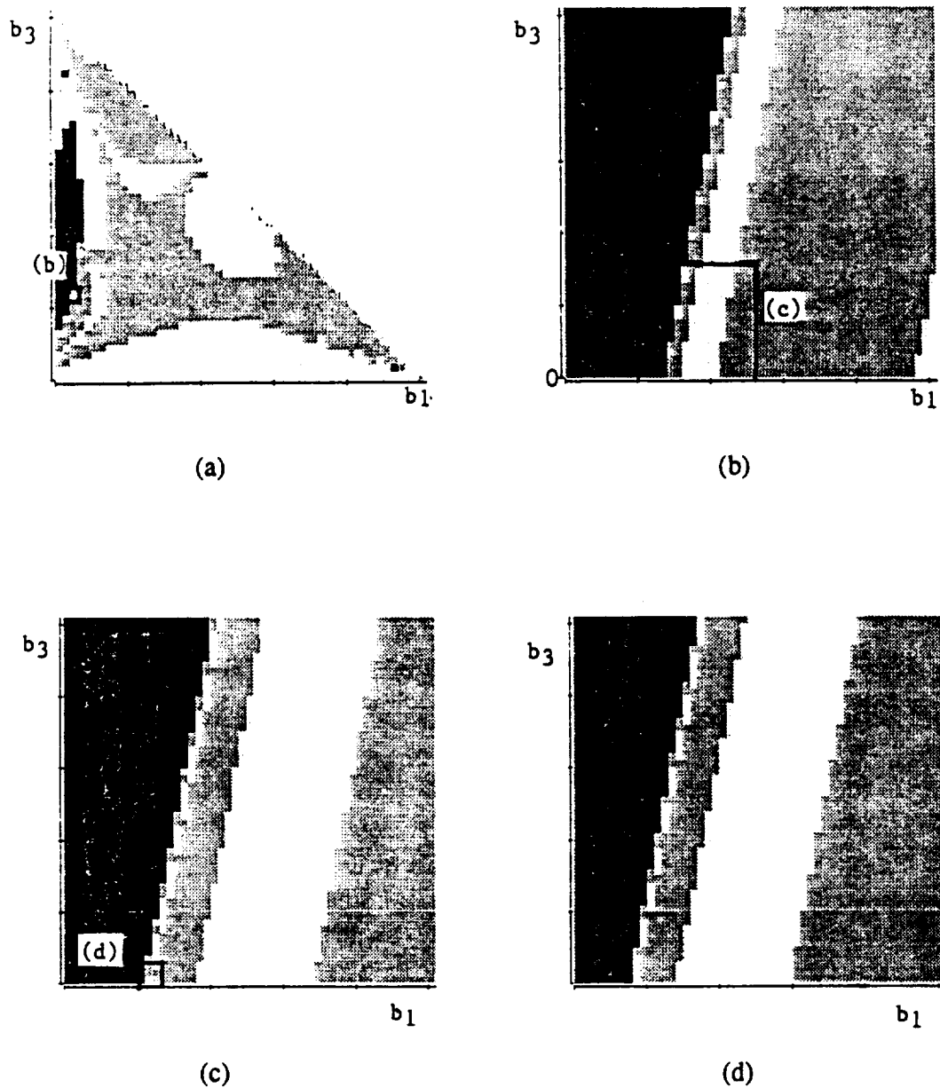
Figure 5 Domains of convergence for inexact line search
