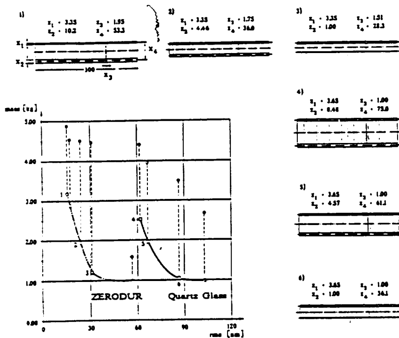
Fig. 5: p-efficient solutions of a mirror plate
