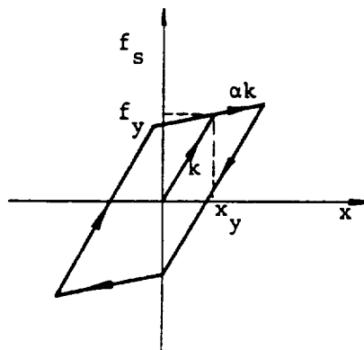
Fig. 2. Restoring force model
