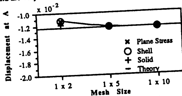
Figure 3—Accuracy of Displacement for Beam.
