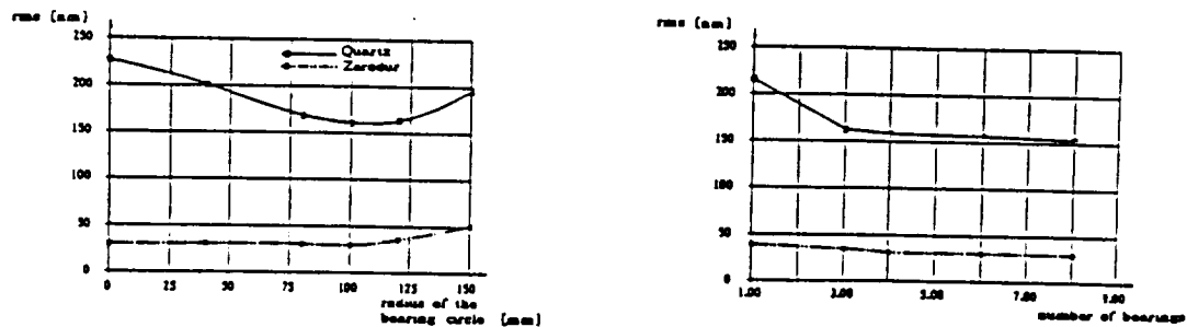
Fig. 6: Optimal ratio of support radii and optimal number of support points
