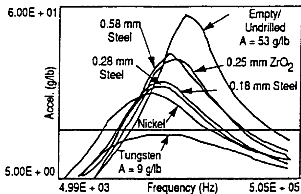
Figure 5. Accelerance Amplitudes of a Torsional Mode at 5021 Hz Under Various Materials
