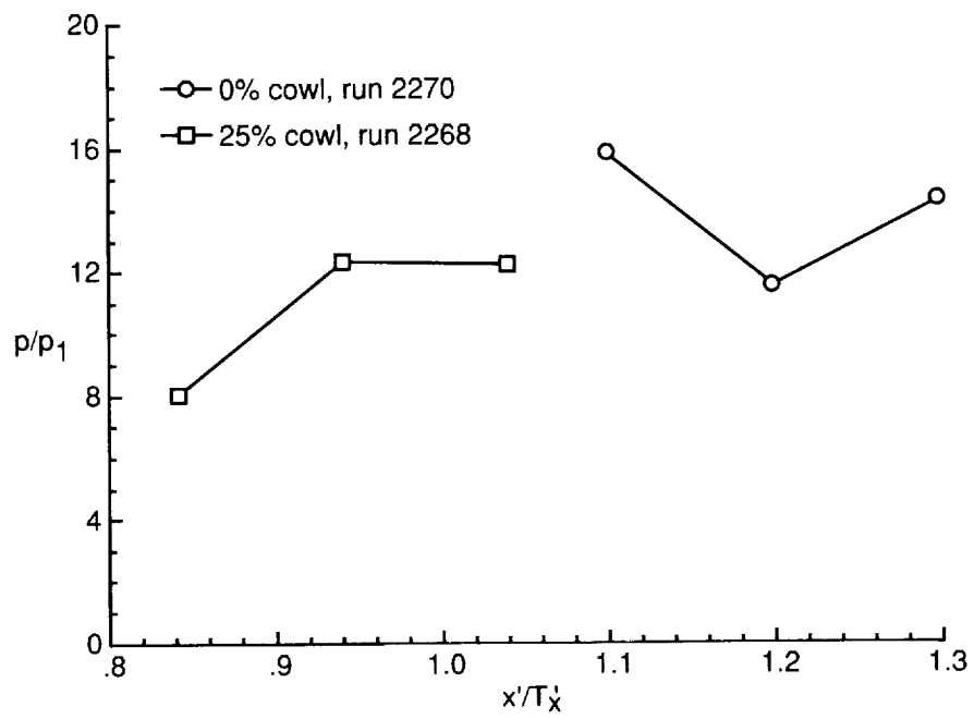
(e) Cowl centerline. Figure 17. Concluded.
