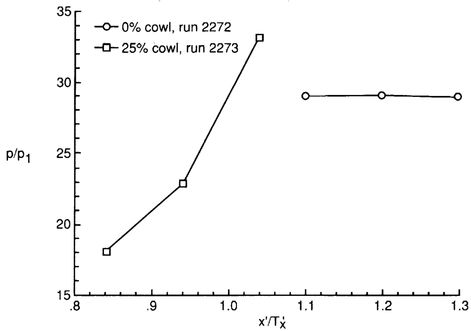
(e) Cowl centerline.
