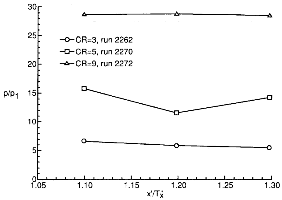
(e) Cowl centerline.
