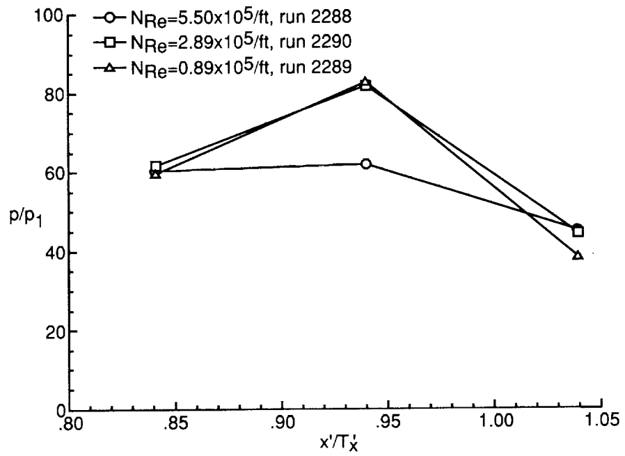
(e) Cowl centerline. Figure 23. Concluded.
