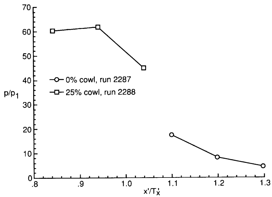
(e) Cowl centerline.
