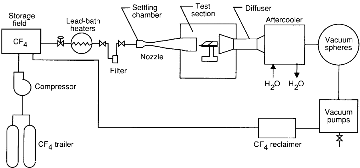
Figure 5. Schematic drawing of the Langley Hypersonic CF 4 Tunnel.
