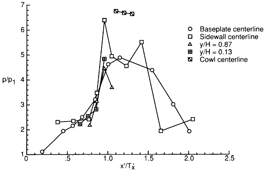
(e) Run 2266. CR = 3; 0-percent cowl; N_{Re} = 2.85 \times 10^5 per foot.
