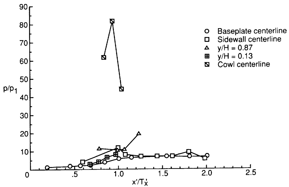
(o) Run 2290. CR = 9; 25-percent cowl; N_{Re} = 2.85 \times 10^5 per foot.
