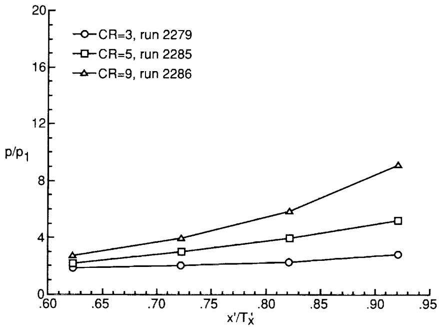
(b) Sidewall at y/H = 0.13 .
