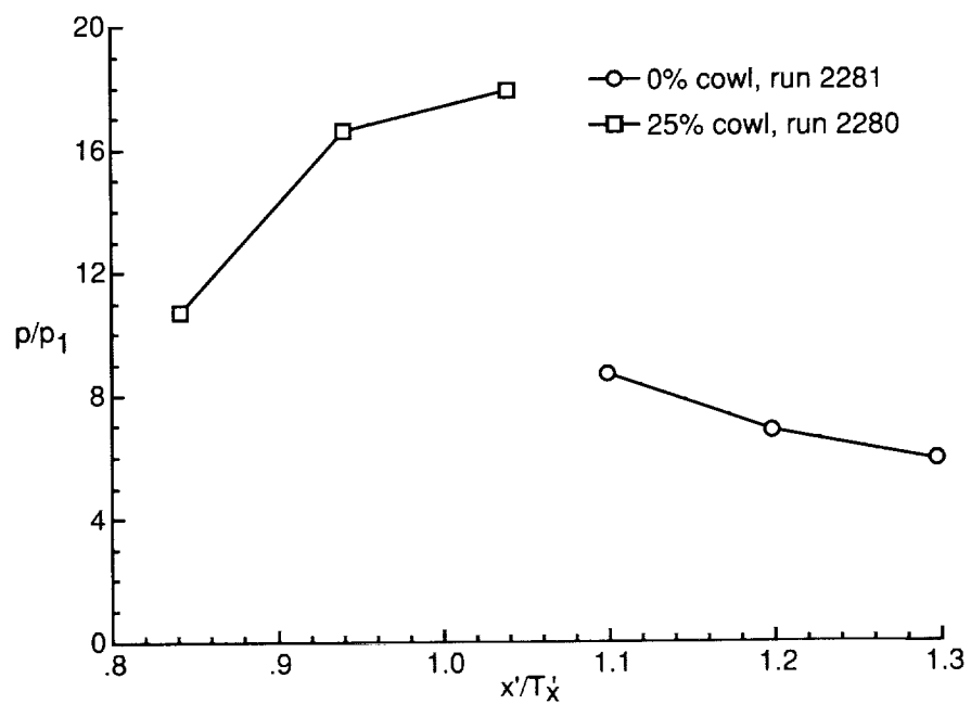
(c) Cowl centerline.
