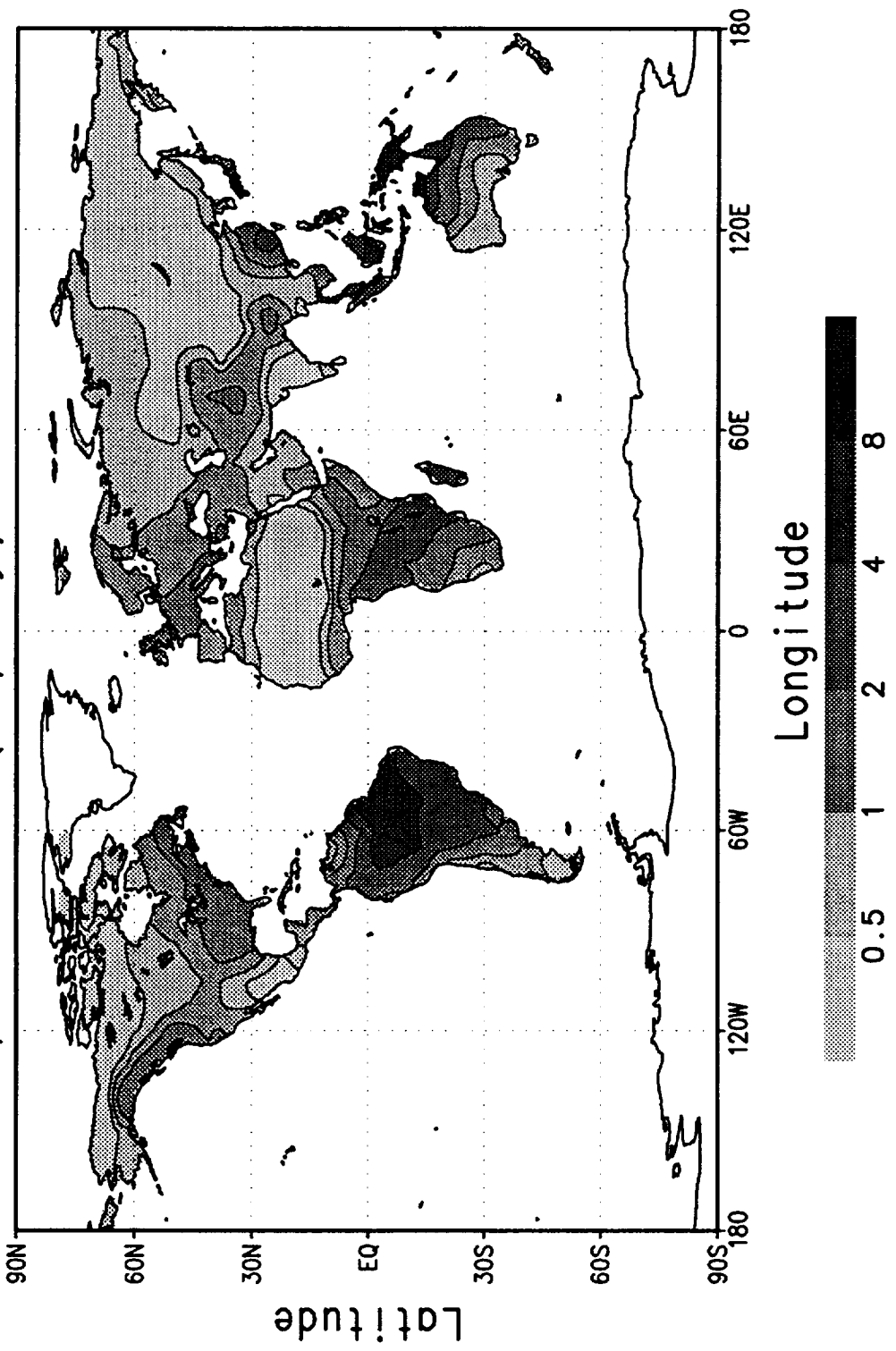
Precipitation (mm/day) March 1979-88
