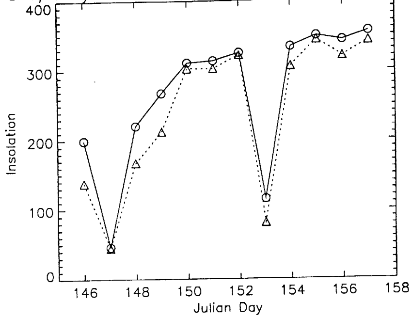
IFC 1, Daily Insolation, Satellite (.....) and Insitu (—)
