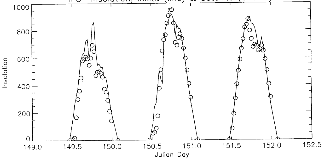
IFC1 Insolation, Insitu (line) & Satellite (circles)
