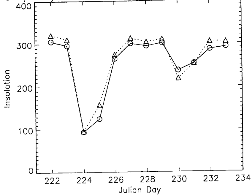
IFC 3, Daily Insolation, Satellite (.....) and Insitu (—)
