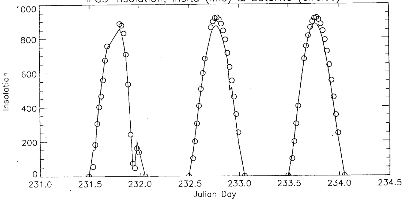
IFC3 Insolation, Insitu (line) & Satellite (circles)
