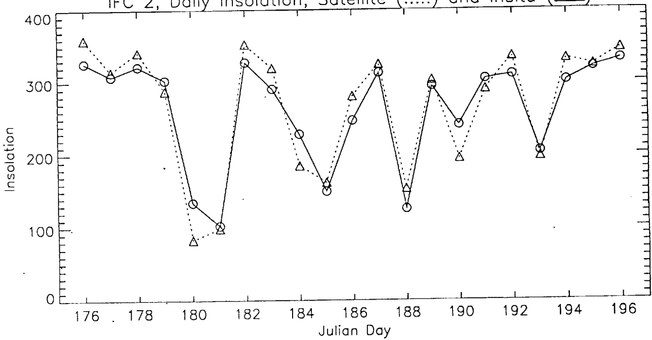
IFC 2, Daily Insolation, Satellite (.....) and Insitu (—)
