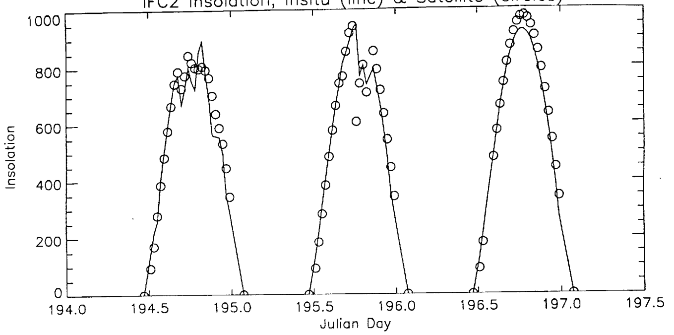
IFC2 Insolation, Insitu (line) & Satellite (circles)
