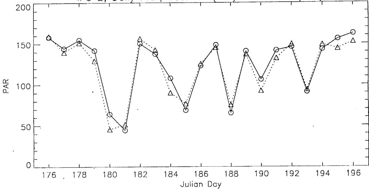
IFC 2, Daily PAR, Satellite (.....) and Insitu (—)
