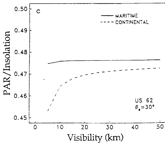
Fig. 2. Ratio of photosynthetically available radiation, PAR, and insolation as a function of water vapor amount (top), ozone amount (middle), and aerosol type and visibility (bottom). (After Baker and Frouin, 1987.)
