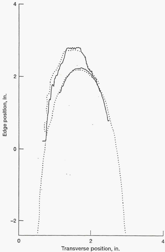
Figure 2.—Optical tracing (solid line) and hand tracing (dotted line) for rime ice accretion.
