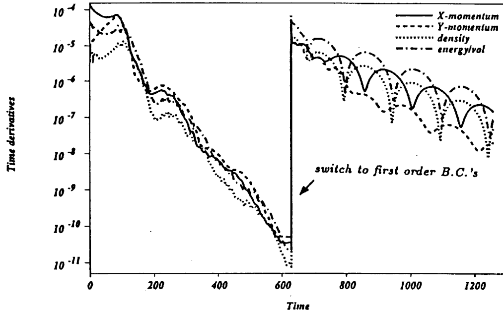
FIGURE 8. Cold jet: History of space averaged time derivatives with switch from zeroth order to first order BC's.
