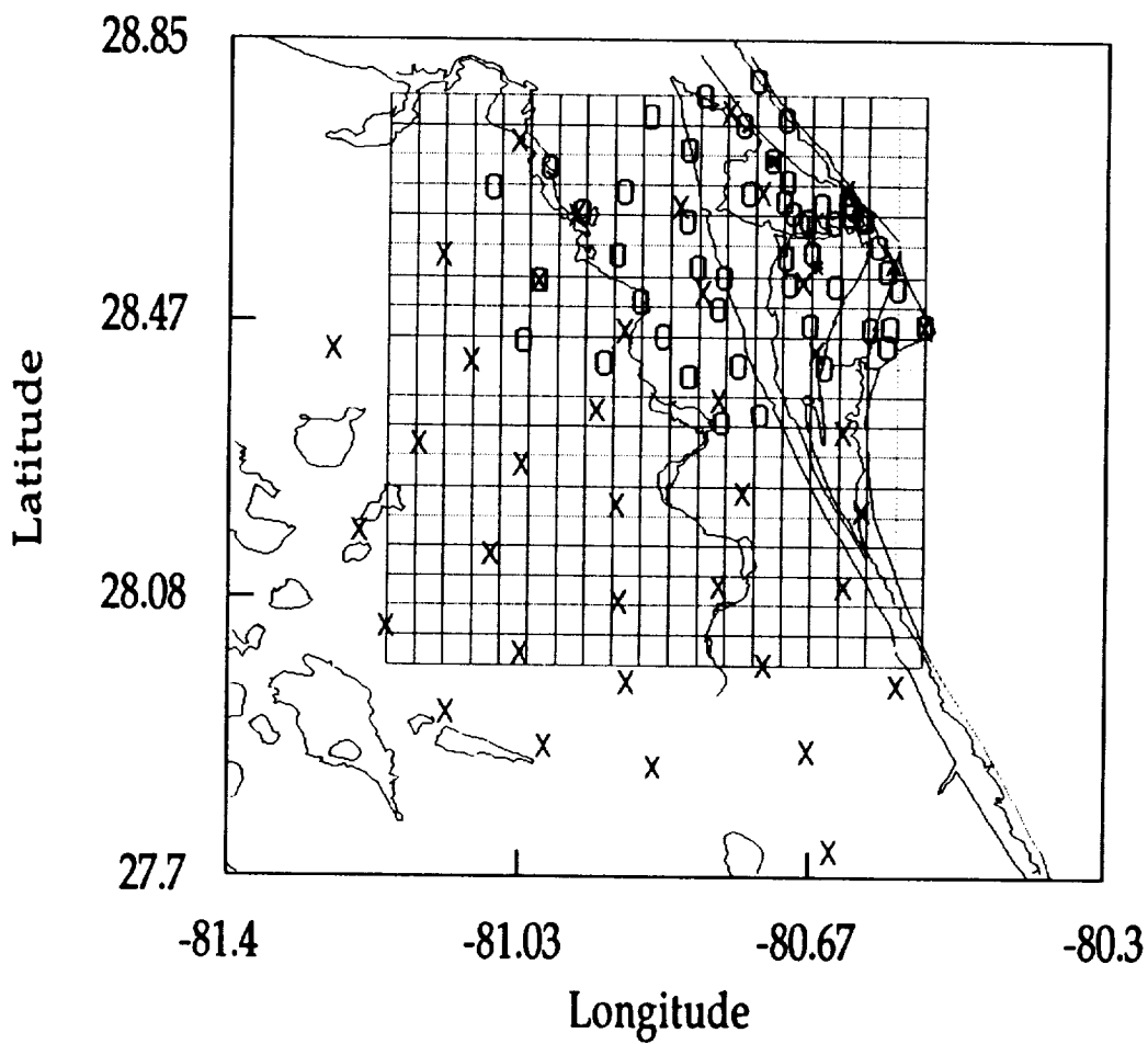
Figure 3: Similar to 2 but with the bivariate spatial interpolation grid overlaid on top of the area. X's are PAM stations, O's are KSC stations and * are the two FSU flux sites.
