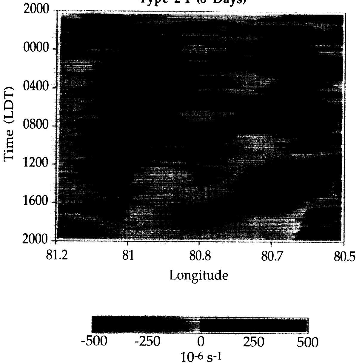
Figure 25b: Time-horizonal space cross sections of divergence over the CaPE study area diurnally averaged over all Type 2-I flow days (8 days). Red and yellow areas indicate negative divergence and blue and black areas represent positive divergence.
