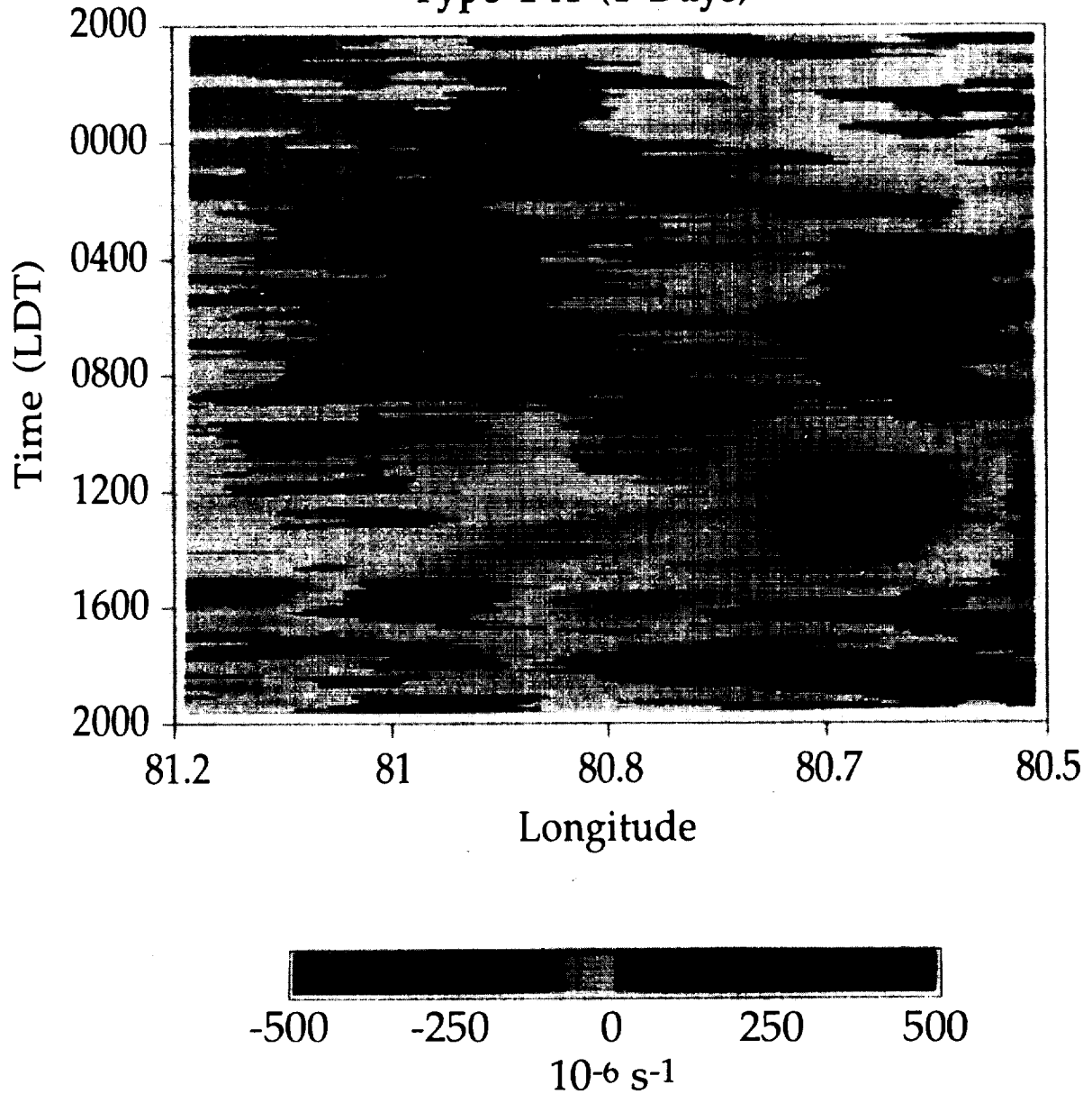
Figure 25c: Time-horizontal space cross sections of divergence over the CaPE study area diurnally averaged over all Type 1-A flow days (4 days). Red and yellow areas indicate negative divergence and blue and black areas represent positive divergence.
