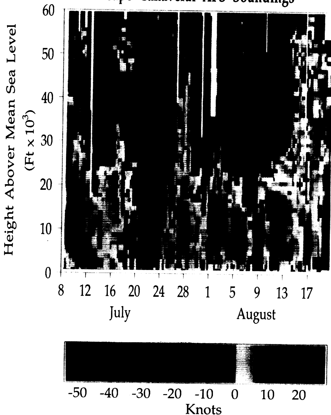
Figure 10: The 40-day time-height cross section of the u-component of wind as calculated from the CCAFS Soundings.
