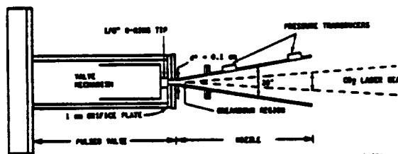
Figure 2. Diagram of pulsed valve-
