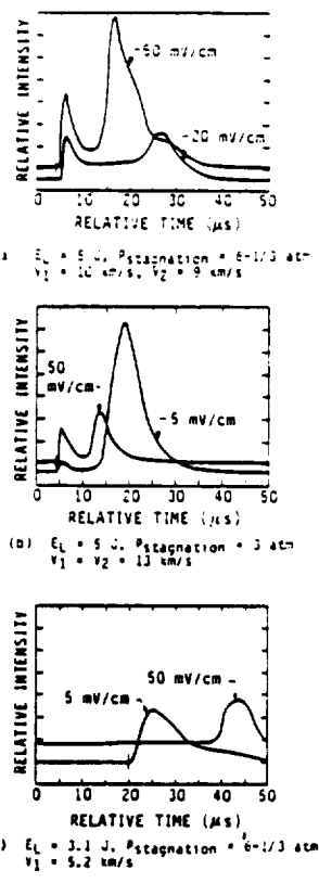
Fig. 4 777.3 nm radiometer histories (timescale is 5 μs per division).
