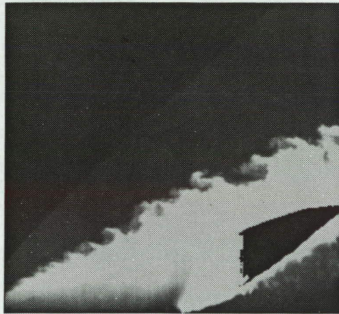
Figure 4.20. Instantaneous Rayleigh scattering image for straight case with water-seeded air fuel at twice matched pressure at side view.
