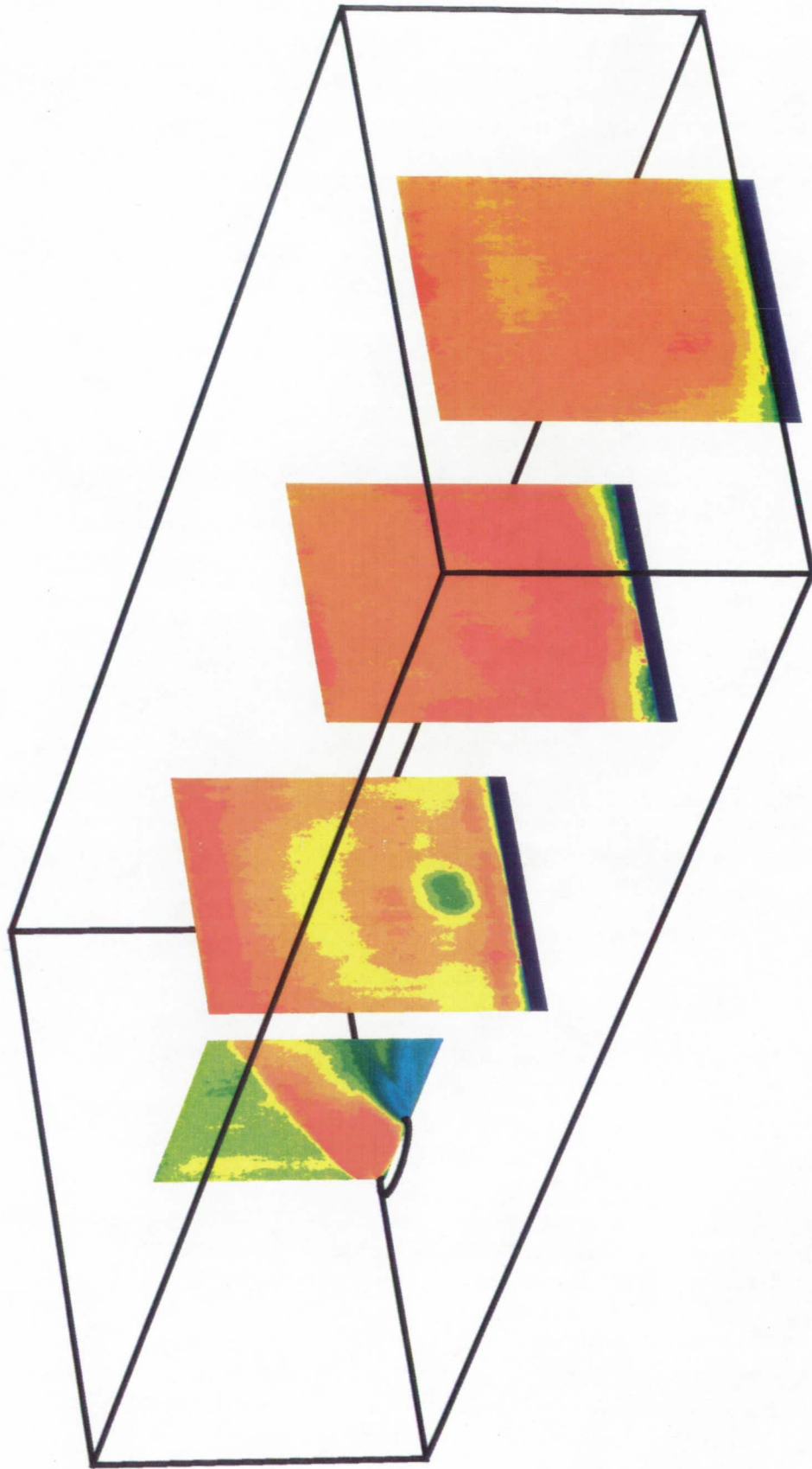
Figure 4.3. Composite view of average Rayleigh scattering images for straight case with air fuel.
