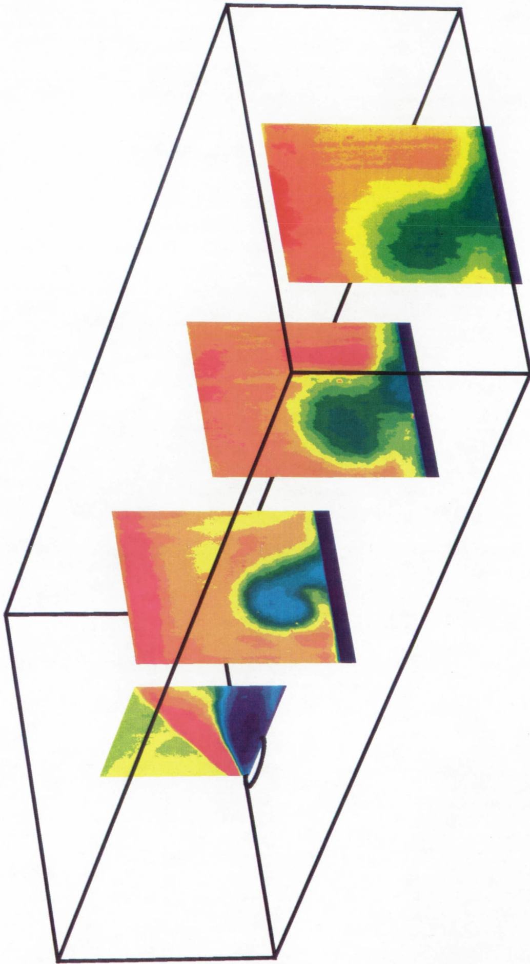
Figure 4.5. Composite view of average Rayleigh scattering images for low-swirl case with helium fuel.
