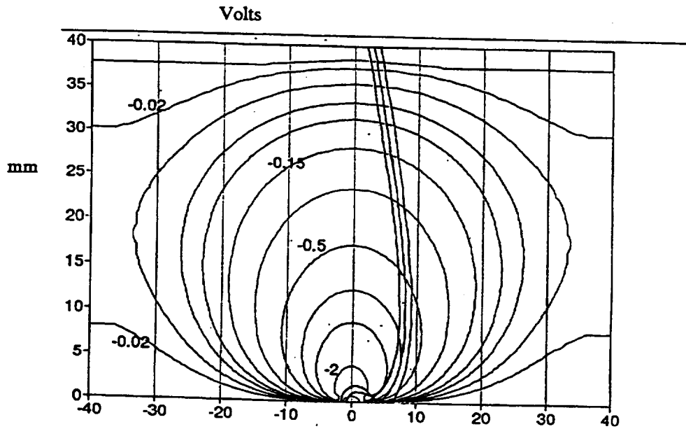
Figure 3. Equipotential contours and ion tracks above a 1 mm pinhole in a perfect insulator, underlying conductor biased to -140 V.
