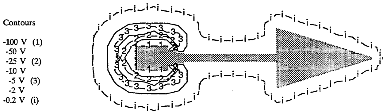
Figure 1. Equipotential contours around SP-100 payload (to left) and power system (right) computed with NASCAP/LEO.
