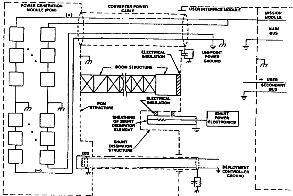
Figure 2. The grounding scheme utilized by SP-100, with the payload at right, and the power system at left. Notice the difference in grounding of the payload and power modules.
