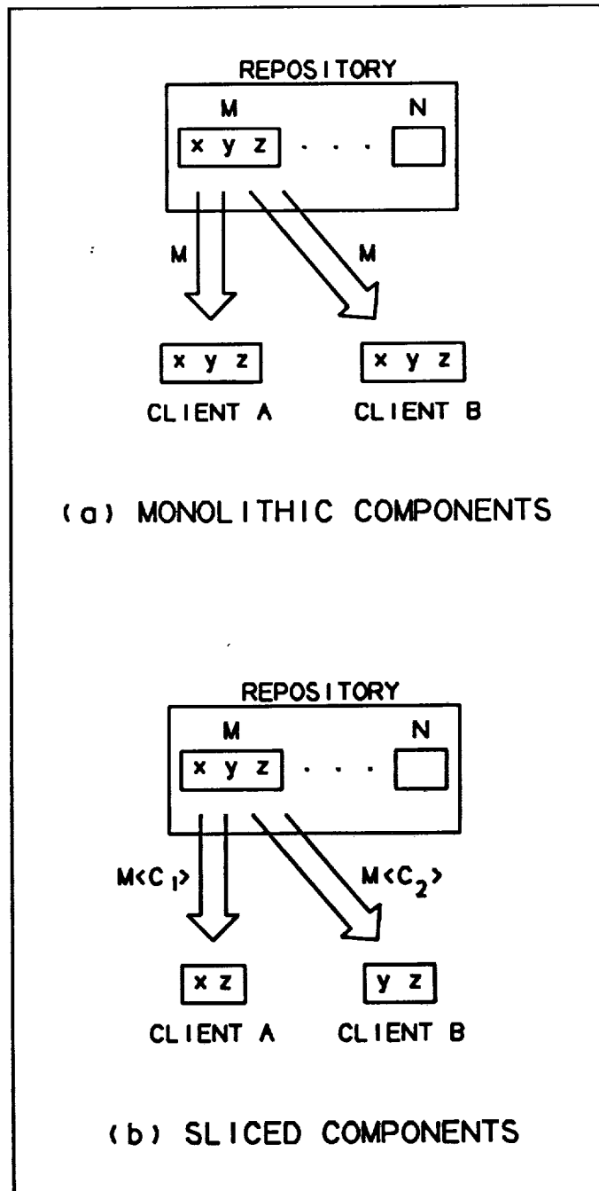
Figure 1 Clients of a repository component
