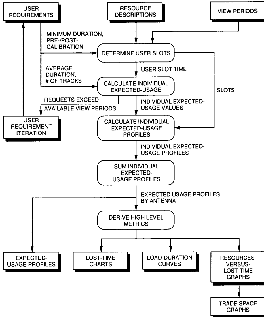
Fig. 8. PC4CAST forecasting engine process flow chart.
