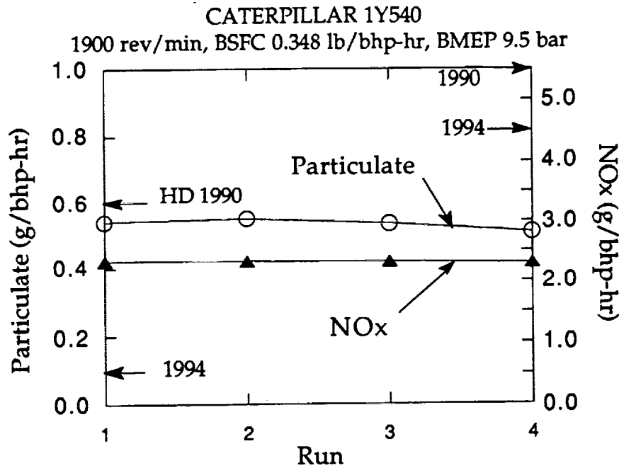
Fig. 20 Particulate and NOx measurements at 1900 rev/min showing repeatability of the emissions measurements for different runs.
