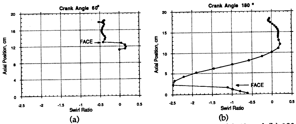
Fig. 14 Swirl ratio variation with depth below the head at (a) 60 and (b) 180 degrees ATDC. The arrow indicates the piston face. Non-zero swirl ratios below the face are in the piston bowl.
