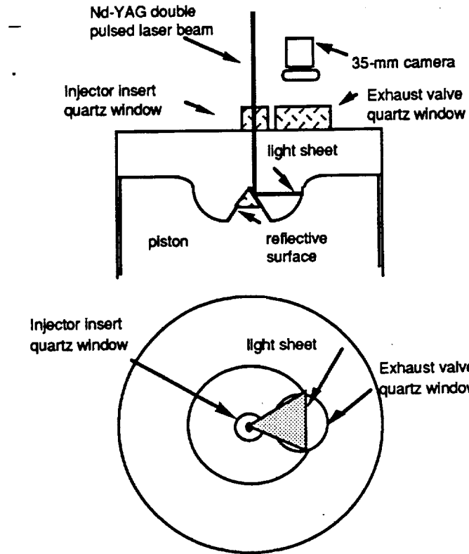
Fig. 27 Schematic diagram of optical layout for in-cylinder PIV.
