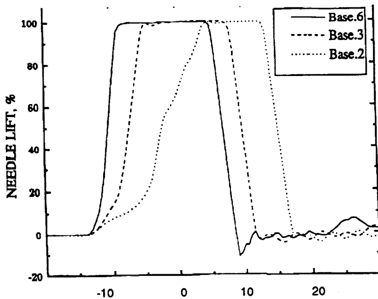
Fig. 22 Needle lift versus crank angle for Nippondenso U2 injector with three different check valve orifice diameters (0.6, 0.3 and 0.2 mm)
