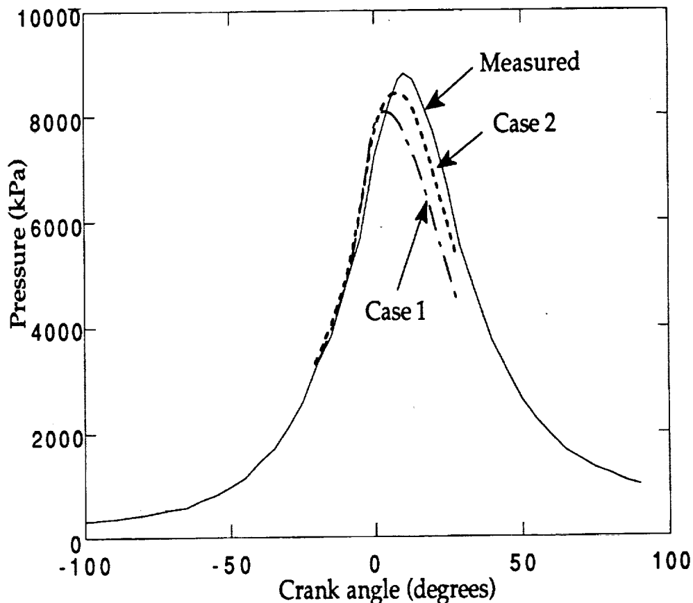
Fig. 6 Measured and predicted pressure histories with the standard one-step Arrhenius model (Case 1) and the multistep Shell ignition model (Case 2). Cummins engine at 1500 rev/min.
