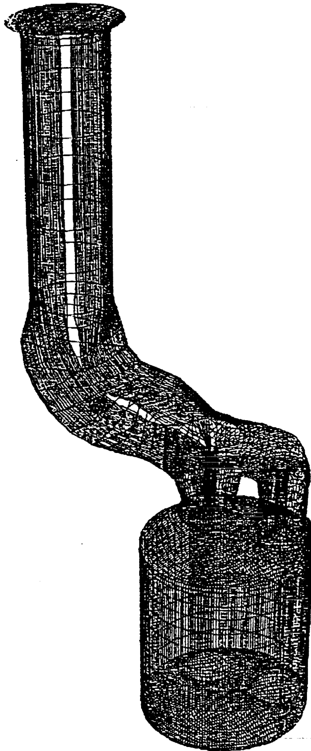
Fig. 10 Computational grid used for the two-intake valve Caterpillar engine. The bell-mouthed entrance to the intake manifold is at the intake surge tank.
