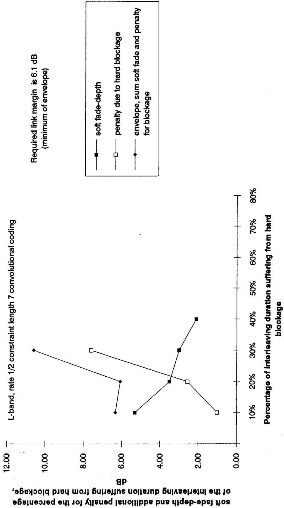
Figure 3 Soft fade-depth and additional penalty due to hard blockage for the typical example of heavy signal blockage
