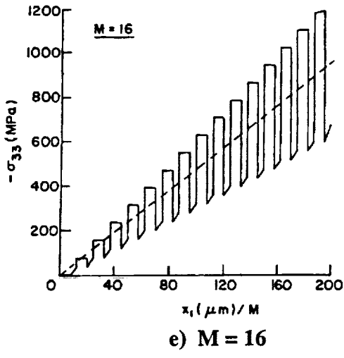
Figure 8 - Through-the-thickness normal stress \sigma_{33} in a unidirectional composite with uniformly spaced fibers in the cross-section containing both phases (—) FG theory, (- - -) continuum theory, (•—•) "primitive" micromechanics.
