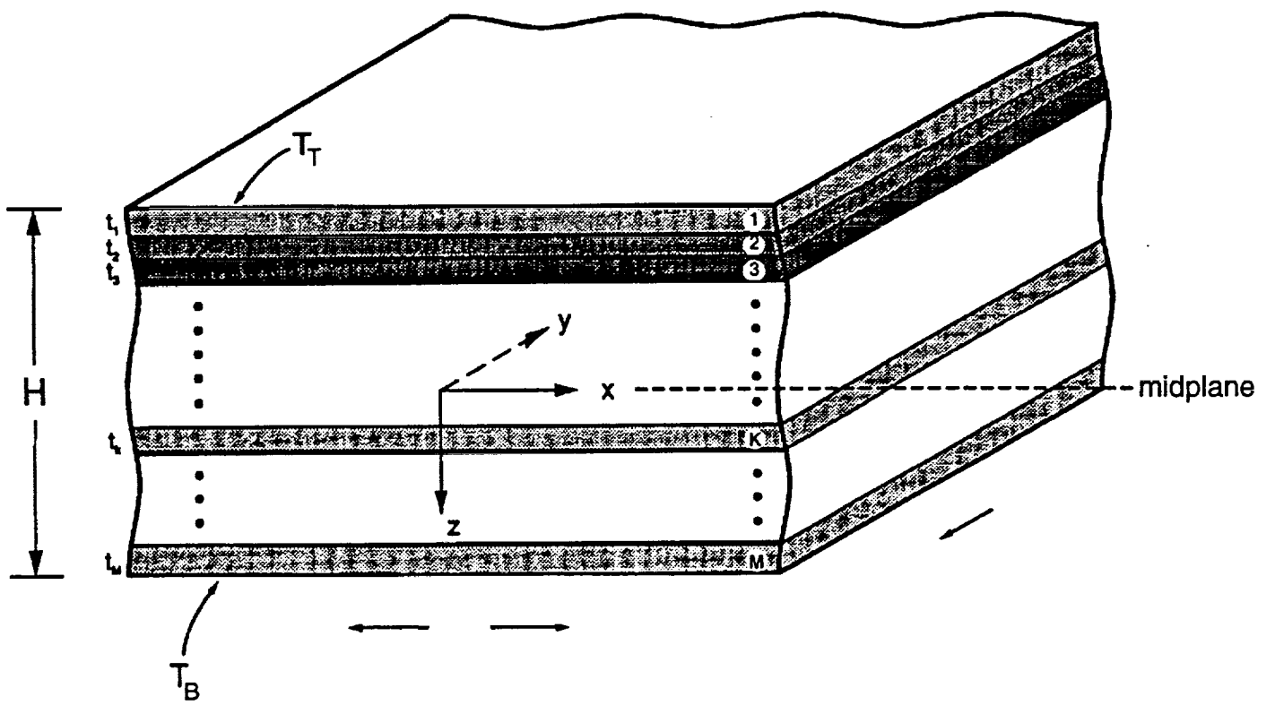
Figure 4 - Laminate geometry.
