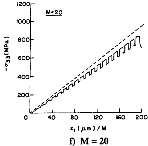
Figure 10 - Through-the-thickness normal stress \sigma_{33} in a unidirectional composite with uniformly spaced fibers in the cross-section matrix phase only (—) FG theory, (---) continuum theory, (•—•) "primitive" micromechanics.
