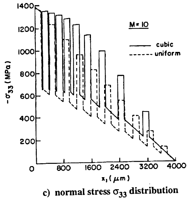
Figure 23 - Effect of reversing the direction of imposed thermal gradient in a unidirectional composite with cubically spaced fibers. Comparison with uniformly spaced fiber composite.
