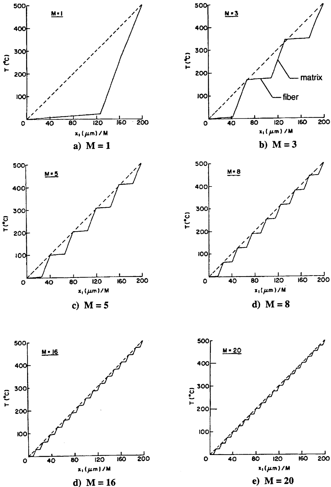
Figure 5 - Through-the-thickness temperature distribution in a unidirectional composite with uniformly spaced fibers in the cross-section containing both phases (—) FG theory, (---) continuum theory.
