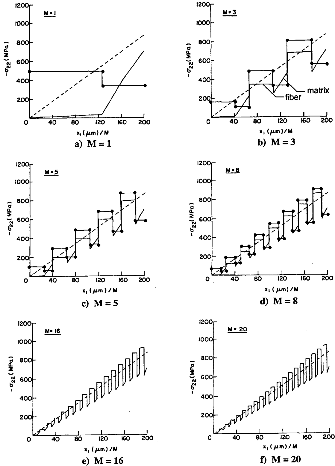
Figure 7 - Through-the-thickness normal stress \sigma_{22} in a unidirectional composite with uniformly spaced fibers in the cross-section containing both phases (—) FG theory, (---) continuum theory, (•—•) "primitive" micromechanics.
