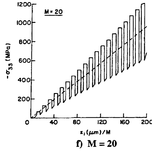
Figure 8 - Through-the-thickness normal stress \sigma_{33} in a unidirectional composite with uniformly spaced fibers in the cross-section containing both phases (—) FG theory, (- - -) continuum theory, (•—•) "primitive" micromechanics.
