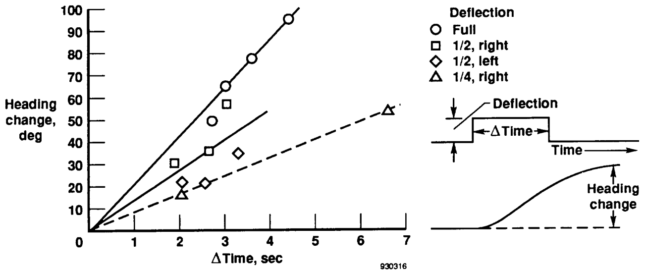
Figure 7. Control power as measured for flights 15 and 16.
