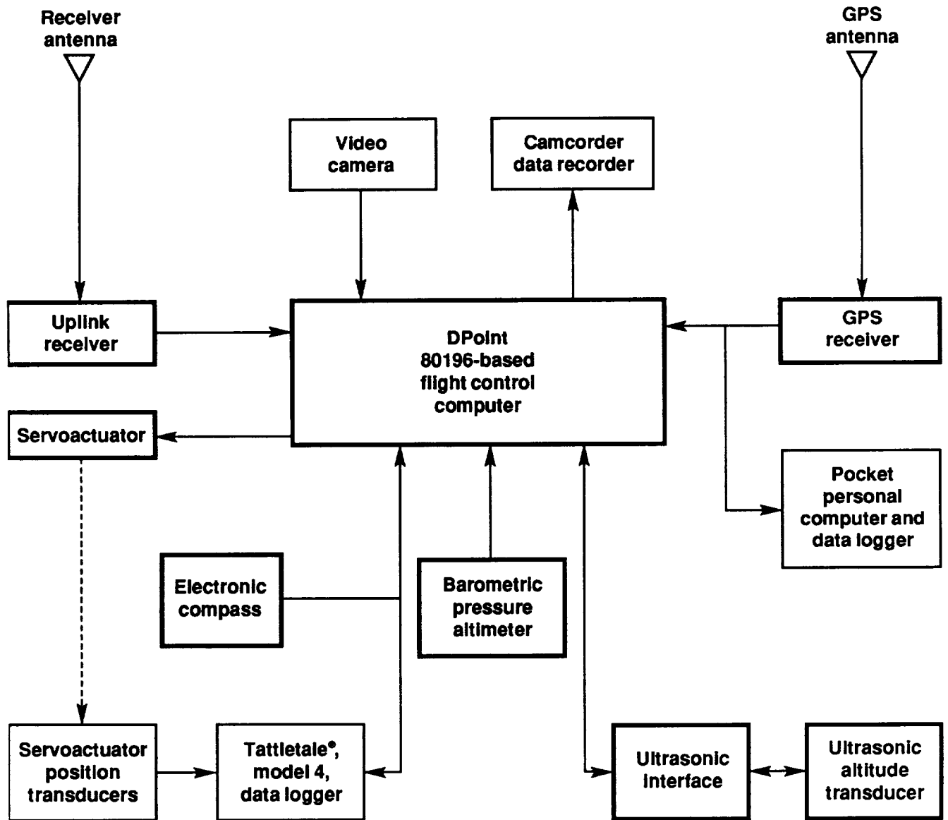
Figure 4. Phase 1 avionics.
