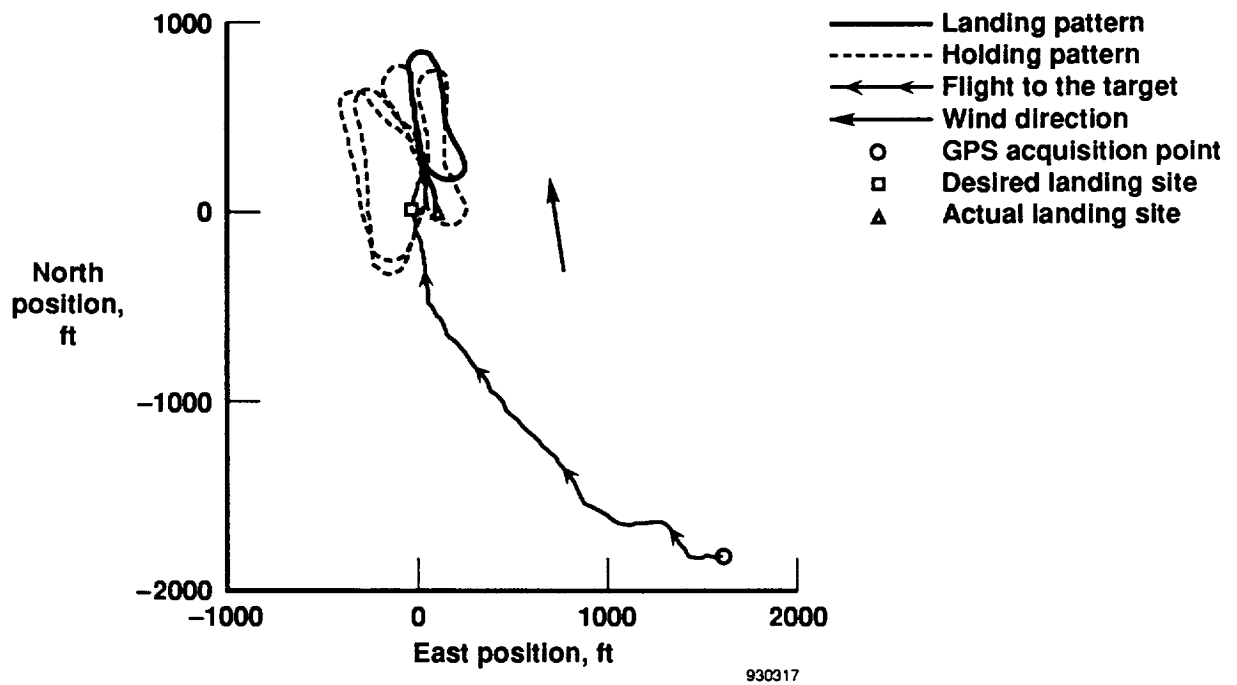
Figure 10. Ground track of flight 33 at an altitude of 6000 ft.
