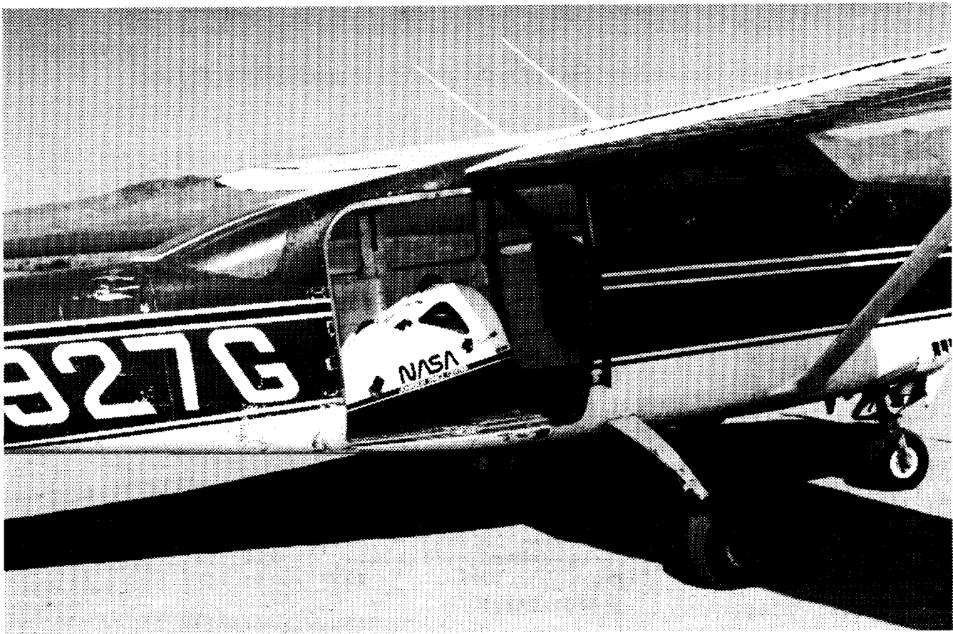
Figure 8. Spacewedge inside of the light airplane launch aircraft.
