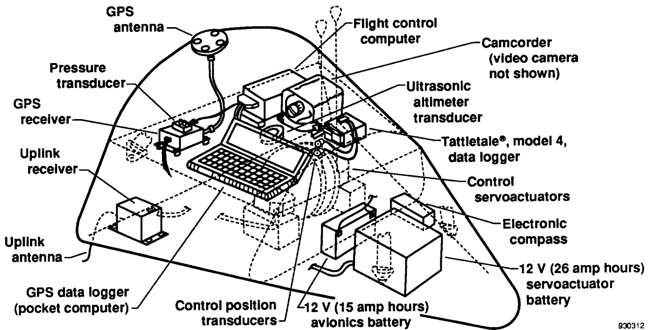
Figure 3. Cutaway drawing of Spacewedge vehicle.
