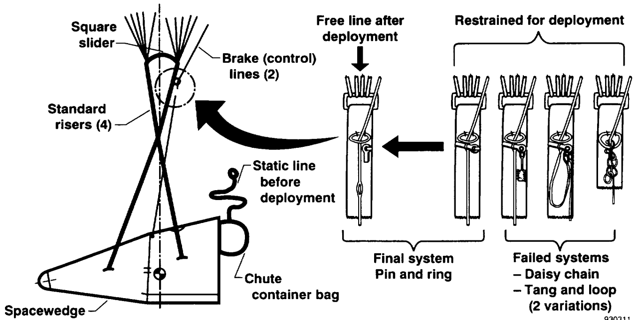
Figure 2. Brake line deployment restraint development.
