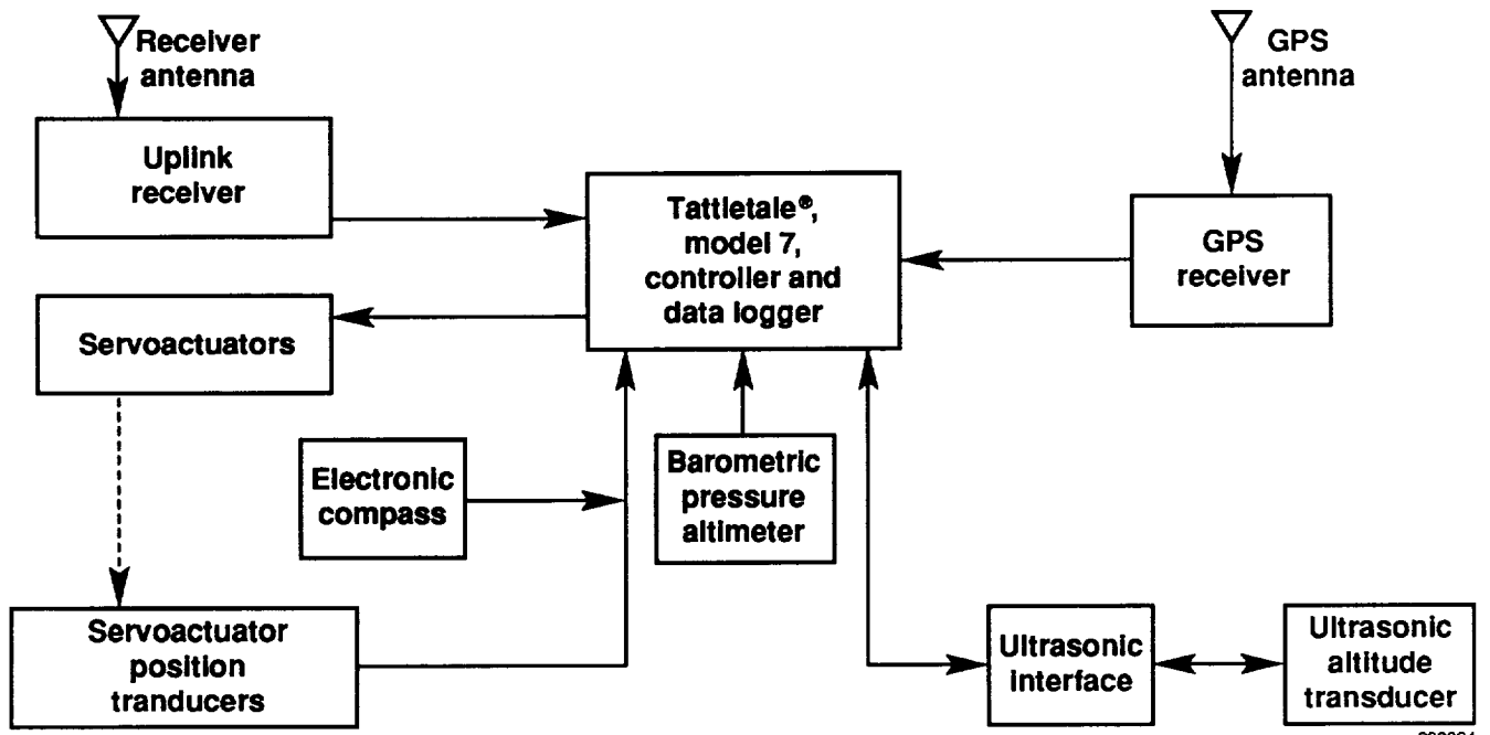
Figure 16. Phase 2 avionics.
