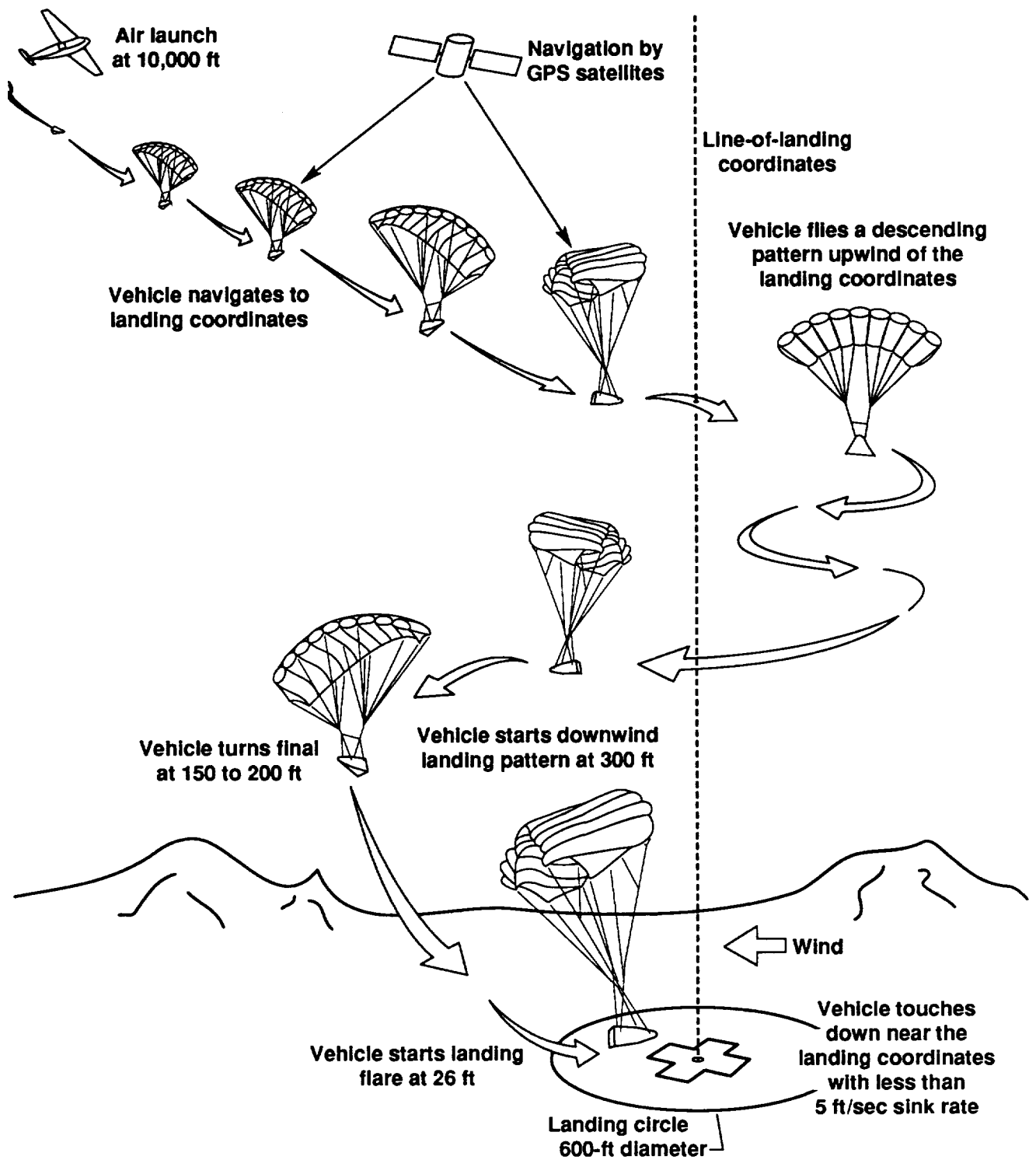
Figure 6. Autonomous mode control elements.
