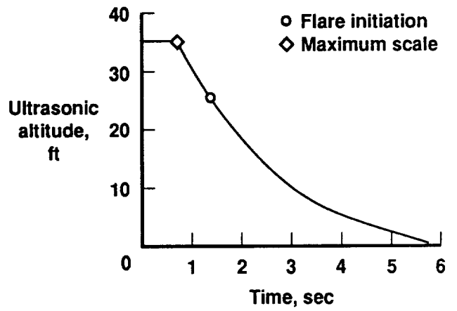
Figure 13. Landing flare control surface position and ultrasonic altitude for flight 35.
