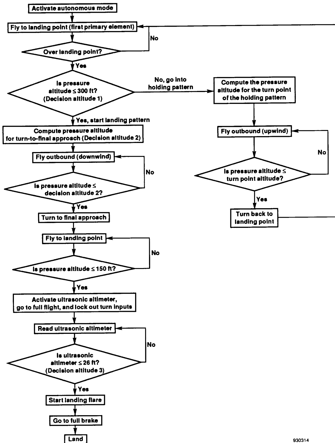
Figure 5. Conceptual autonomous mode logic.
