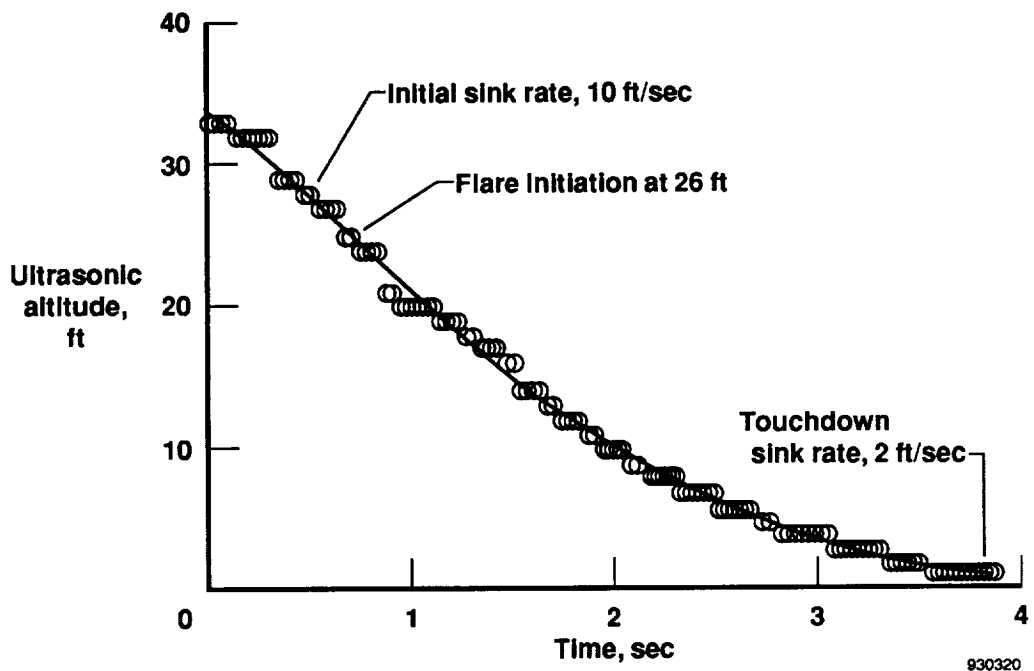
Figure 12. Landing flare for flight 28.
