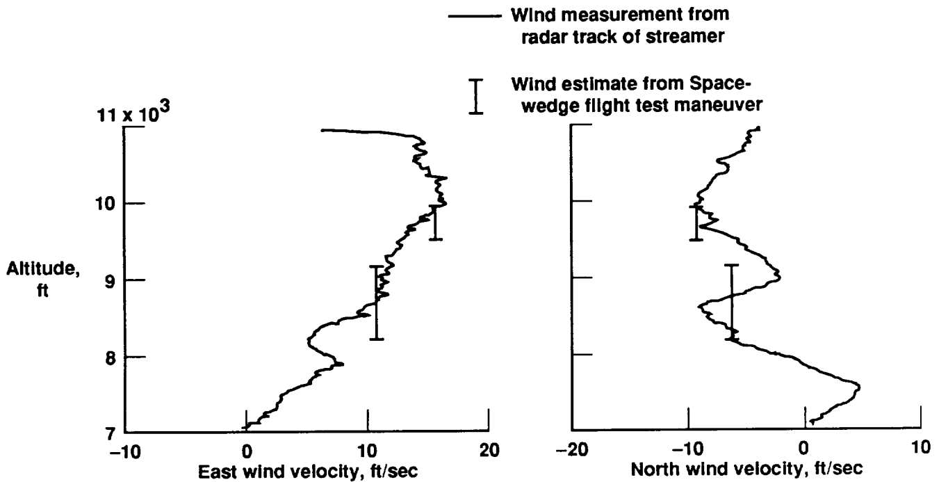
Figure 15. Comparison of the three-circle maneuver results with the radar data.
