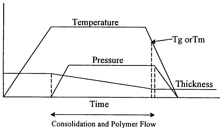
Figure 4. Towpreg Textile Preform Consolidation Cycle
