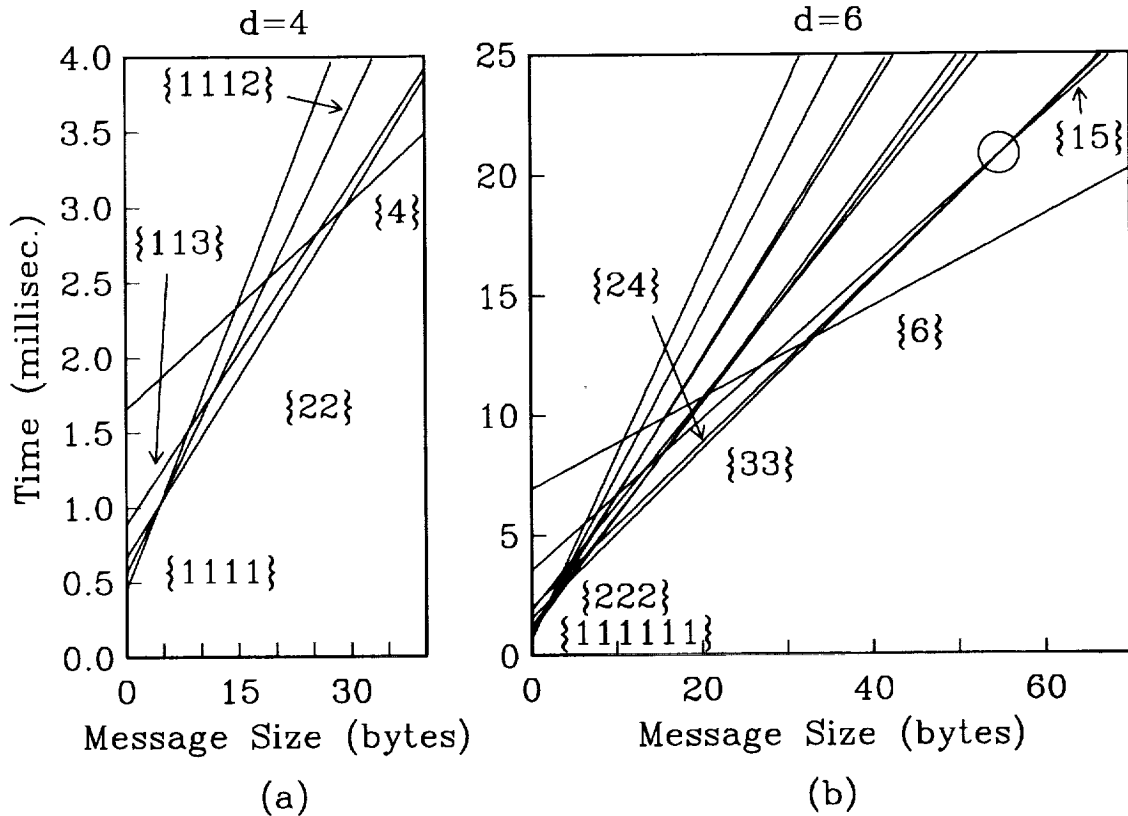
Figure 1: Run times for d = 4, 6 . In this particular example, \lambda = 100 , \delta = 10 ( \mu\text{sec.} ) and \tau = 2, \rho = 1 ( \mu\text{sec./byte} ). Circle indicates the point of intersection of all partitions of cardinality 2: {33}, {24} and {15}
