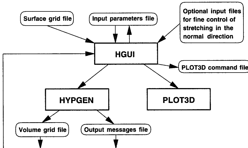
Figure 1.1. Overview of input and output files for running HYPGEN in batch mode.
