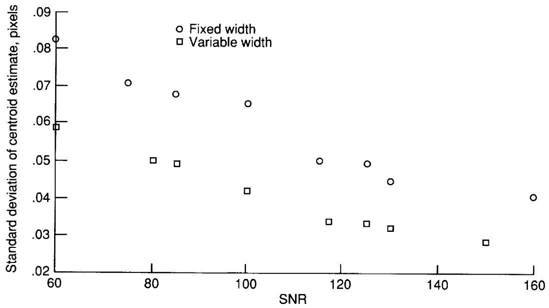
Figure 21. Standard deviation of centroid estimate versus SNR for uniform window of variable width and fixed width of N = 14 .
