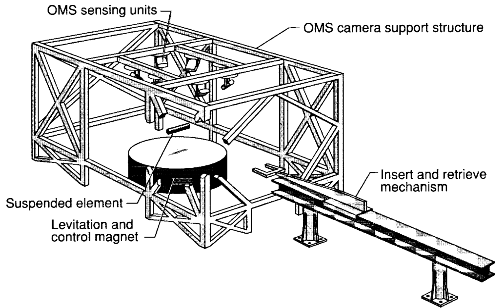
Figure 1. Optical measurement system (OMS) of large gap magnetic suspension system (LGMSS).
