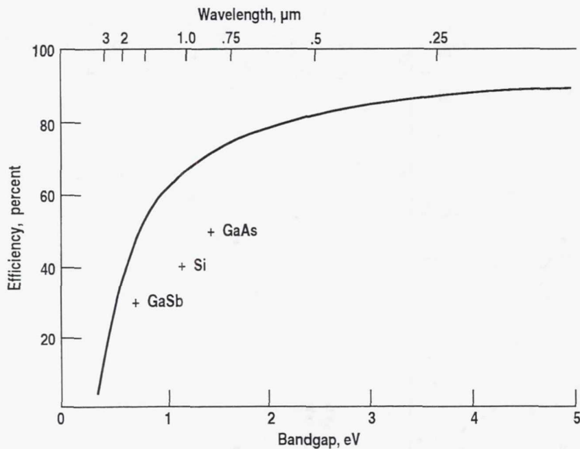
Figure 5.—Theoretical conversion efficiency of photovoltaic cells for monochromatic light. Intensity, 500 \text{ mW/cm}^2 ; temperature, 25^\circ \text{C} .
