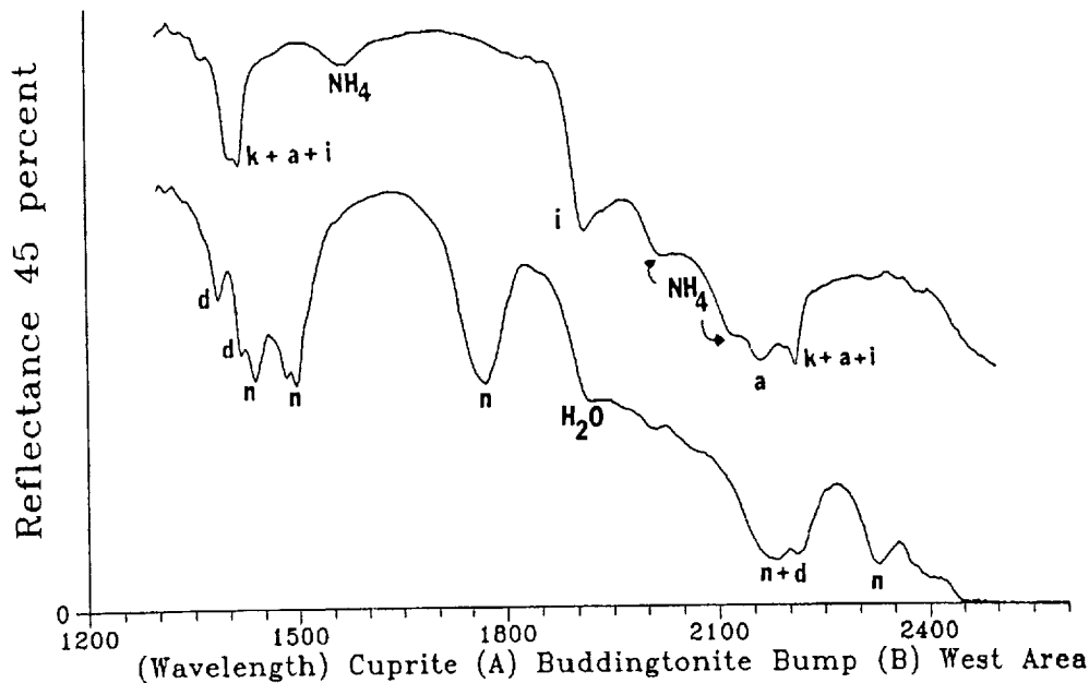
Fig. 2. PIMA-II Spectra from Cuprite, NV. (A) is from the Buddingtonite Bump; (B) from the Alteration Zone West of U.S. Highway 95. Key for the Minerals in the Spectra: K = Kaolinite, A = Alunite, N = natro-alunite, D = dickite, I = Illite. Spectra Collected with the PIMA-II Portable Short Wave Infrared (SWIR) Spectrometer, Integrated Spectronics, Pty Ltd., Sydney, Australia.
