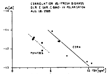
Fig. 2 Correlations of \sigma_{na} (derived from the mean grey value per field) with the fresh biomass of corn and potatoes (C-band image, Aug. 1989).
