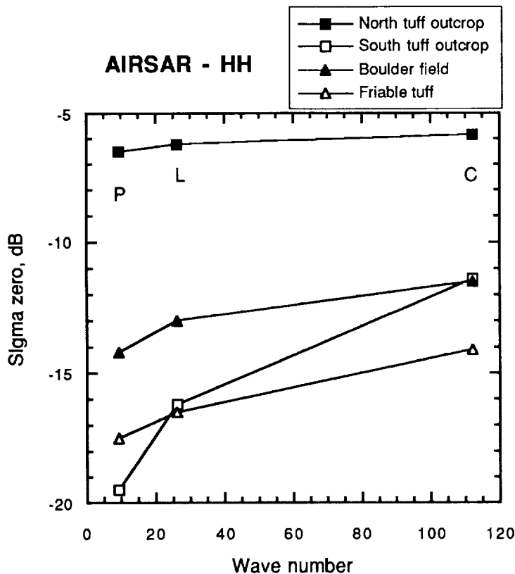
Figure 2. AIRSAR HH polarization backscatter cross section ( \sigma_0 ) as a function of wave number ( 2\pi/\lambda ). Corresponding wavelengths are: P-band 68 cm, L-band 24 cm, C-band 5.6 cm. Flat spectrum of north tuff indicates topographic control. Steep spectrum of south tuff indicates low "power" at larger scales of surface roughness.
