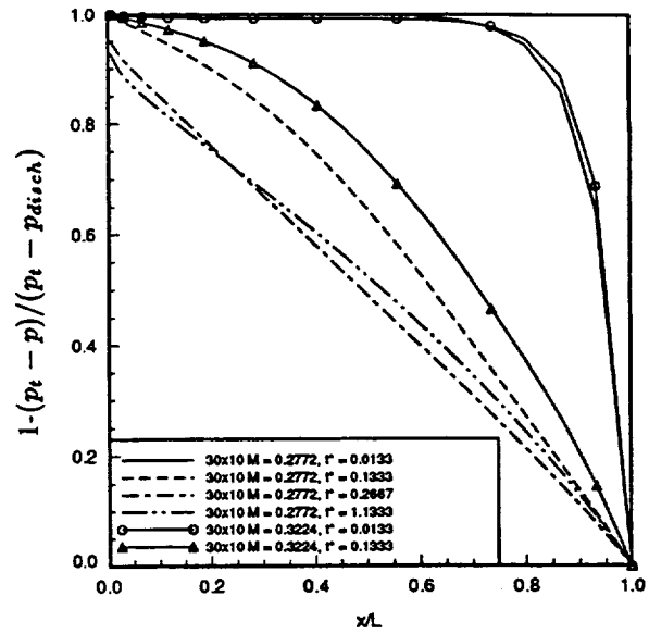
Figure 13: Predicted distribution of centerline pressure along pipe at early times, E=0.108 .
