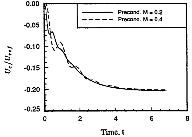
Figure 3: Time history of predicted u component of velocity at cavity center, Re=100, impulsively started cavity.
