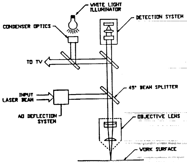
Fig. 19. Direct write laser microlithography from NEOS Corporation.
