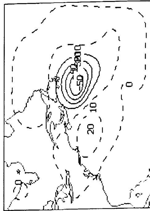
OMEP TIME 0, DRY 8501Z0, 400, MB
