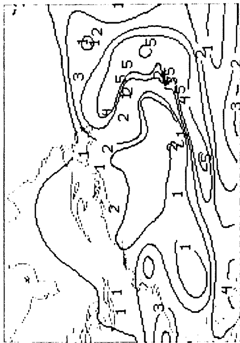
MIXR (BPK6) TIME 12. DRY 690120. 700. MB 24H FORECAST
