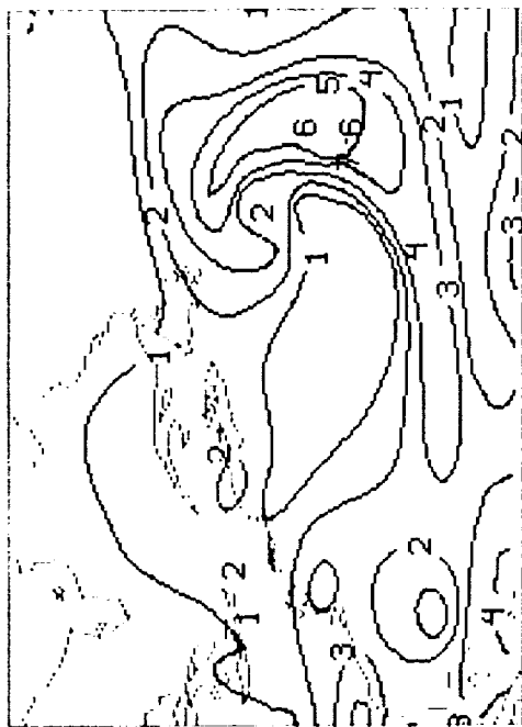
MIXR (BPK6) TIME 12. DRY 690120. 700. MB 12H FORECAST COLD
