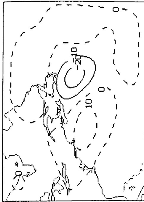
OMEP TIME 0, DRY 8501Z0, 400, MB
