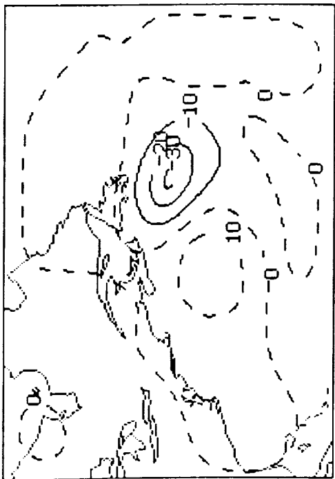
OMEP TIME 0, DRY 8501Z0, 700, MB
