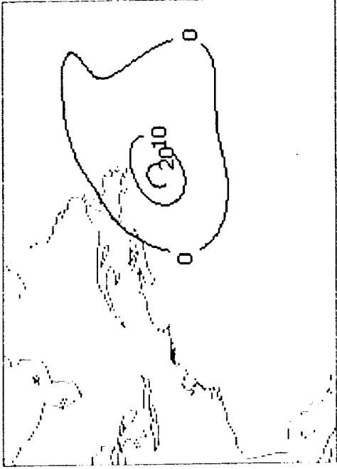
PFTN (MM) TIME 12. DRY 850120. EXTERNALLY FORCED 12H
