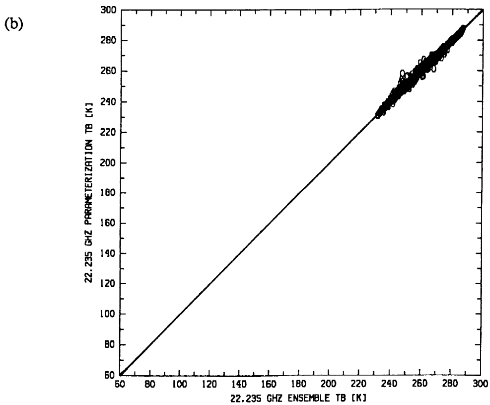
Fig. 11. Plot of parameterized brightness temperatures vs. cloud ensemble/radiative model brightness temperatures at (a) 19.35 GHz and (b) 22.235 GHz. For reference, the solid line in each panel represents a perfect correlation.
