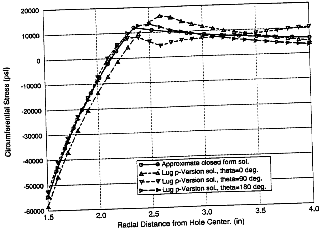
Figure 13: Cold-worked attachment lug. "Circumferential" stresses after unloading for various locations. Comparison with analytical solution of cold-worked tube.
