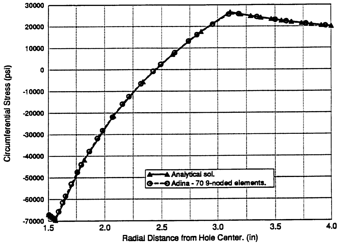
Figure 5: Circumferential stress in pressurized tube, loading case. Results of h-version FEM analysis with 9-noded elements.
