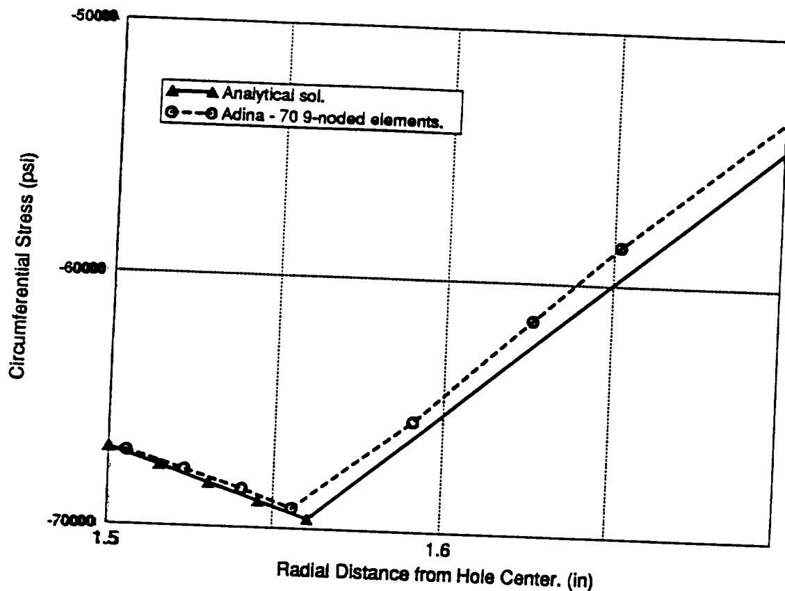
Figure 10: Circumferential stress in pressurized tube. Residual stress after cold-working. Results of h-version FEM analysis with 9-noded elements and exact solution. Zoom of zone of compressive plastification.
