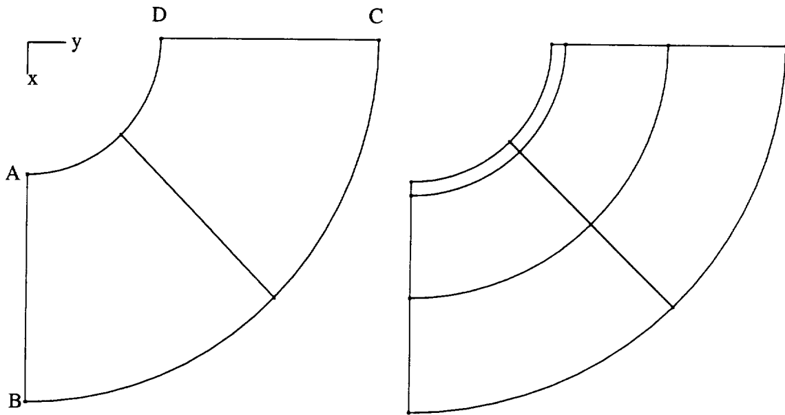
Figure 1: Meshes used in the p-version analysis of the tube under internal pressure.
