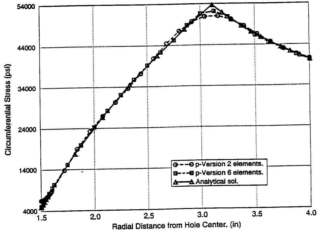
Figure 3: Circumferential stress in pressurized tube, loading case. Results of p-version FEM analysis and exact solution.
