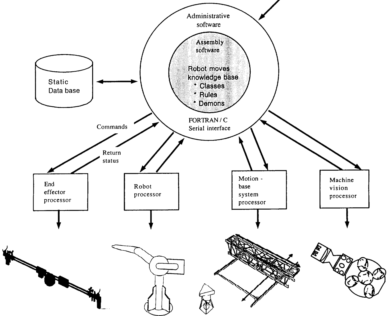
Figure 6. ASAL software architecture.
