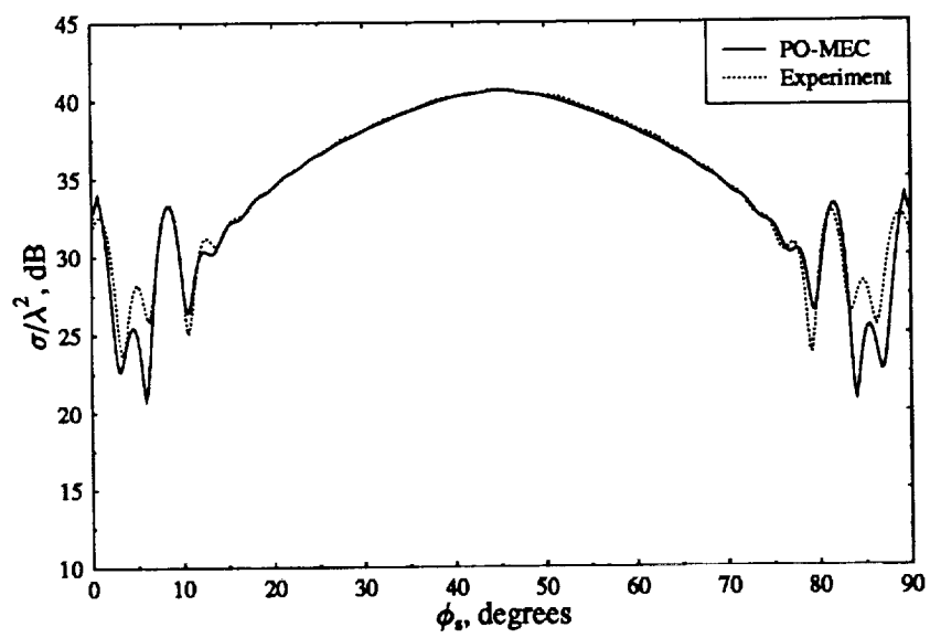
Figure 27: Monostatic RCS of a 10\lambda triangular trihedral on a great circle at \theta_g = 80^\circ .
