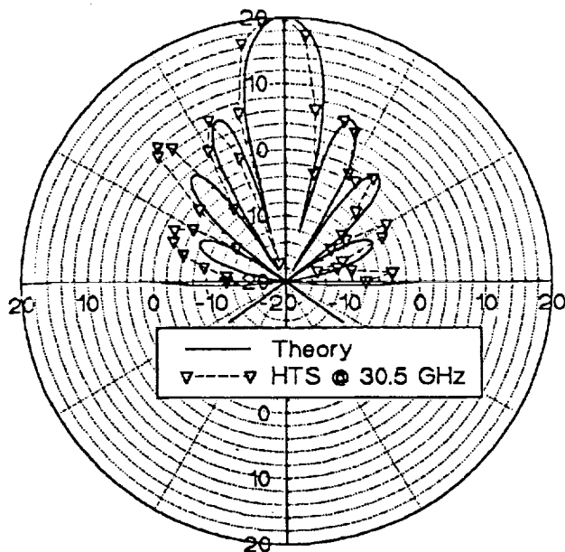
Fig. 5 H-plane radiation pattern, normalized to 20 dB.
