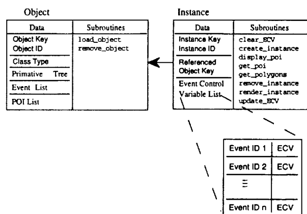
Fig. 1. 3D-EDGE Data Hierarchy Diagram
