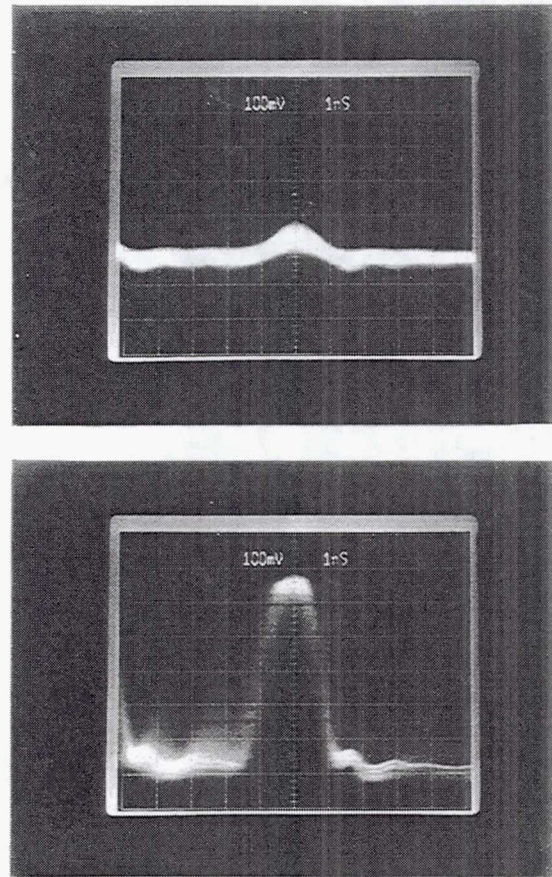
Figure 7.--Analog signal conditioning waveforms: (top) input signal, (bottom) amplified matched filter output.
