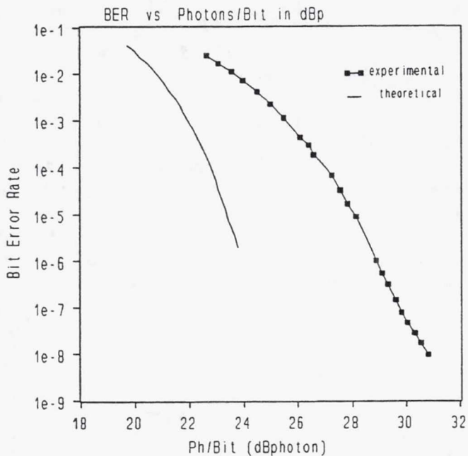
Figure 16.--Optical STE configuration results comparing theory to experimental data on a dB scale relative to one photon.
