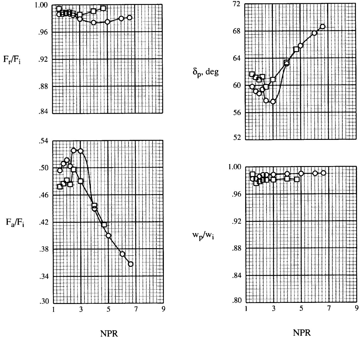
Figure 11. Resultant thrust ratio, thrust-vector angle, axial thrust ratio, and discharge coefficient as functions of nozzle pressure ratio. \delta_v = 60^\circ .
