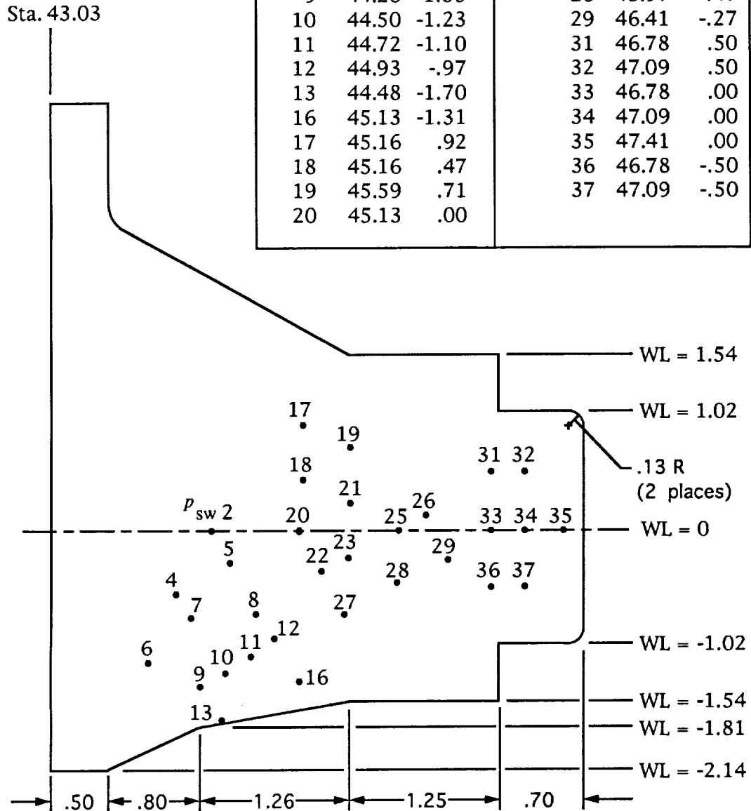
Figure 6. Sidewall dimensions and pressure orifice locations on right sidewall. All linear dimensions are in inches.
