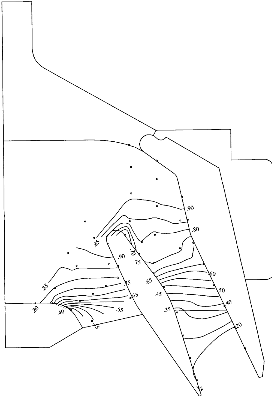
(b) Max 60° configuration. NPR = 3.0.
