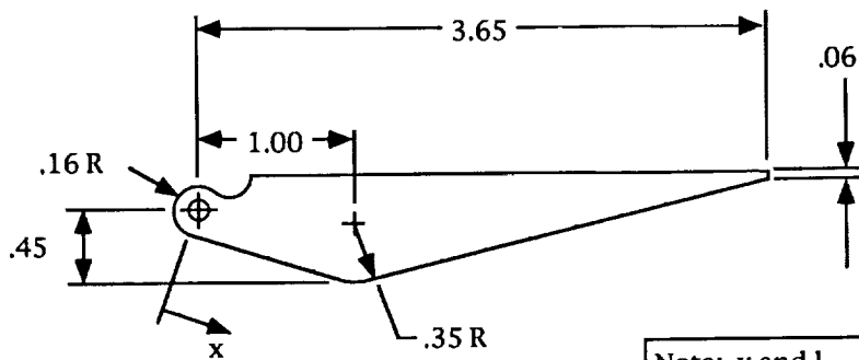
(a) Unvectored upper flaps. \delta_v = 0^\circ .
