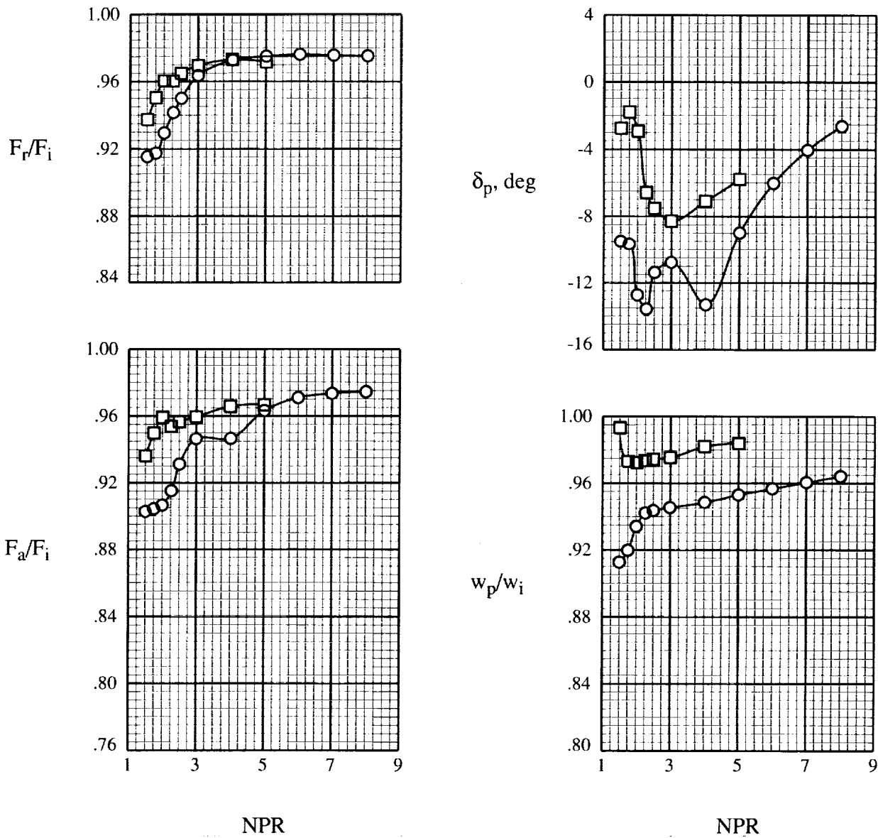
Figure 7. Resultant thrust ratio, thrust-vector angle, axial thrust ratio, and discharge coefficient as functions of nozzle pressure ratio. \delta_v = 0^\circ .
