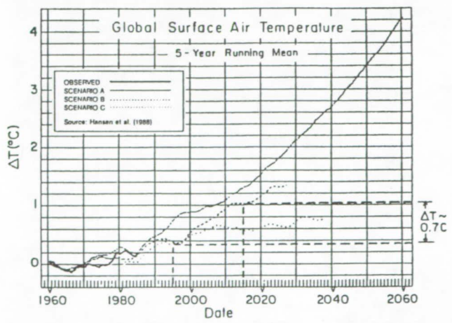
Fig. 3.1. Simulated global temperature change in climate simulations of Hansen et al. (1988). Rate of warming in the most realistic scenario (B), about 0.3°C/decade, is typical of other GCM and IPCC (1992) estimates.
