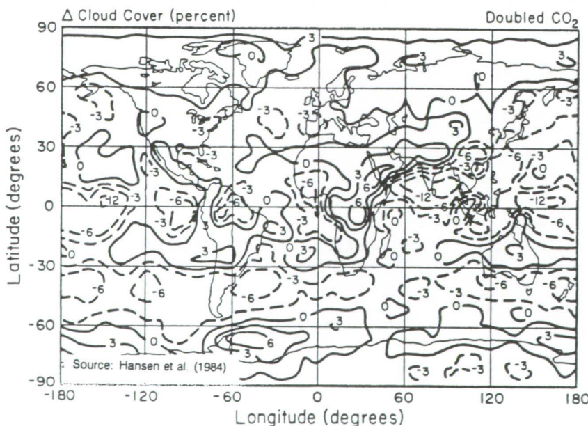
Fig. 3.6. Cloud cover changes in a doubled \text{CO}_2 experiment with the GISS GCM (Hansen et al. , 1984).
