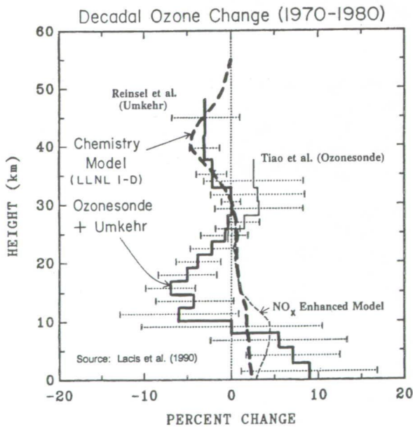
Fig. 2.4. Ozone changes predicted on the basis of homogeneous chemistry and ozone changes measured in the 1970s (figure reproduced from Lacis et al. , 1990).
