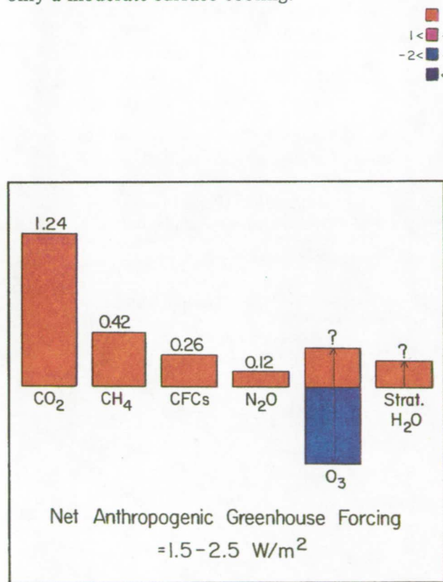
Fig. 2.2. Anthropogenic greenhouse climate forcings ( \text{W/m}^2 ) due to measured or estimated trace gas changes between 1850 and 1990. The forcing is calculated as the change in net radiative flux at the tropopause caused by the change in atmospheric composition.
