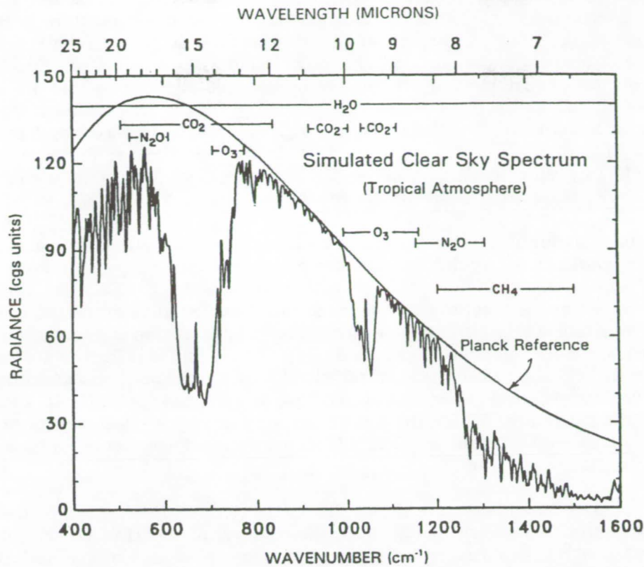
Fig. 10.1. Clear sky spectrum at 3 \text{ cm}^{-1} (IRIS) resolution. The spectral locations of the principal absorption features are identified.
