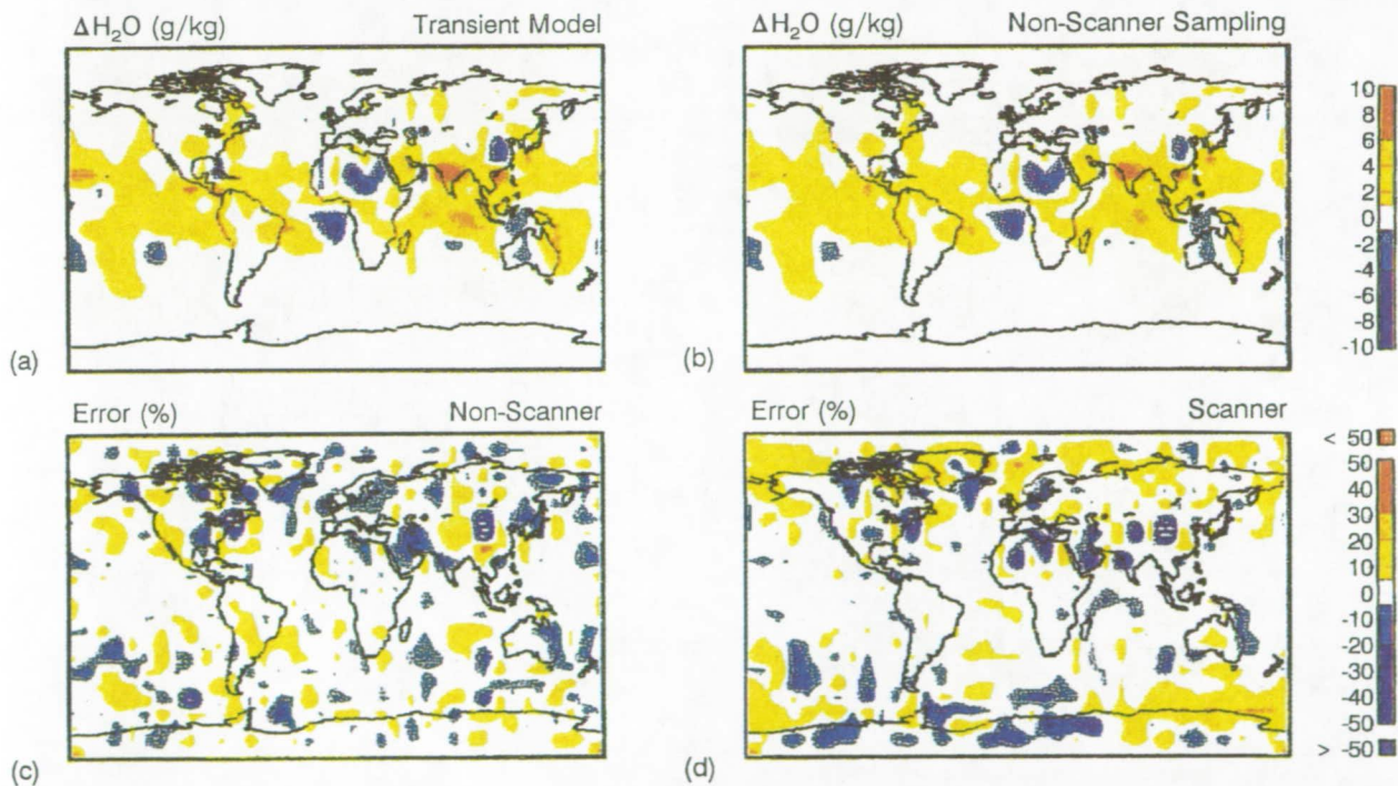
Fig. 12.9. Model-predicted changes (a) in specific humidity ( \text{g/kg} ) in the upper troposphere and measured changes (b) with Climsat non-scanning sampling. Errors are shown (in percent) for non-scanning sampling (c) and scanning sampling (d).
