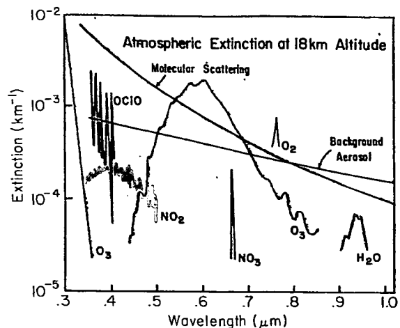
Fig. 8.2. Extinction contributions from different atmospheric constituents at 18 km altitude. On SAGE III a CCD linear array will provide 1 nm resolution from 0.29 μm to 1.02 μm, with an additional channel at 1.55 μm.
