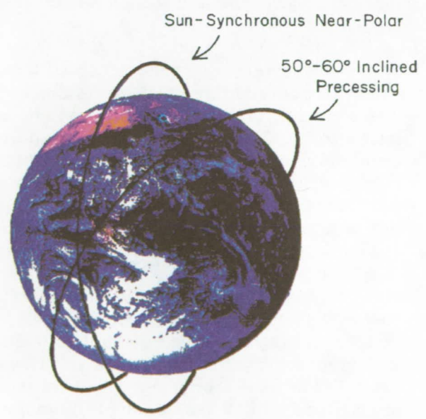
Fig. 12.1. Required satellite orbits for the Climsat observing system.
