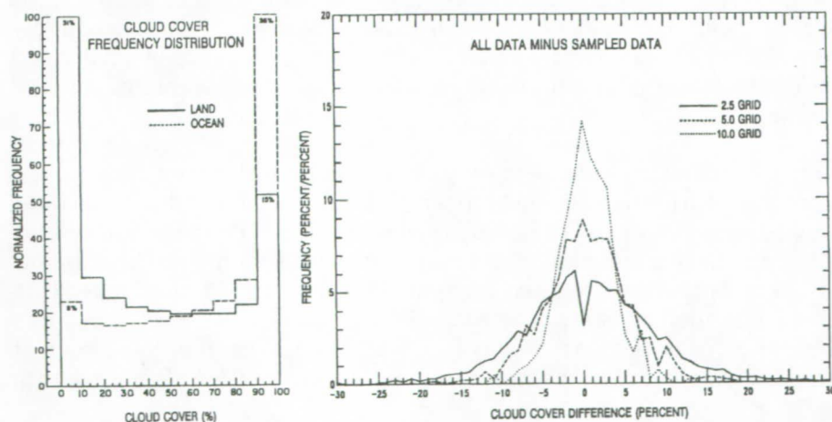
Fig. 12.5. Cloud cover frequency distribution for land and ocean and distribution of differences in monthly regional mean values produced by non-scanning sampling from Climatsat orbits.
