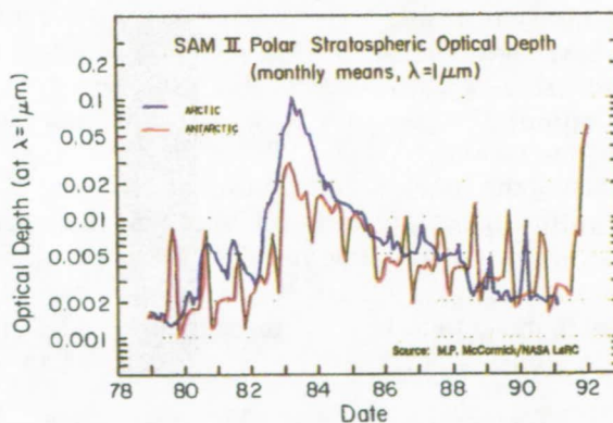
Fig. 2.7. Stratospheric aerosol optical depth at 1 \mu\text{m} wavelength in the polar regions measured by a solar occultation instrument on the Nimbus-7 spacecraft (M.P. McCormick, private communication).
