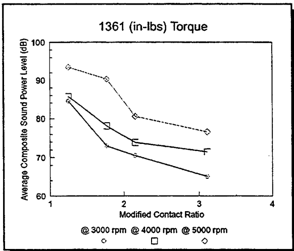
Figure 19 - Modified Contact Ratio Effect
