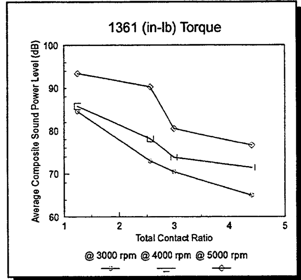
Figure 20 - Total Contact Ratio Effect
