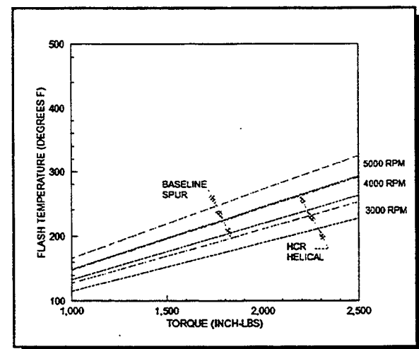
Figure 9 - Flash Temperature v Torque
