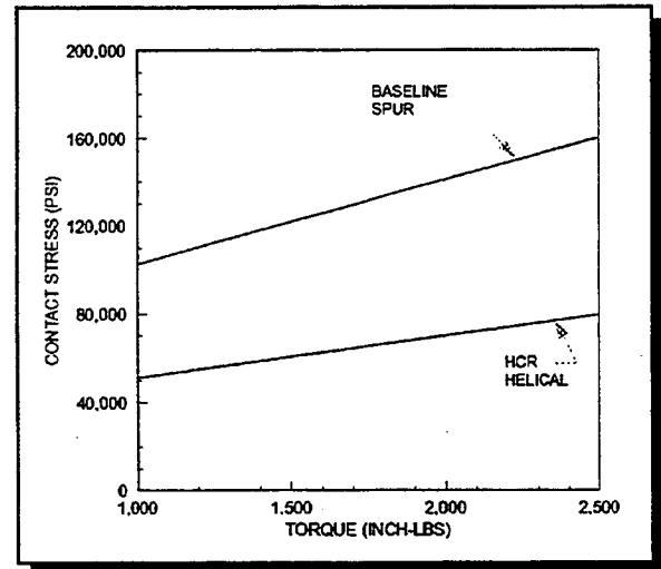
Figure 8 - Contact Stress v Torque
