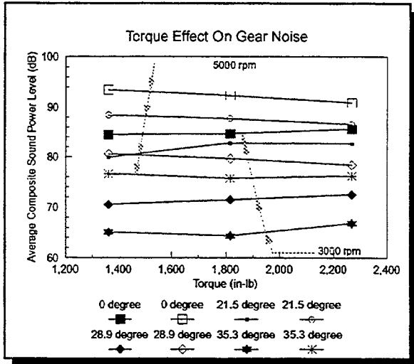
Figure 15 - Torque Effect On Gear Noise
