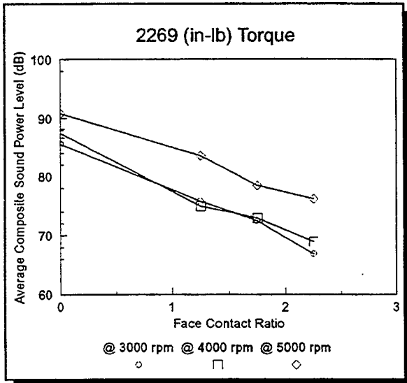
Figure 18 - Face Contact Ratio Effect High Torque
