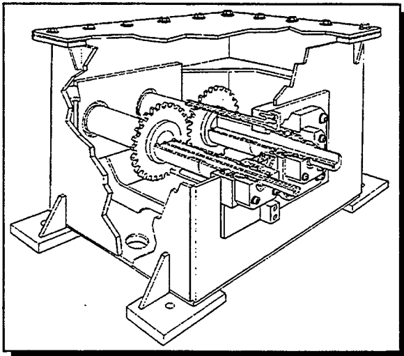
Figure 3 - Test Gear Box Cutaway Section
