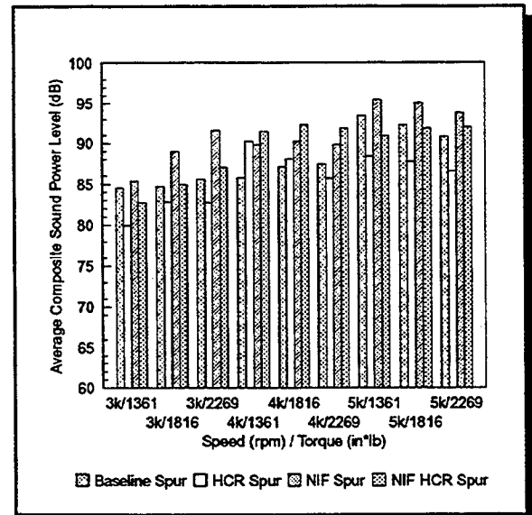
Figure 21 - Tooth Form Effect
