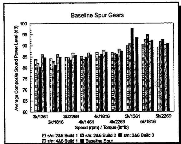
Figure 13 - Spur Gear Build Variations
