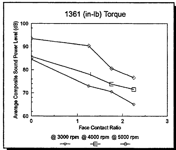
Figure 17 - Face Contact Ratio Effect Low Torque
