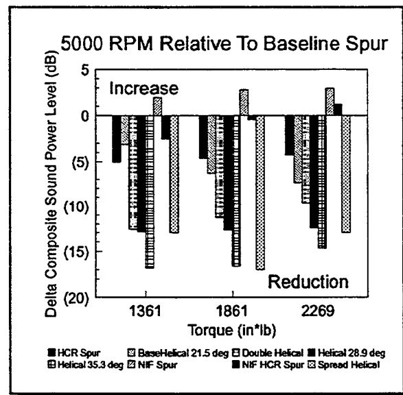
Figure 24 - 5,000 RPM Noise Summary
