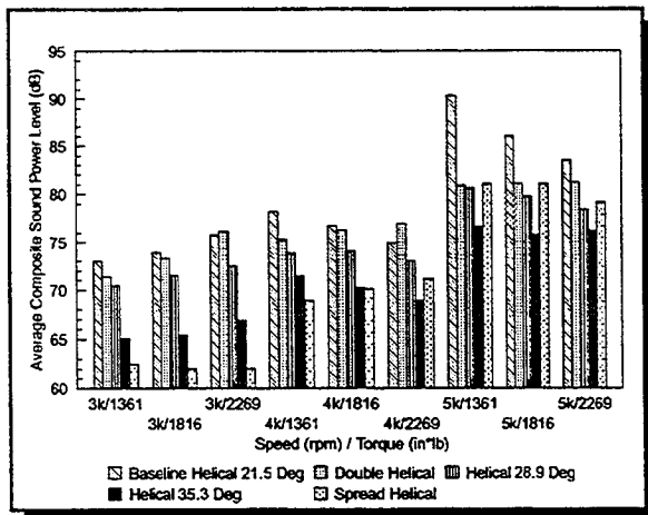
Figure 12 - Helical Gear Noise Levels
