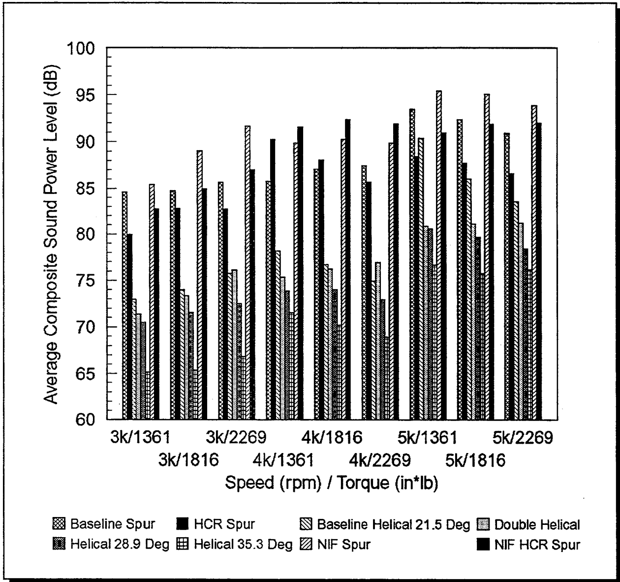
Figure 10 - Summary Of Test Results
