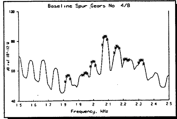
Figure 6 - Enlargement of Figure 5 (Around First Harmonic)
