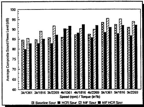
Figure 11 - Spur Gear Noise Levels
