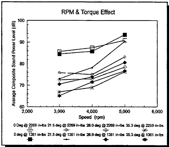
Figure 16 - Combined Speed & Torque Effects
