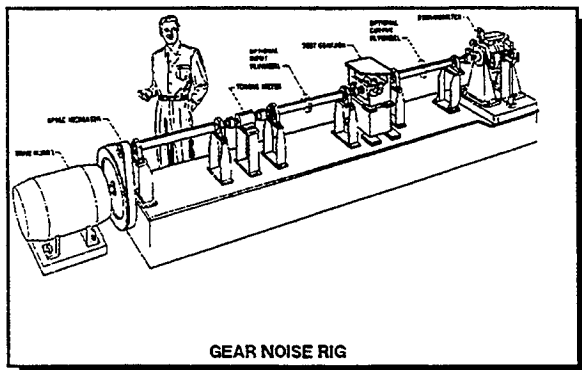
Figure 2 - Nasa Gear Test Rig
