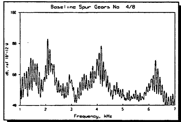
Figure 5 - Baseline Spur Spectrum
