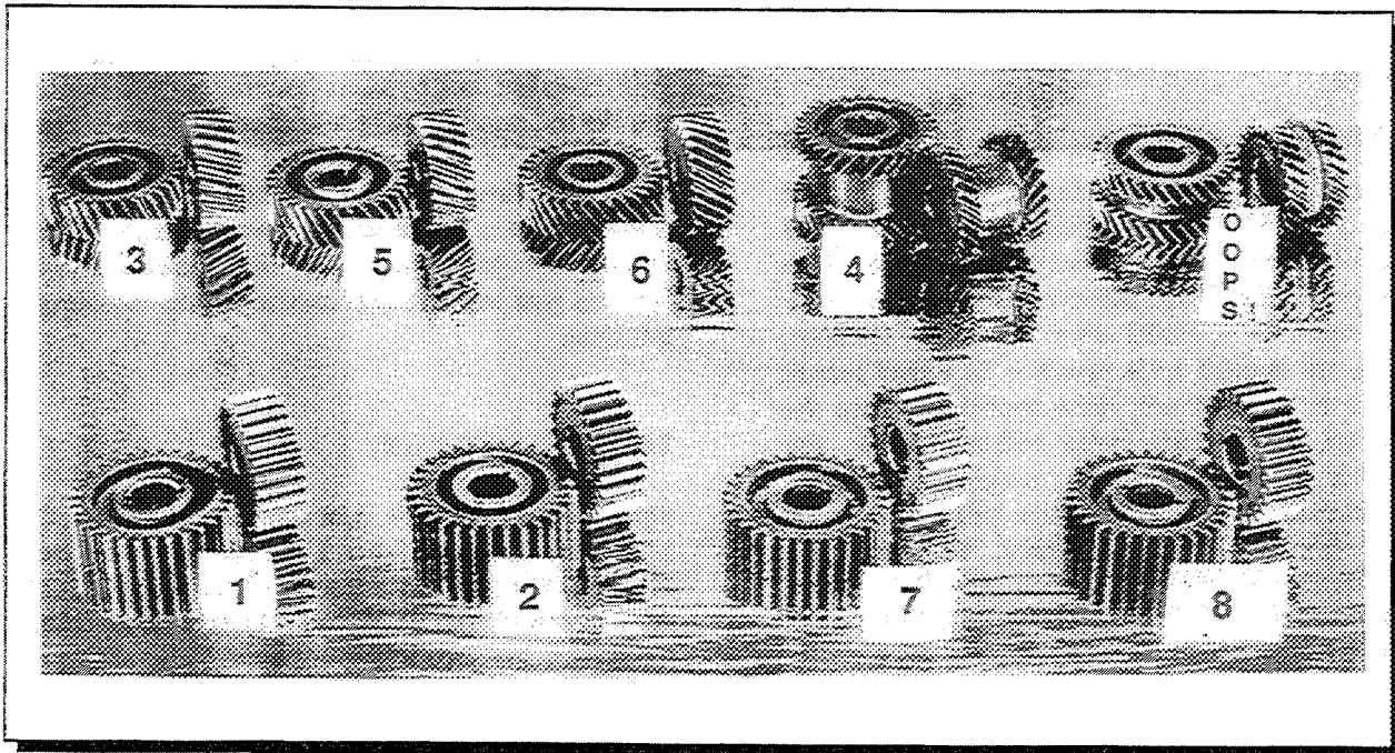
Figure 1 - Test Gears
