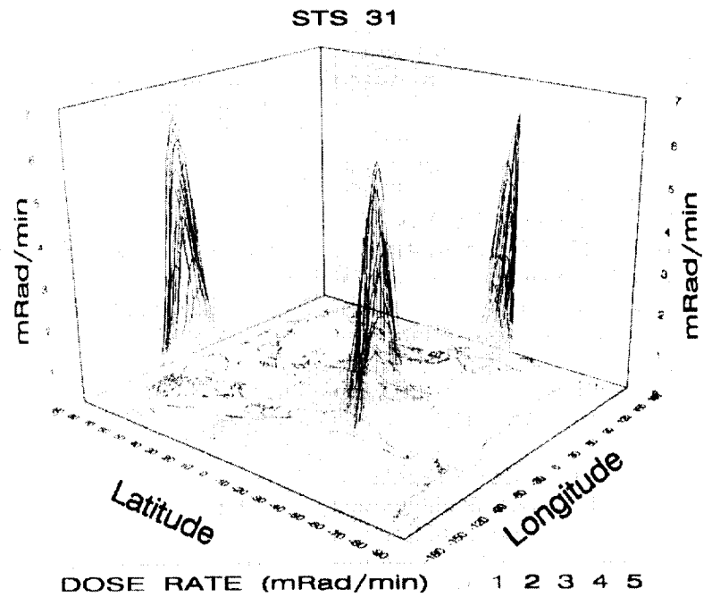
Figure 3. Absorbed dose rate as a function of position for a 28.5-degree inclination Shuttle flight.
