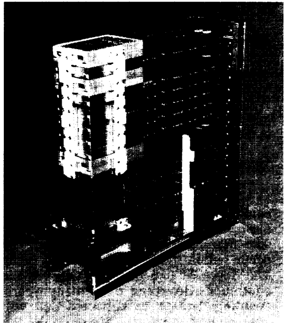
Figure 14. Charged particle directional spectrometer (CPDS).
