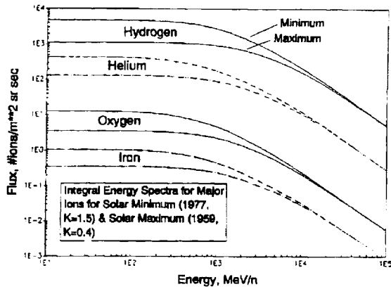
Figure 5. Integral GCR fluence as a function of solar cycle.
