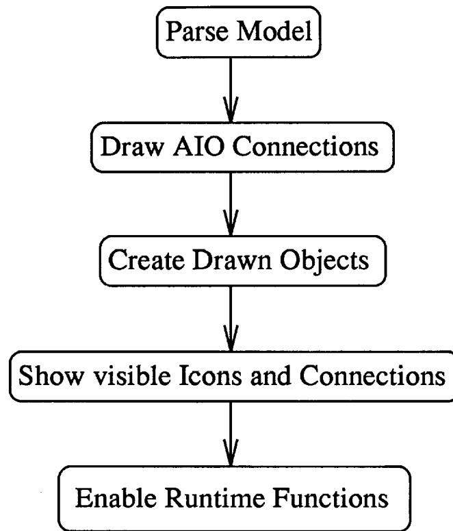
Figure 4: Program Flow for Load Model
