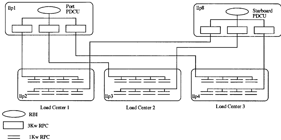
Figure 2: The SSM/PMAD Breadboard Schematic
