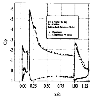
Pressure Coefficient Comparison
