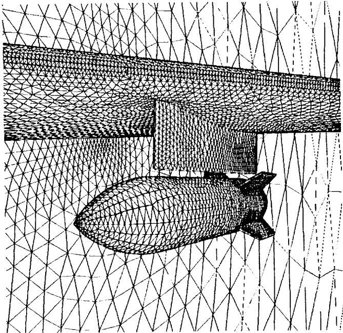
Details of Surface Grid on a Wing/Pylon/Store Configuration
