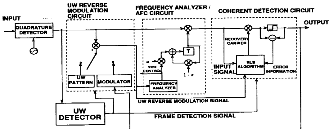
Figure 5 Configuration of UW-Reverse-Modulation Type Demodulator
