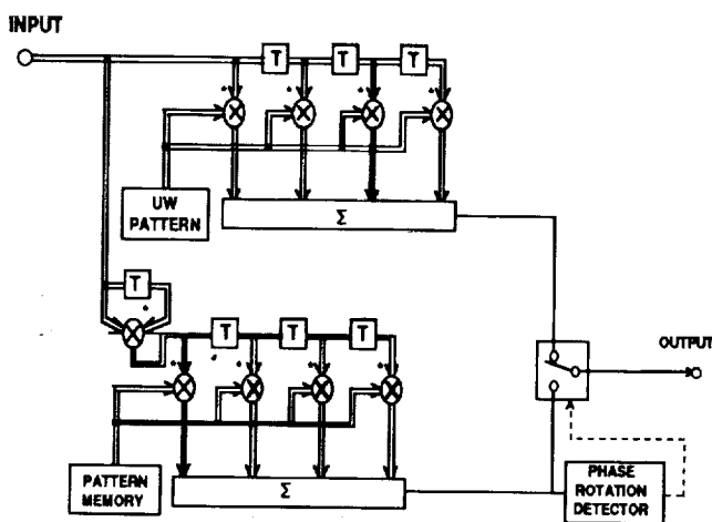
Figure 4 Configuration of UW Detector
