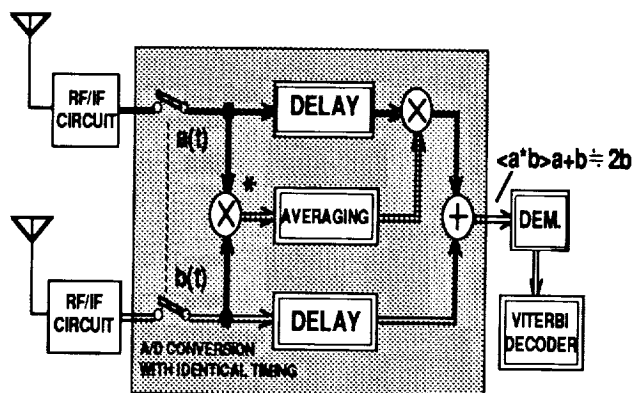
Figure 2 Configuration of Pre-detection Signal Combiner
