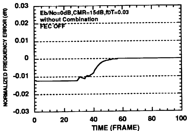
Figure 6 Pull-in Performance
