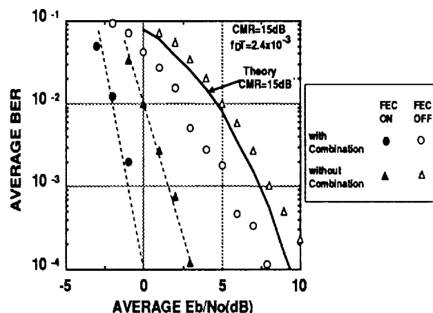
Figure 8 Average BER Performances
